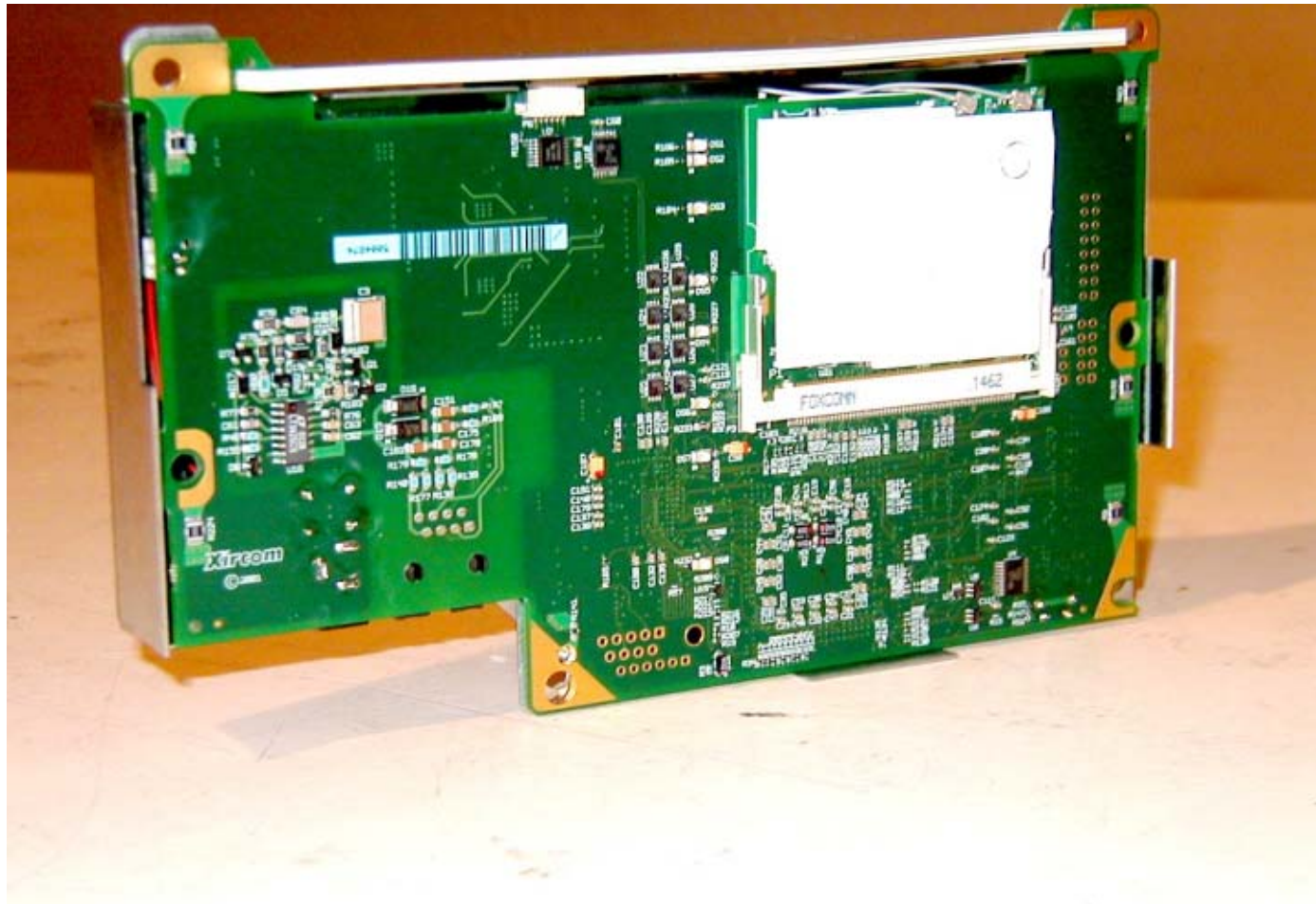
Half shield removed, exposing the Front Side of AP Motherboard (LED Side)
