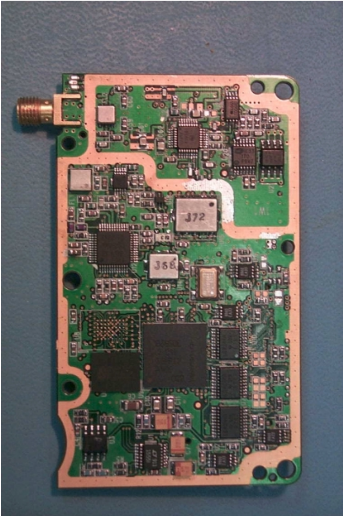
Photo 1. Top of Eagle II PCB (shields removed).
