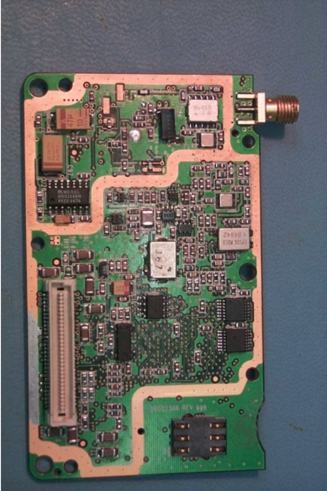
Photo 2. Bottom of Eagle II PCB (shields removed).
