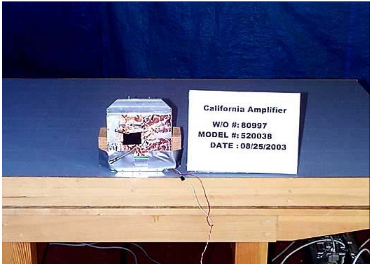
Radiated Emissions - Minimum Power Front View
