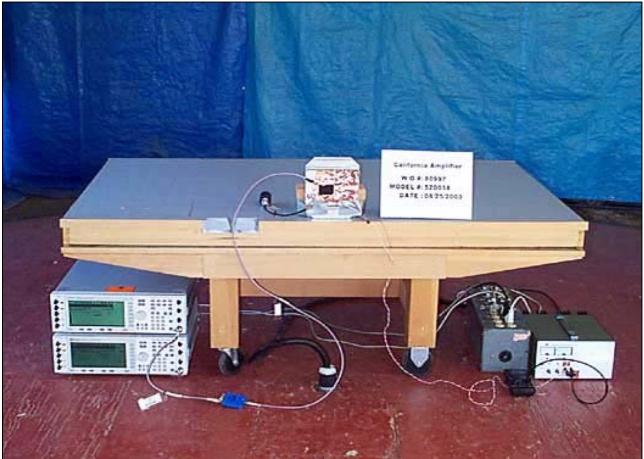
Radiated Emissions - Maximum Power Front View
