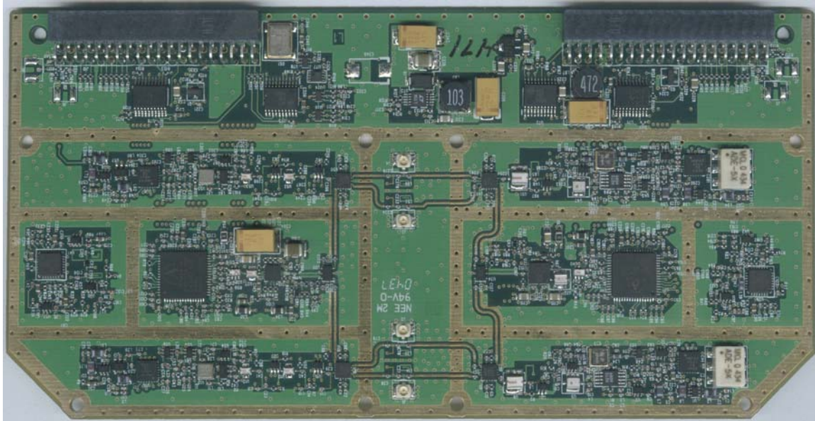
132621 board top
