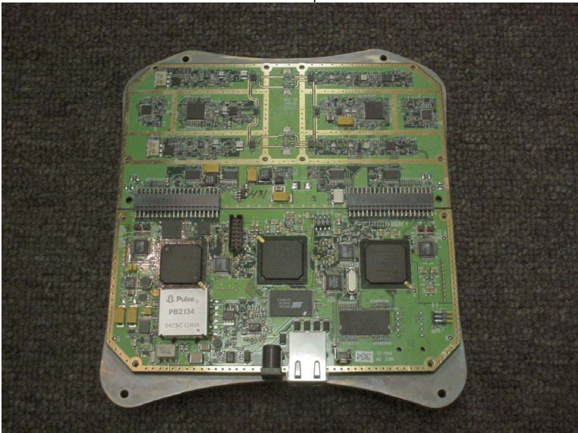
No shield – top rear
