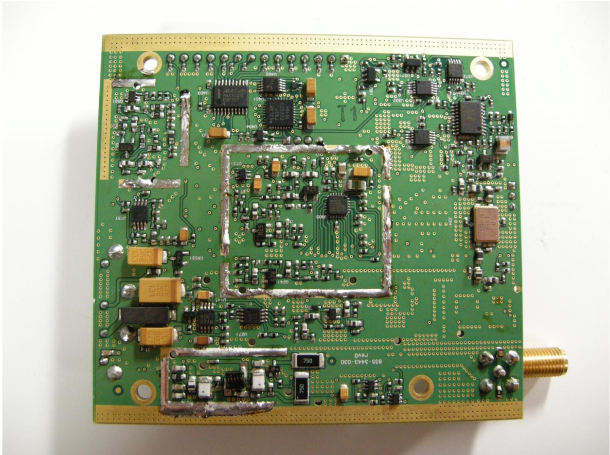
TX PCB Shield Removed Bottom
