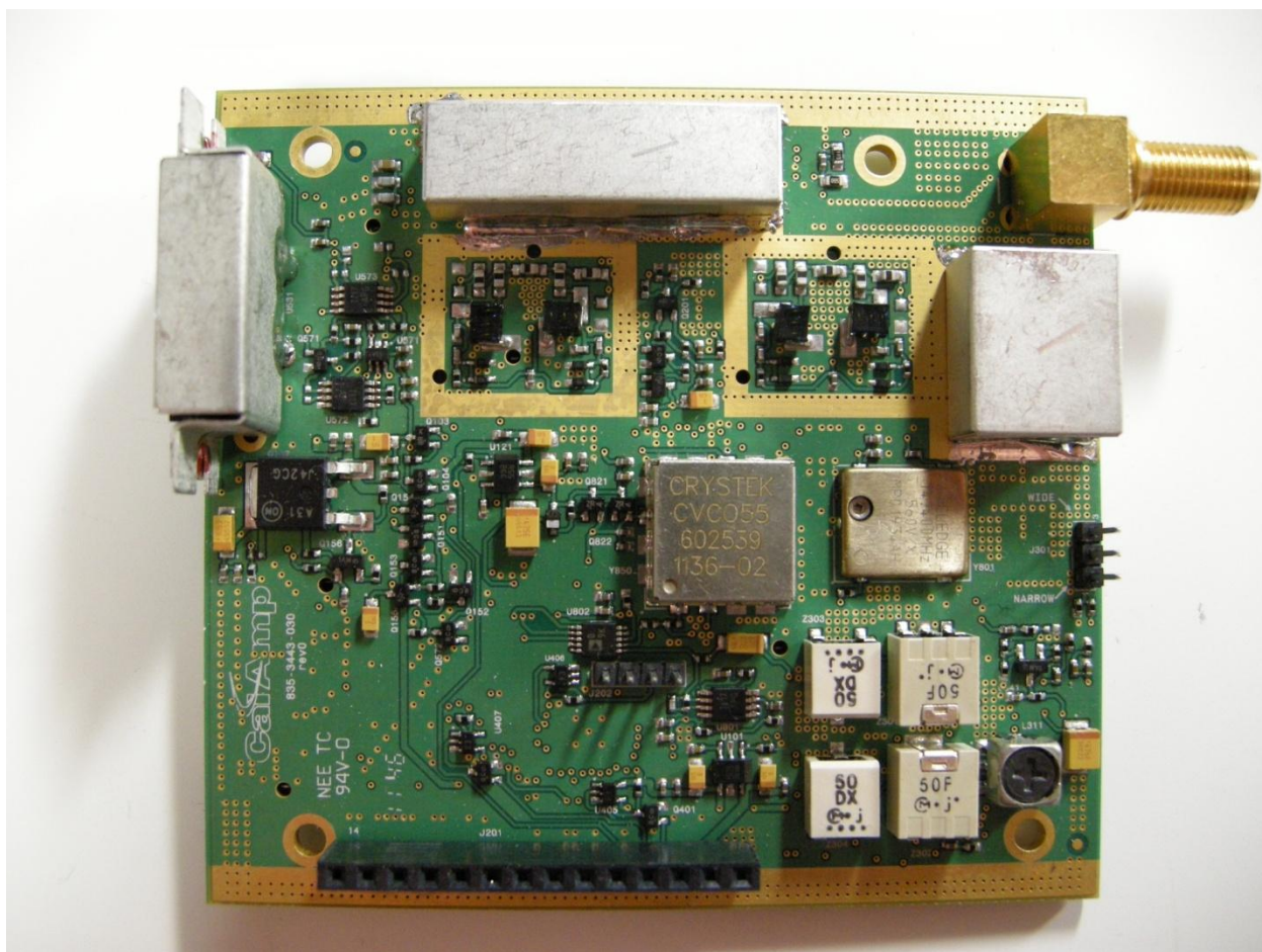
TX Module Exposed Top
