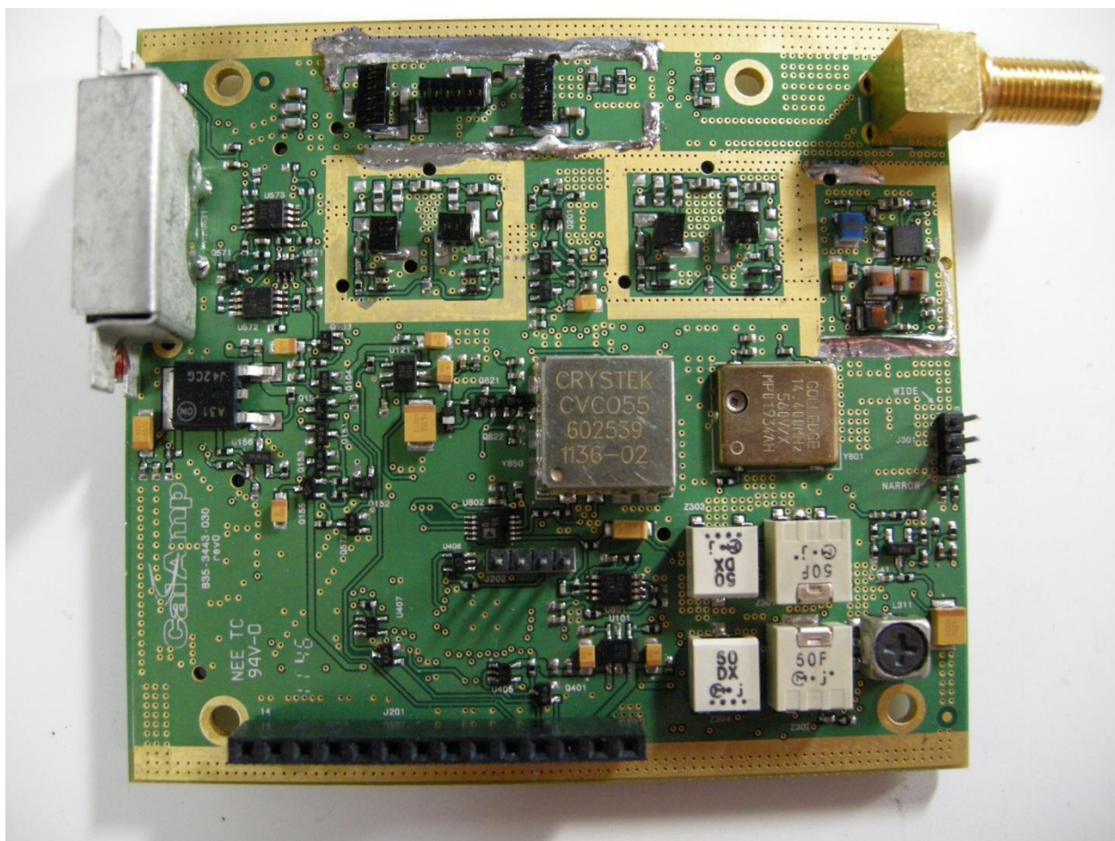
TX PCB Shield Removed Top
