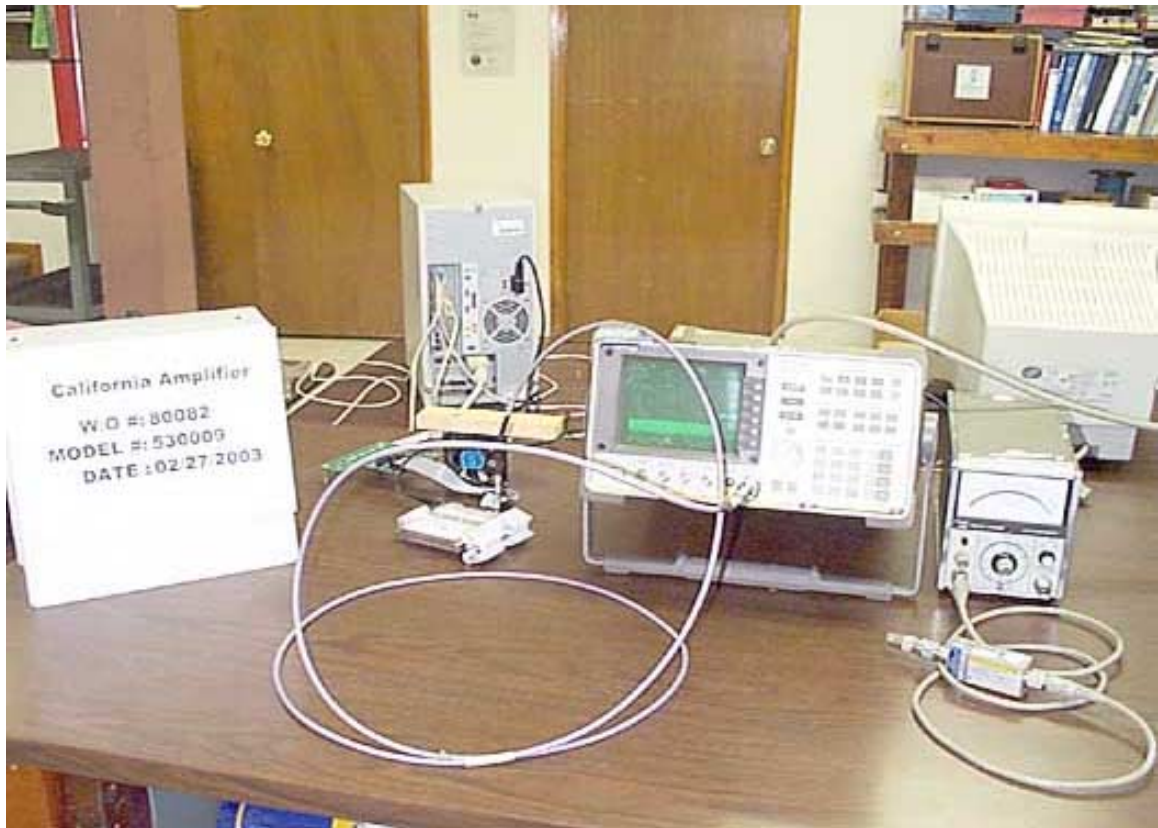
Test Setup Photo for 2.1049 & 2.1051
