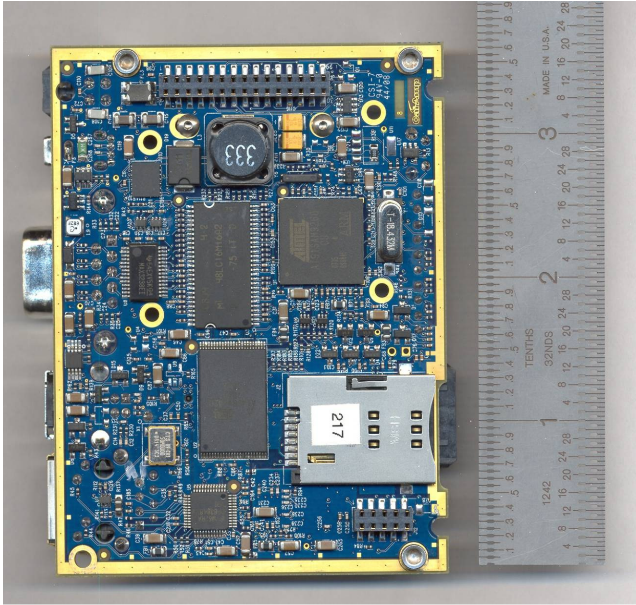
WiMetry Core Module Bottom Side
