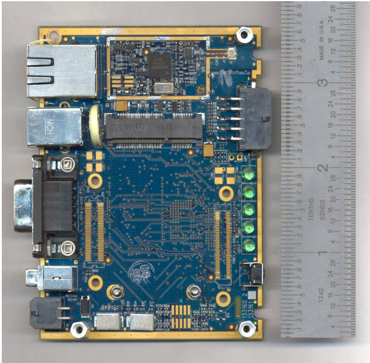
WiMetry Core Module Top Side with 802.15 Shield Removed
