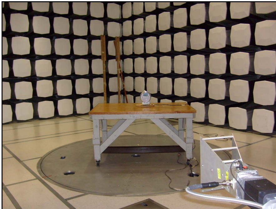
Photograph 4. Radiated Emissions, Test Setup, Horn
