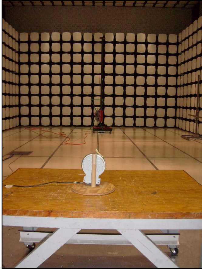
Photograph 3. Radiated Emissions, Test Setup, Back View
