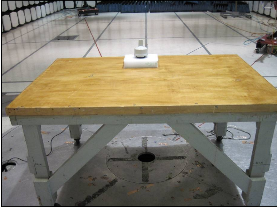
Photograph 5. Radiated Emission, Test Setup, Rear Review
