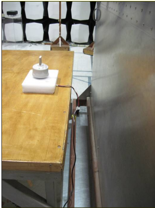
Photograph 2. Conducted Emissions, Test Setup, Side View
