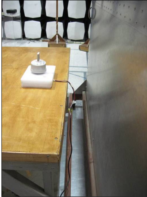
Photograph 7. Conducted Emissions, 15.207, Test Setup, Side View
