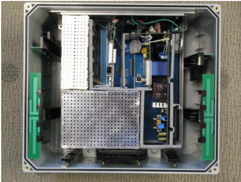
Internal View-2
