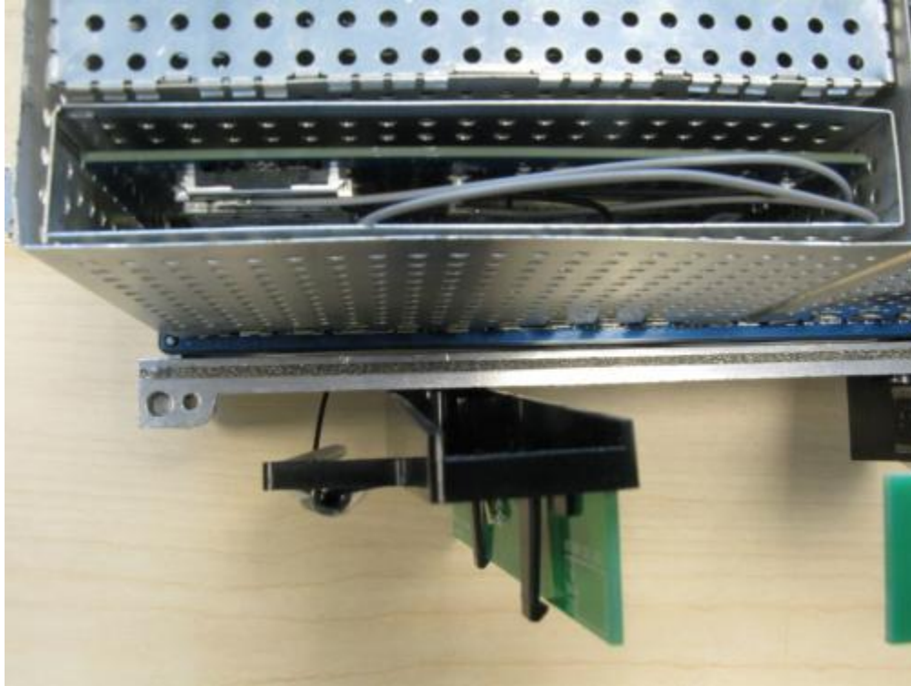
Internal View-4: Antenna Connection
