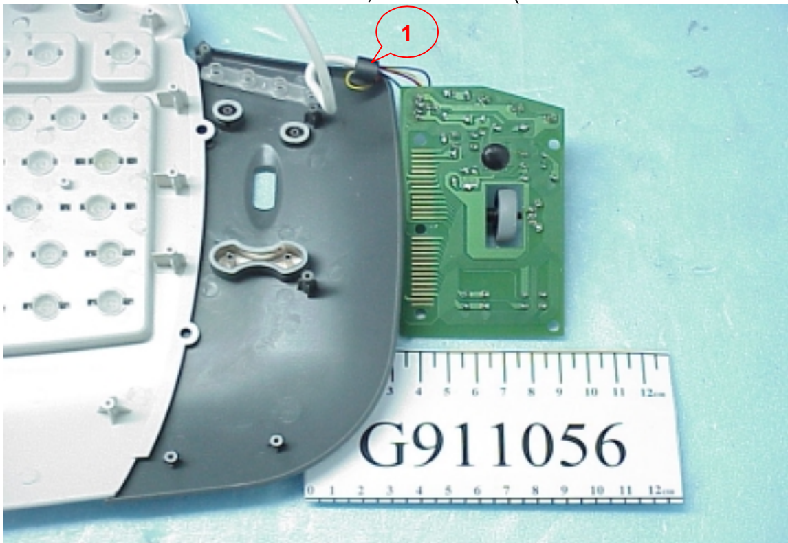
Figure 4 M/N OFFICE 800, Internal View (Removed LED / Control Board)
