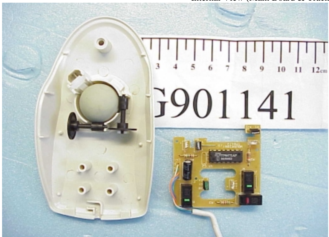
Figure 4 Internal View (Main Board & Trackball)
