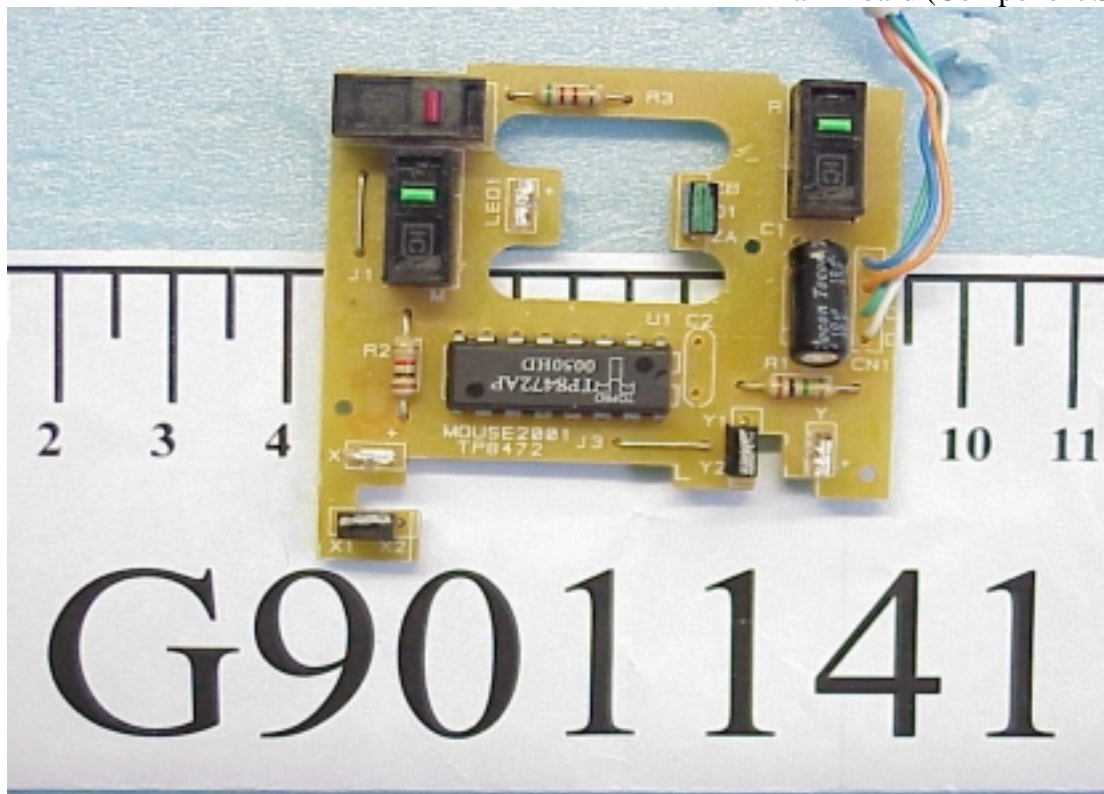
Figure 5 Main Board (Component Side)
