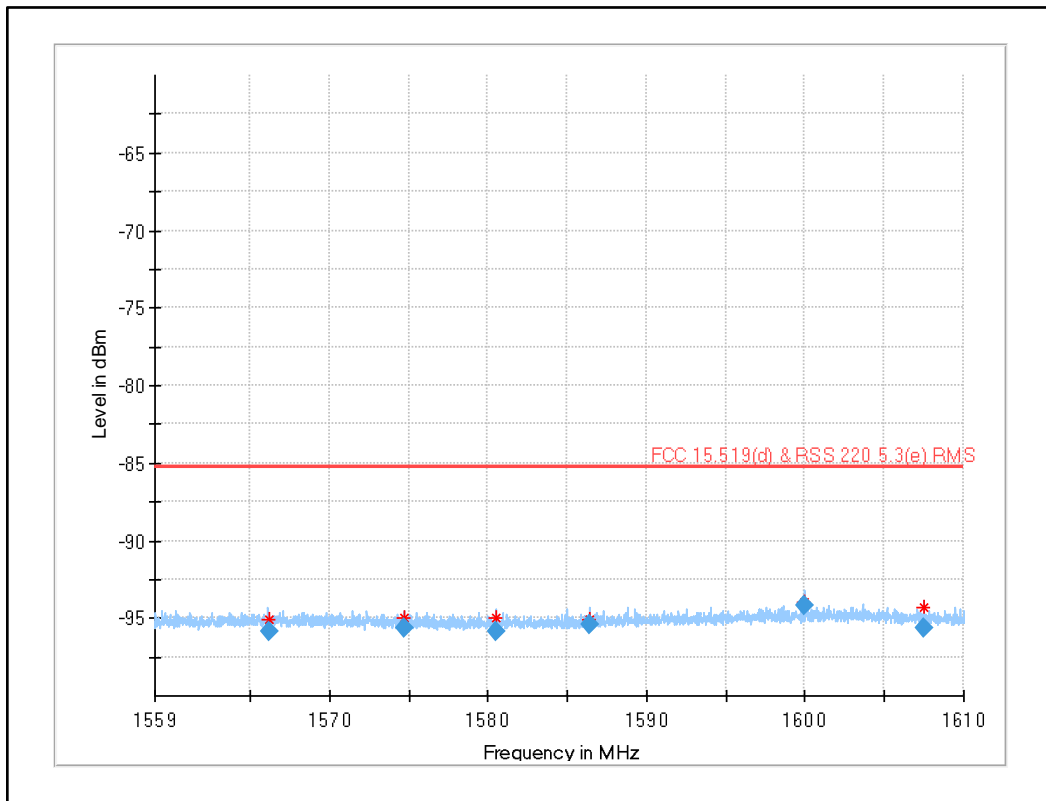
Plot 26: 1559 MHz to 1610 MHz UWB test mode channel 6
