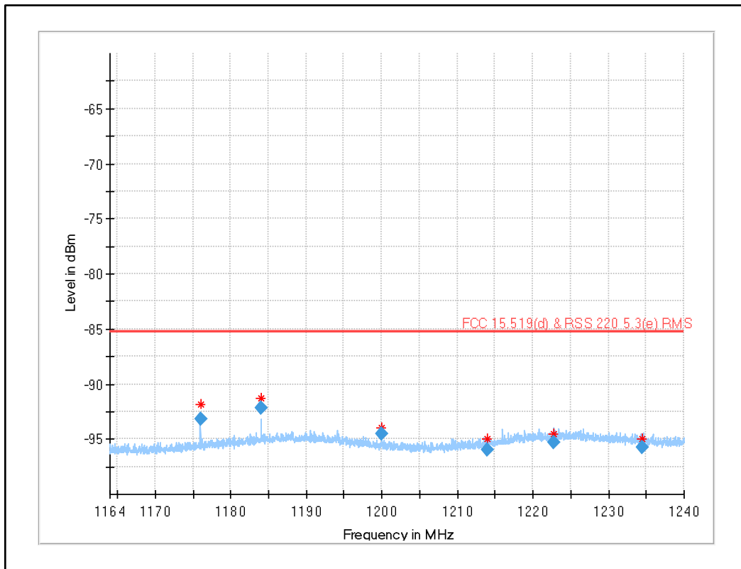
Plot 14: 1164 MHz to 1240 MHz UWB test mode channel 5
