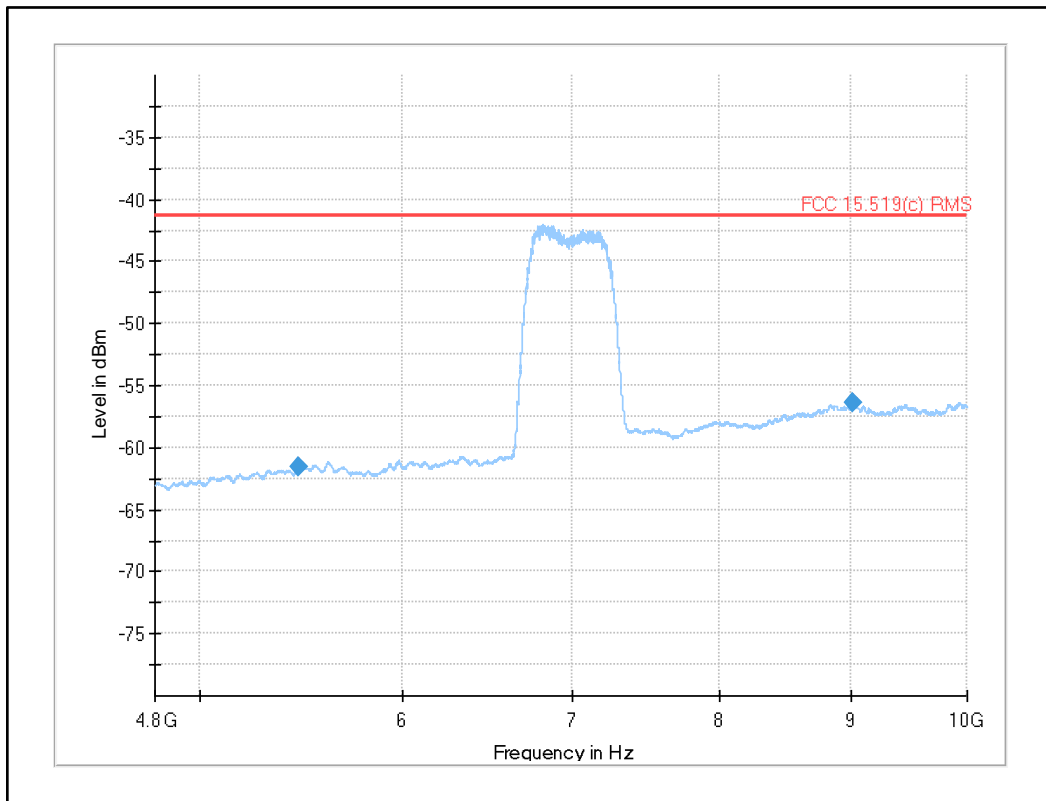
Plot 21: 4.8 GHz to 10 GHz, UWB test mode channel 6
