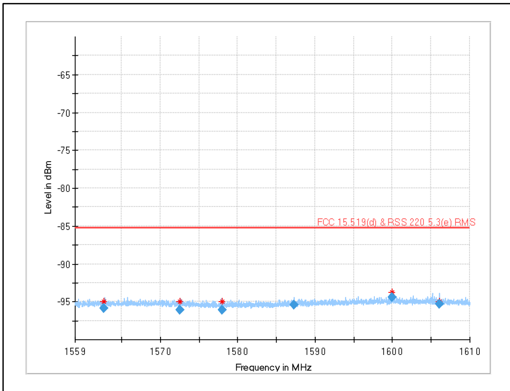
Plot 15: 1559 MHz to 1610 MHz UWB test mode channel 5
