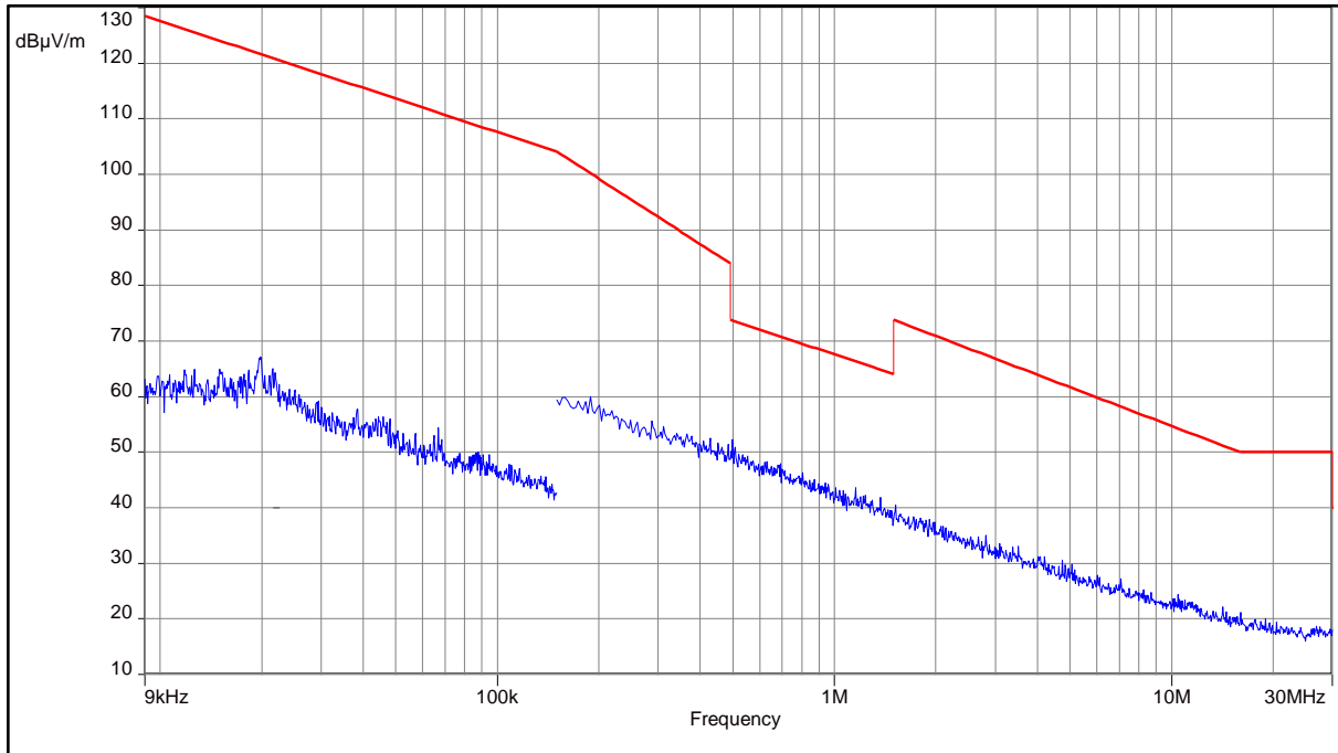
Plot 18: 9 kHz to 30 MHz, UWB test mode channel 6
