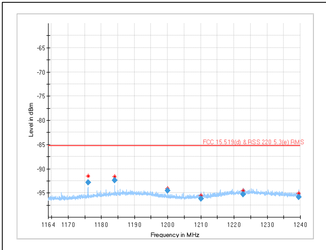
Plot 25: 1164 MHz to 1240 MHz UWB test mode channel 6
