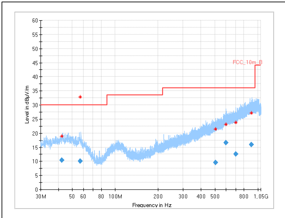
Plot 8: 30 MHz to 1 GHz, UWB test mode channel 5
