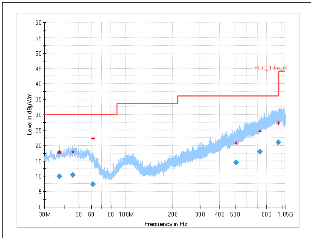
Plot 42: 30 MHz to 1 GHz, UWB test mode channel 9
