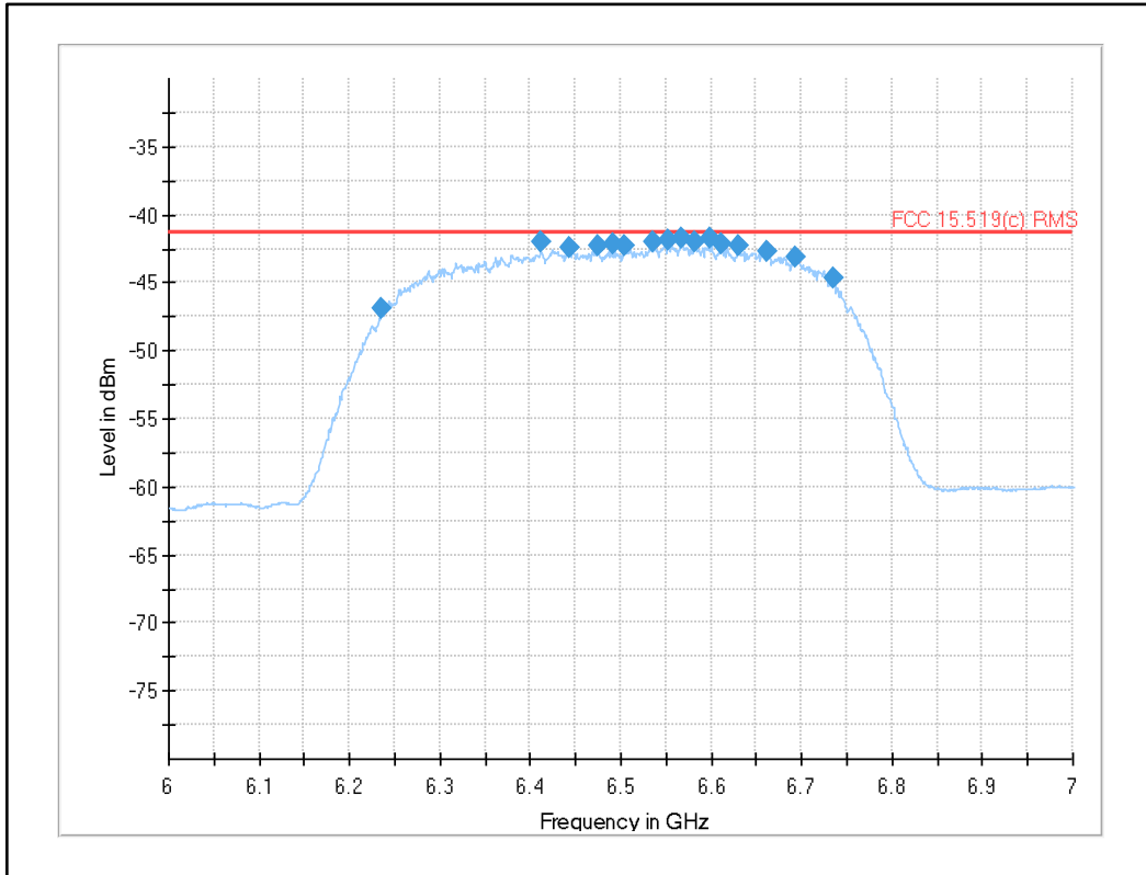
Plot 5: Fundamental emission (UWB test mode): RMS channel 5
