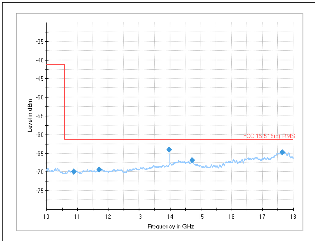
Plot 22: 10 GHz to 18 GHz, UWB test mode channel 6
