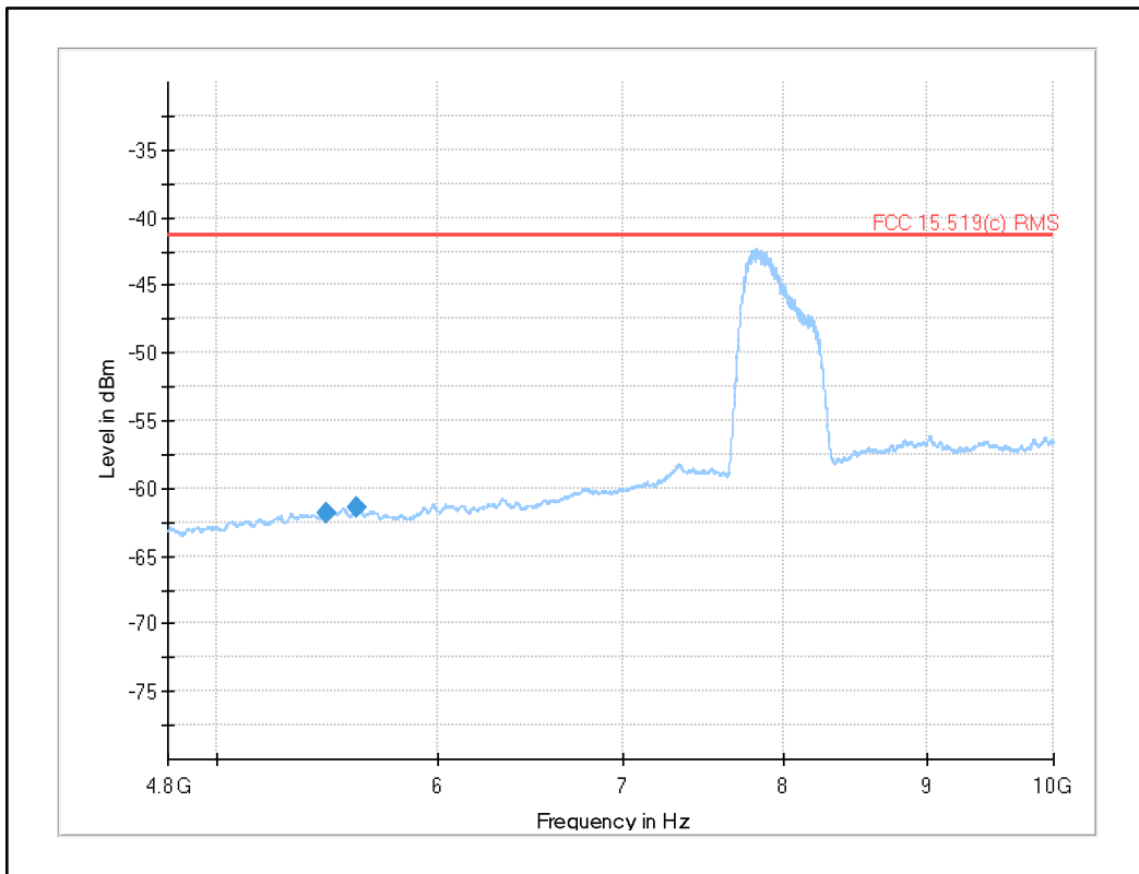
Plot 44: 4.8 GHz to 10 GHz, UWB test mode channel 9
