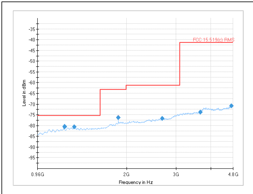
Plot 20: 960 MHz to 4.8 GHz, UWB test mode channel 6
