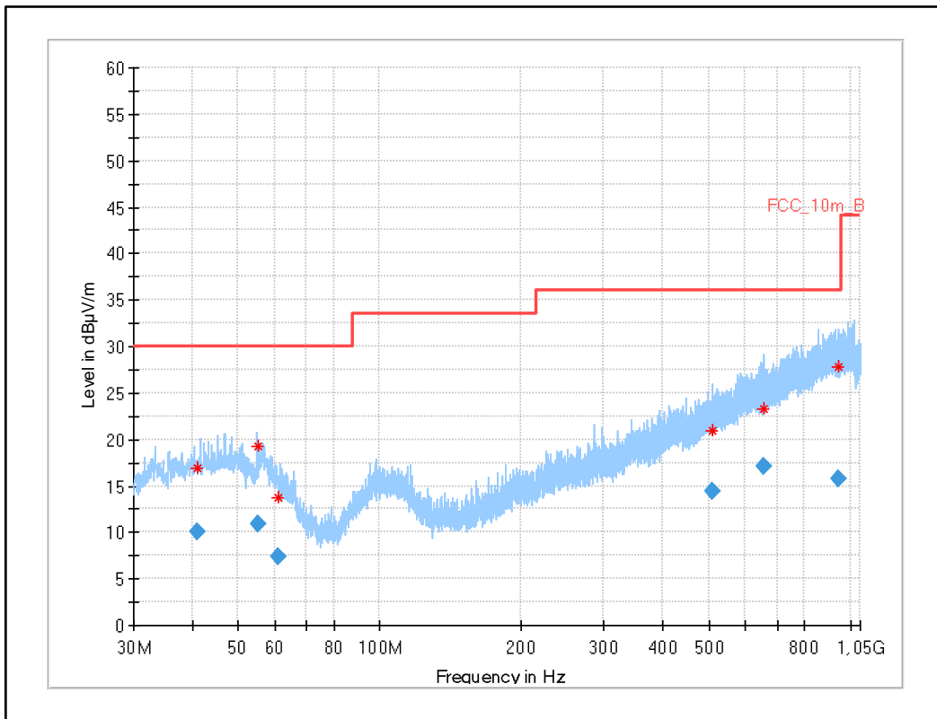
Plot 19: 30 MHz to 1 GHz, UWB test mode channel 6
