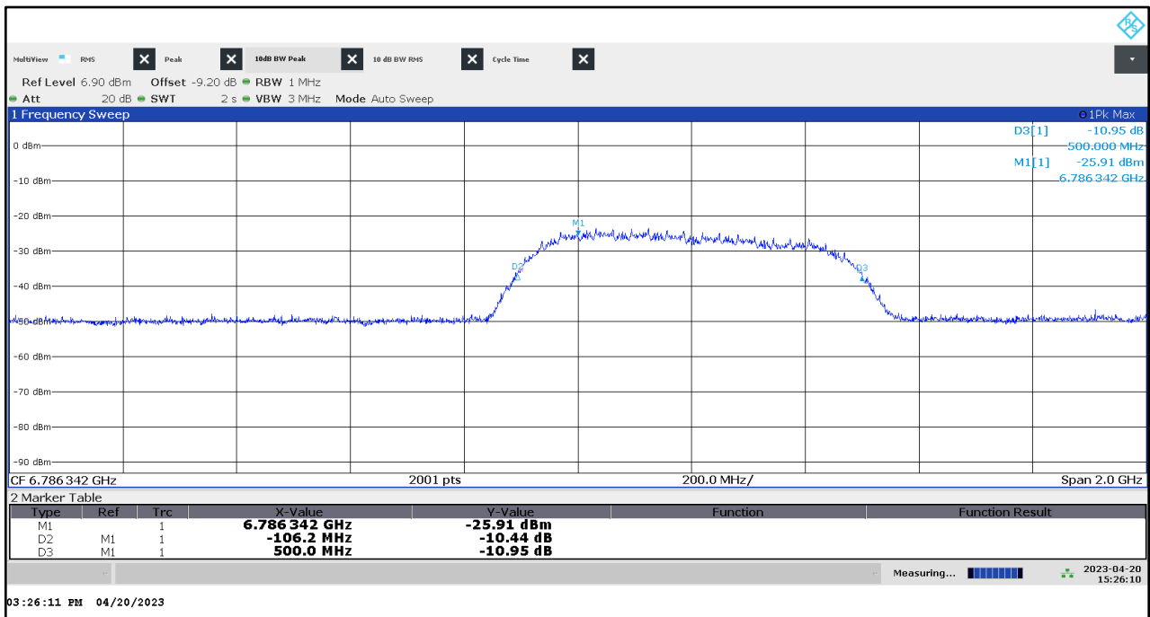
Plot 2: 10 dB bandwidth, EUT 2 UWB test mode on channel 6
