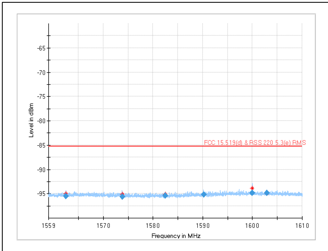
Plot 38: 1559 MHz to 1610 MHz UWB test mode channel 6
