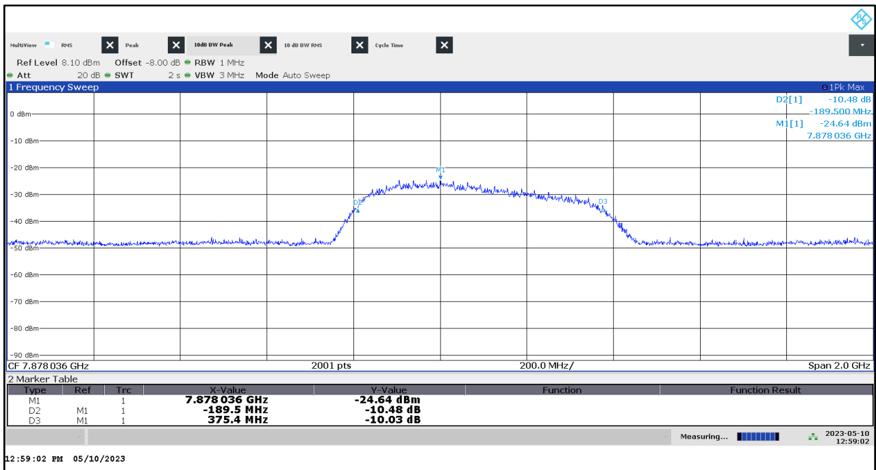
Plot 4: 10 dB bandwidth, EUT 4 UWB test mode on channel 9
