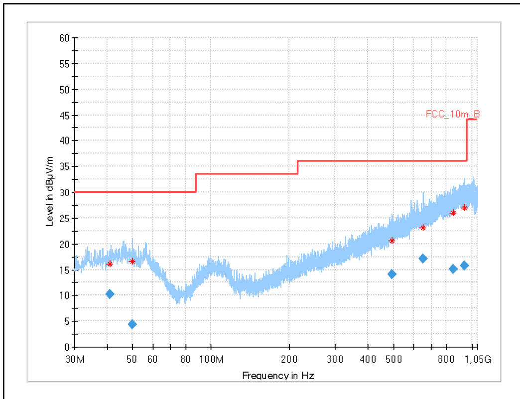
Plot 30: 30 MHz to 1 GHz, UWB test mode channel 8
