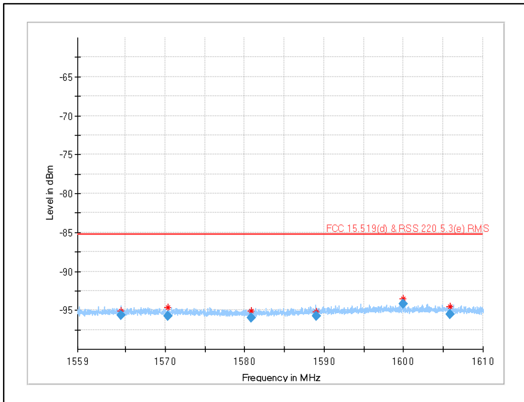
Plot 50: 1559 MHz to 1610 MHz (§15.519 (d)), UWB test mode channel 9
