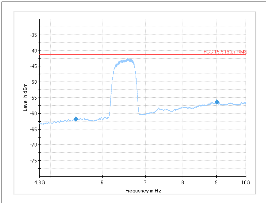
Plot 10: 4.8 GHz to 10 GHz, UWB test mode channel 5
