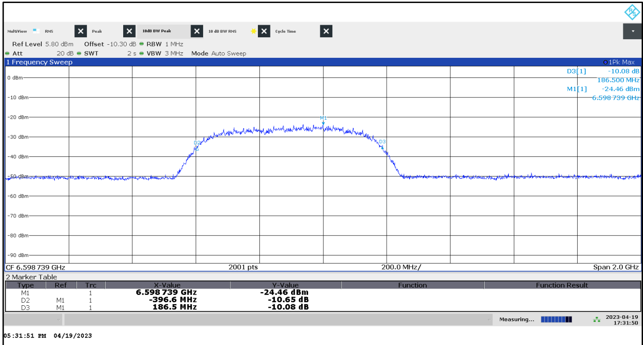
Plot 1: 10 dB bandwidth, EUT 1 UWB test mode on channel 5
