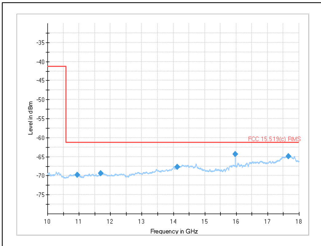
Plot 45: 10 GHz to 18 GHz, UWB test mode channel 9
