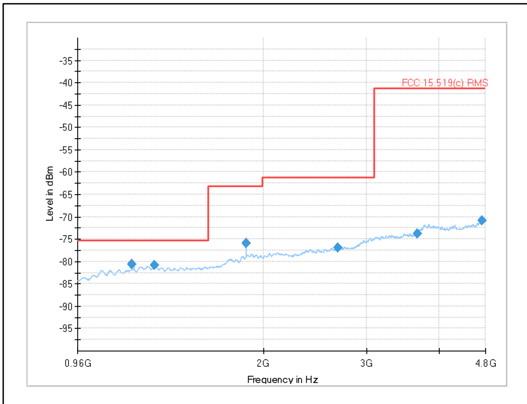
Plot 31: 960 MHz to 4.8 GHz, UWB test mode channel 8
