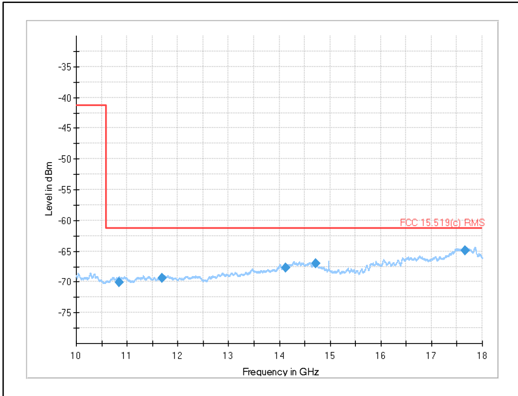
Plot 33: 10 GHz to 18 GHz, UWB test mode channel 8
