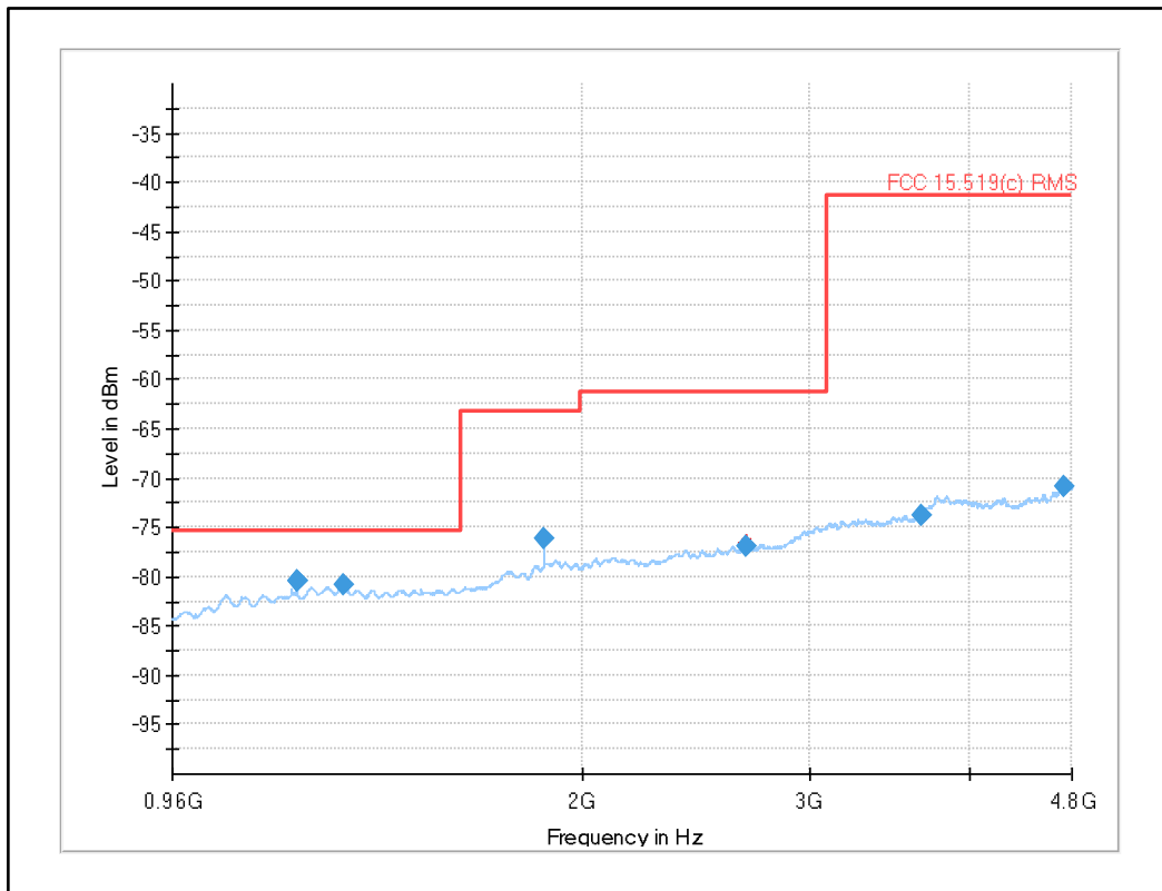
Plot 9: 960 MHz to 4.8 GHz, UWB test mode channel 5
