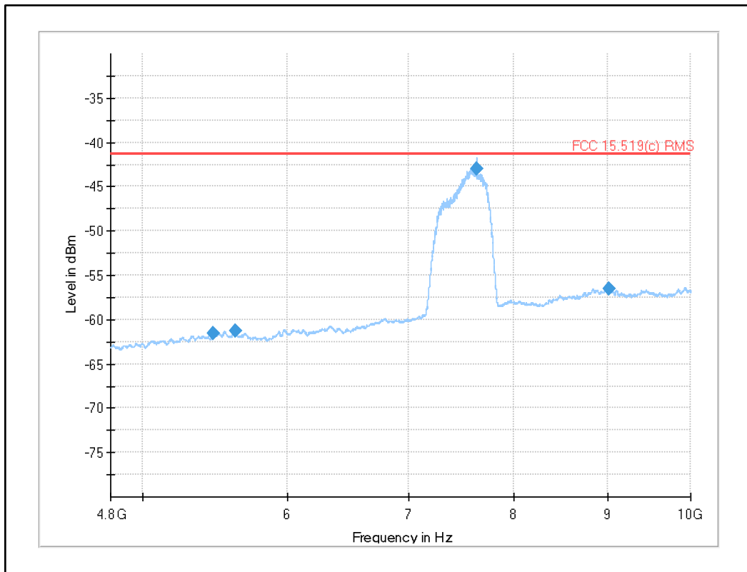
Plot 32: 4.8 GHz to 10 GHz, UWB test mode channel 8
