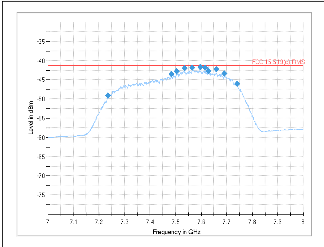
Plot 27: Fundamental emission (UWB test mode): RMS channel 8
