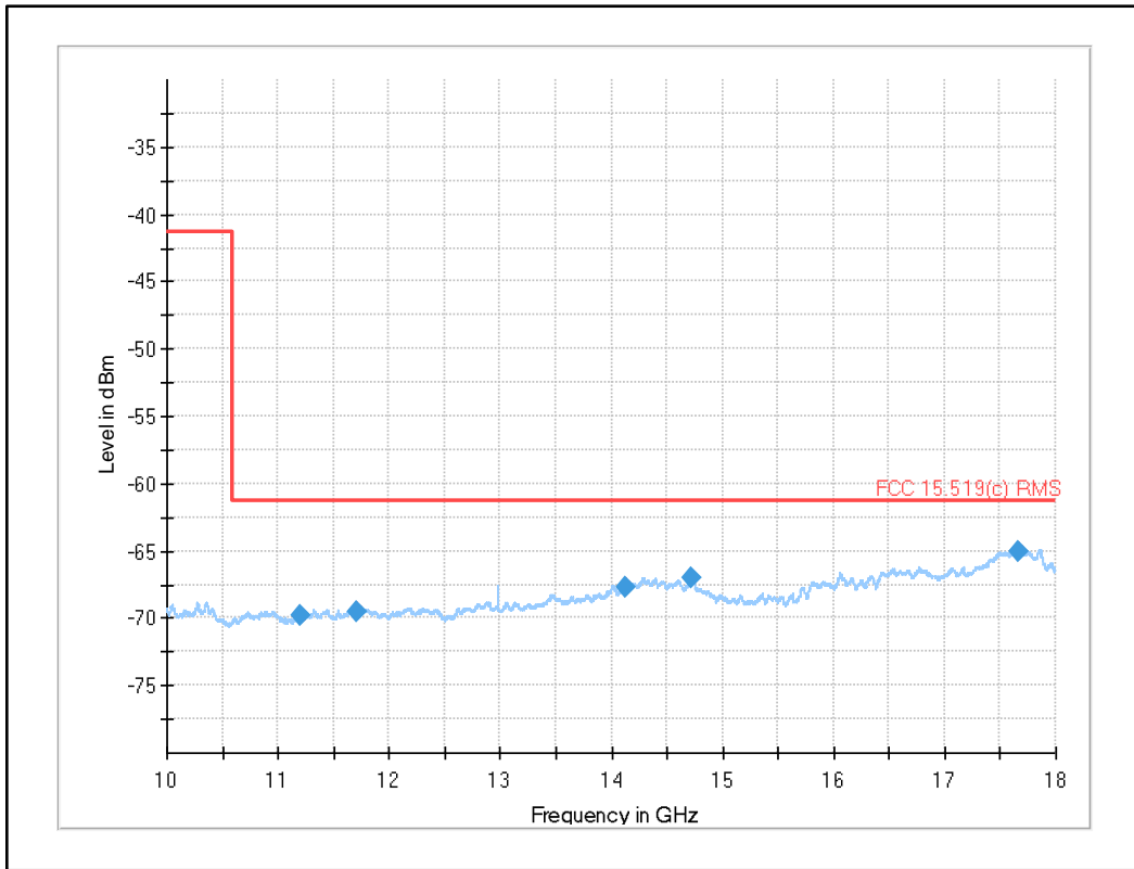
Plot 11: 10 GHz to 18 GHz, UWB test mode channel 5
