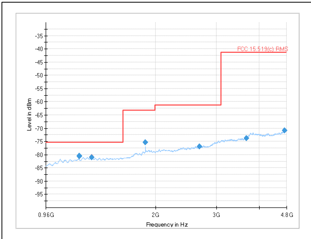
Plot 43: 960 MHz to 4.8 GHz (Limit acc. to §15.519 (c)), UWB test mode channel 9
