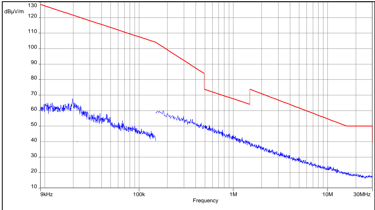
Plot 29: 9 kHz to 30 MHz, UWB test mode channel 8
