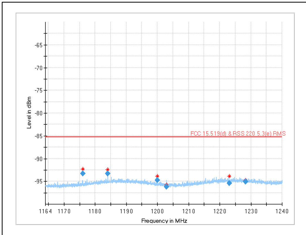
Plot 49: 1164 MHz to 1240 MHz (§15.519 (d)), UWB test mode channel 9
