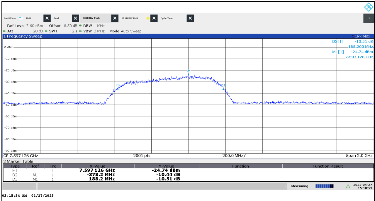
Plot 3: 10 dB bandwidth, EUT 3 UWB test mode on channel 8
