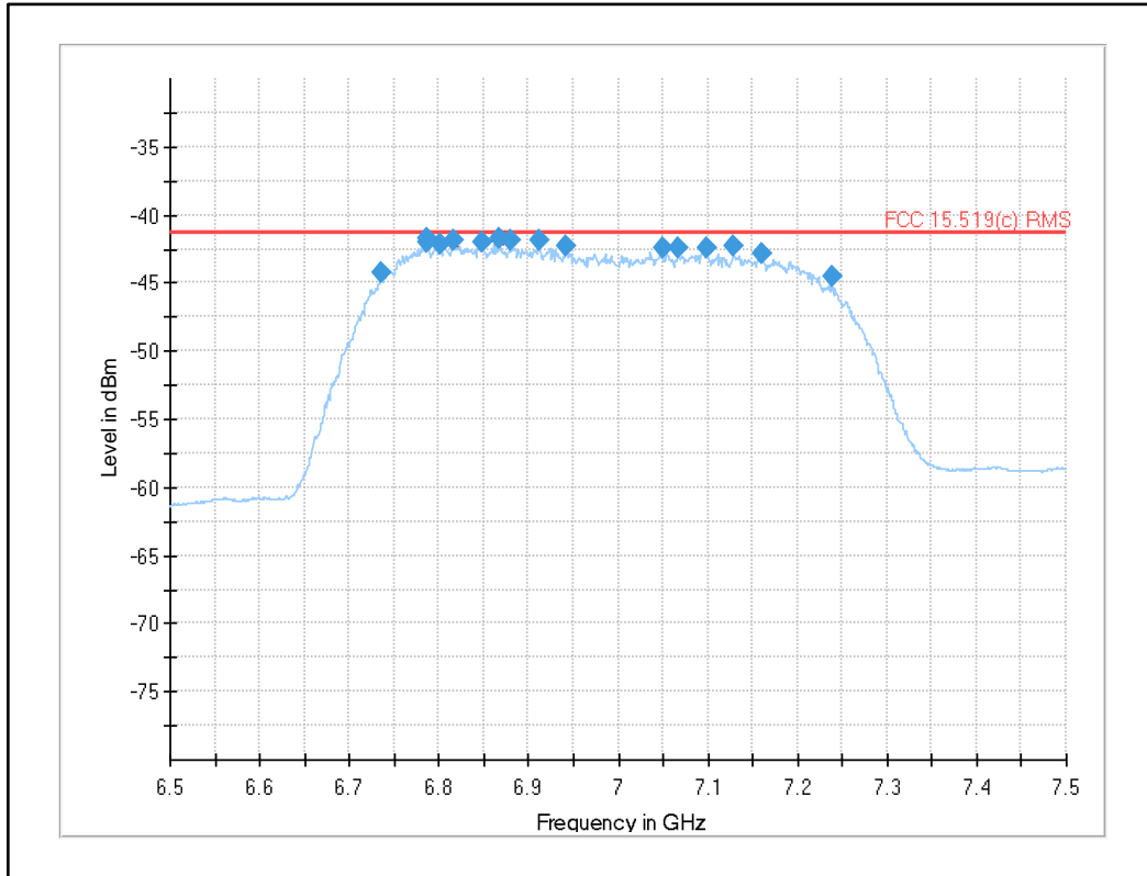
Plot 16: Fundamental emission (UWB test mode): RMS channel 6
