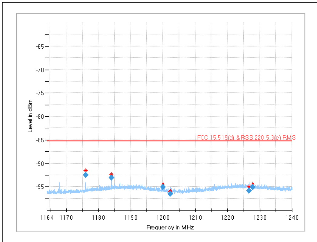
Plot 37: 1164 MHz to 1240 MHz UWB test mode channel 8
