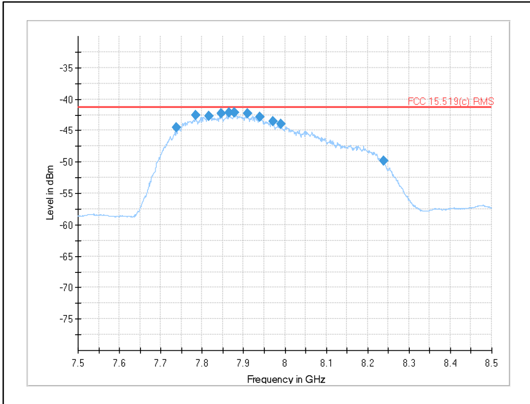
Plot 39: Fundamental emission (UWB test mode): RMS channel 9
