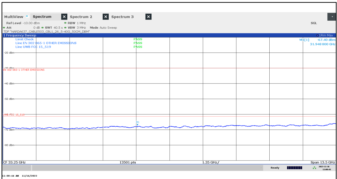
Plot 52: 26.5 GHz to 40.0 GHz, UWB test mode
