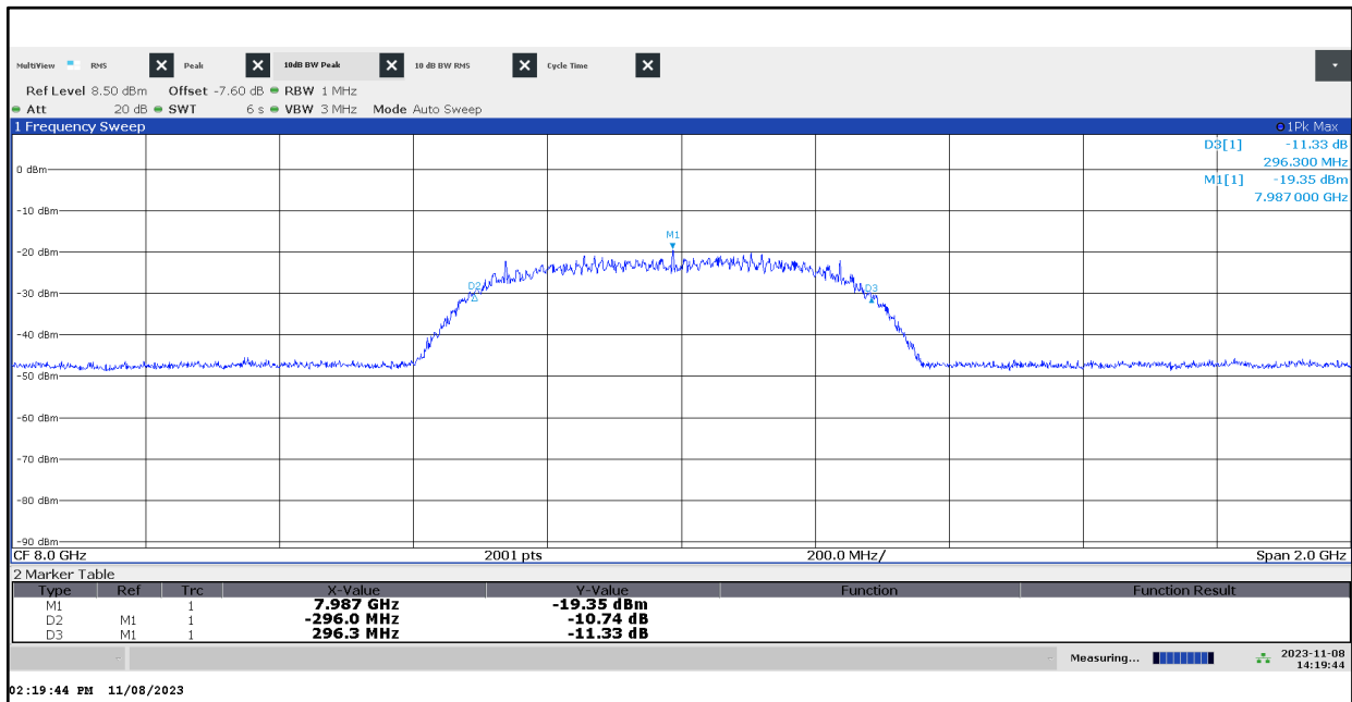
Plot 4: 10 dB bandwidth, UWB test mode channel 9
