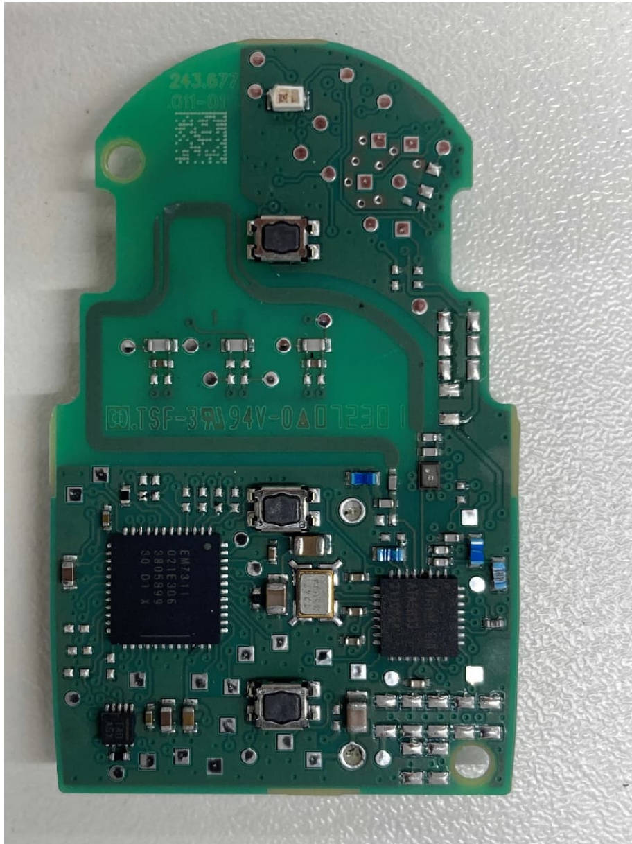
MS6, PCB, top view Photo supplied by the applicant
