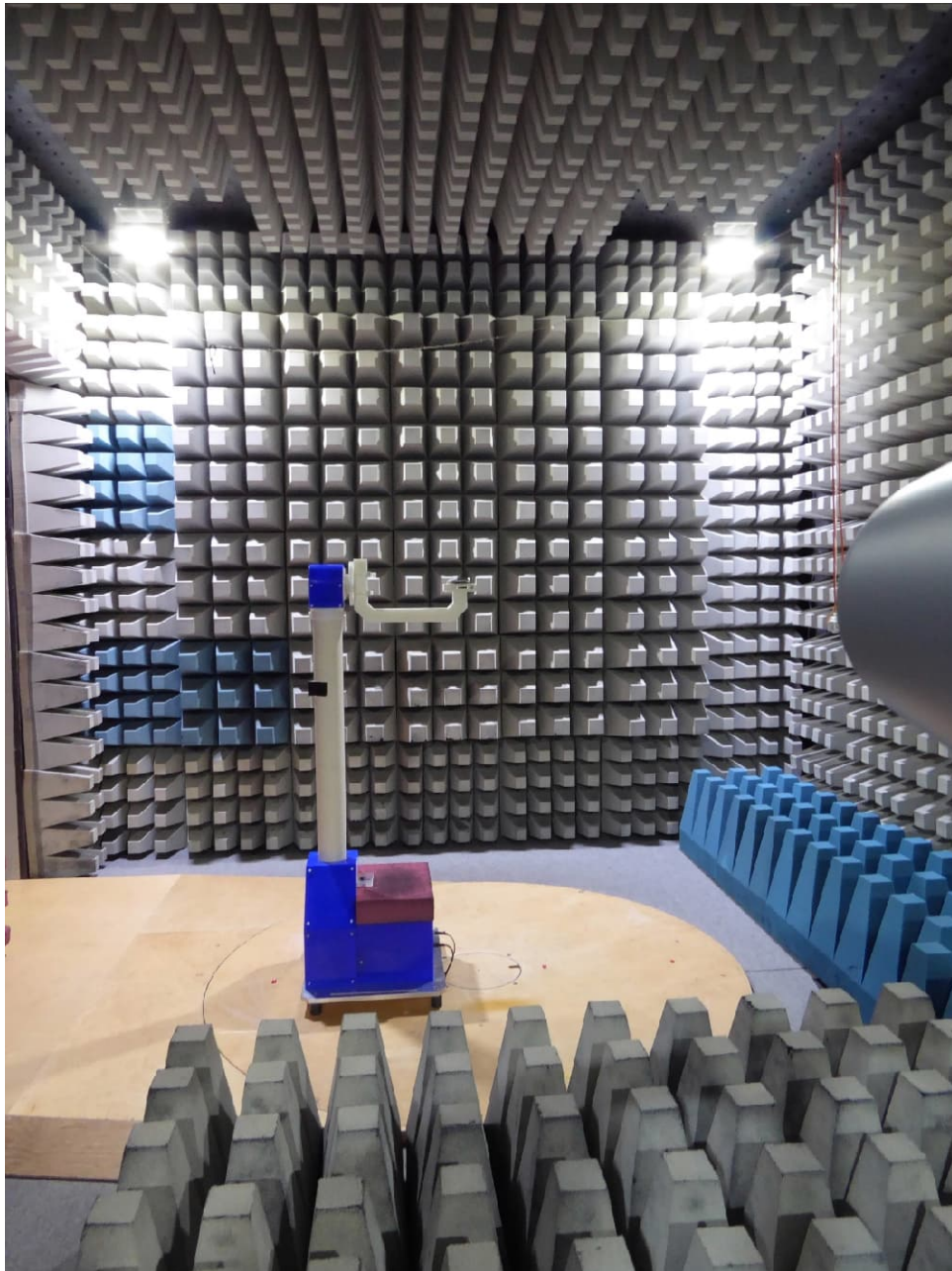
Test setup fully anechoic chamber (1 GHz to 2 GHz)
