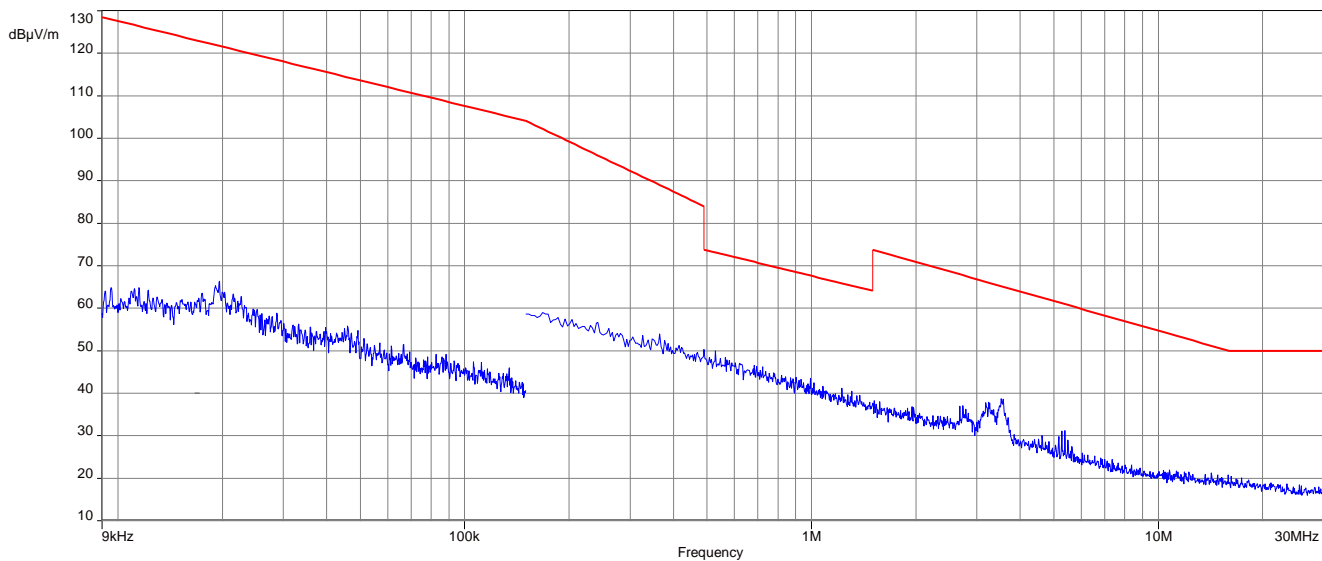
Plot 8: Channel B, 9 kHz to 30 MHz
