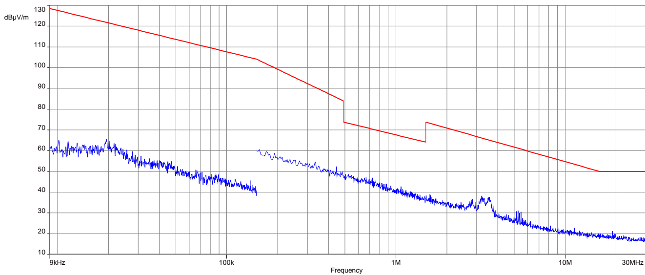
Plot 9: Channel C, 9 kHz to 30 MHz
