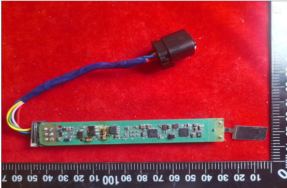
Figure 1. Top View
