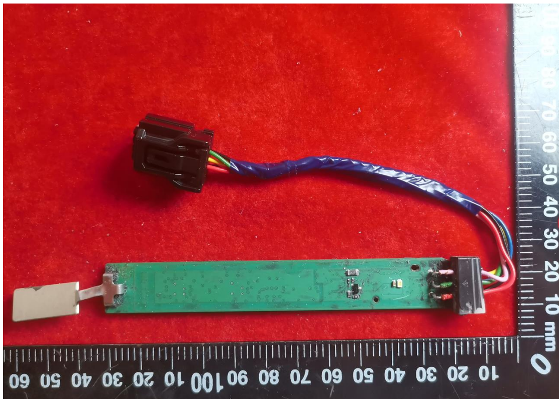
Figure 2. Bottom View
