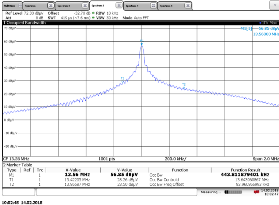
Plot 1: 99 % emission bandwidth, NFC only
