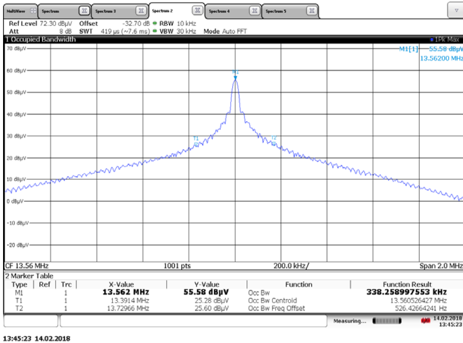
Plot 2: 99 % emission bandwidth, NFC+WPC
