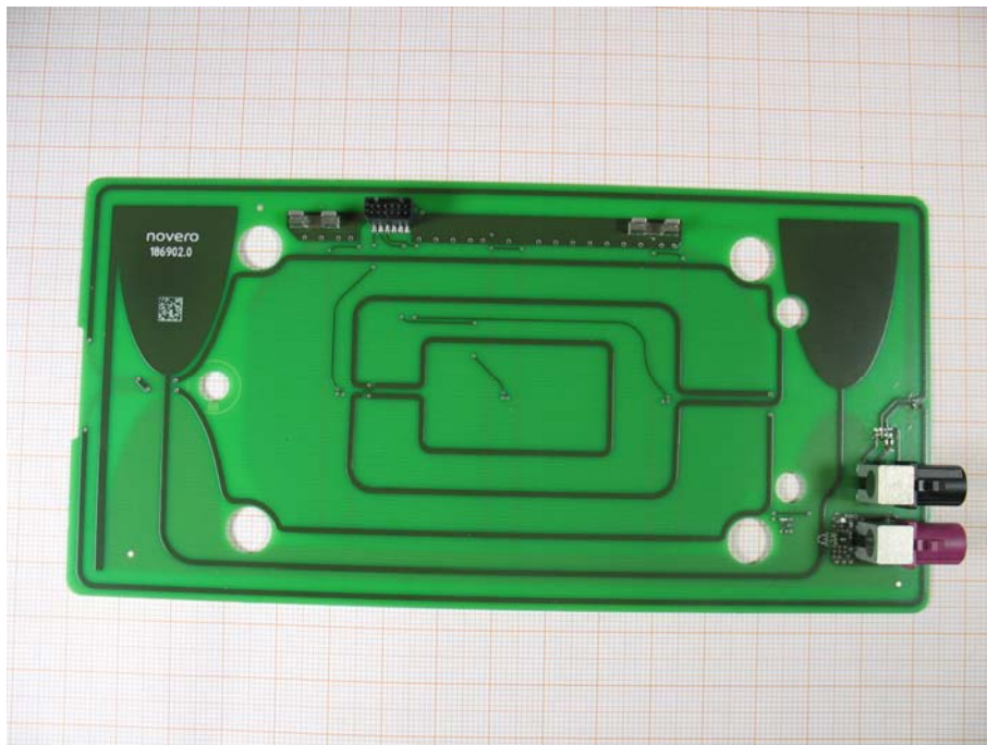
Photo 8: NFC+WPC antenna
