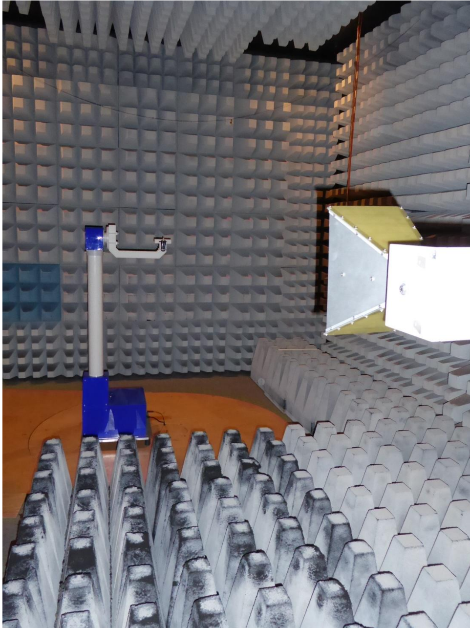
153783_5.JPG: Test setup fully anechoic chamber
