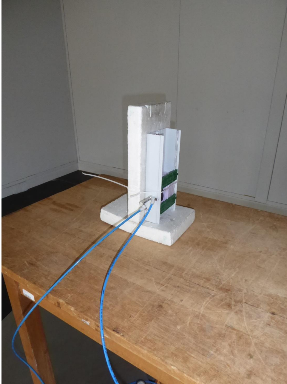
153783_6.JPG: Test setup open area test site
