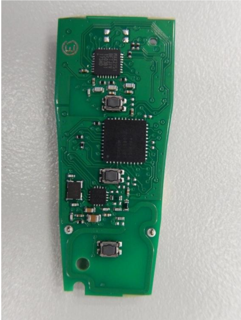
153783_14.JPG: PK1, PCB, top view
