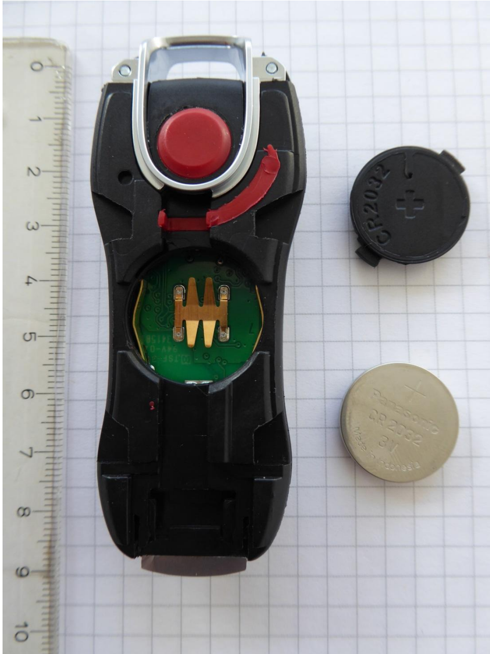
153783_11.JPG: PK1, top view (side covers, battery cover and battery removed)
