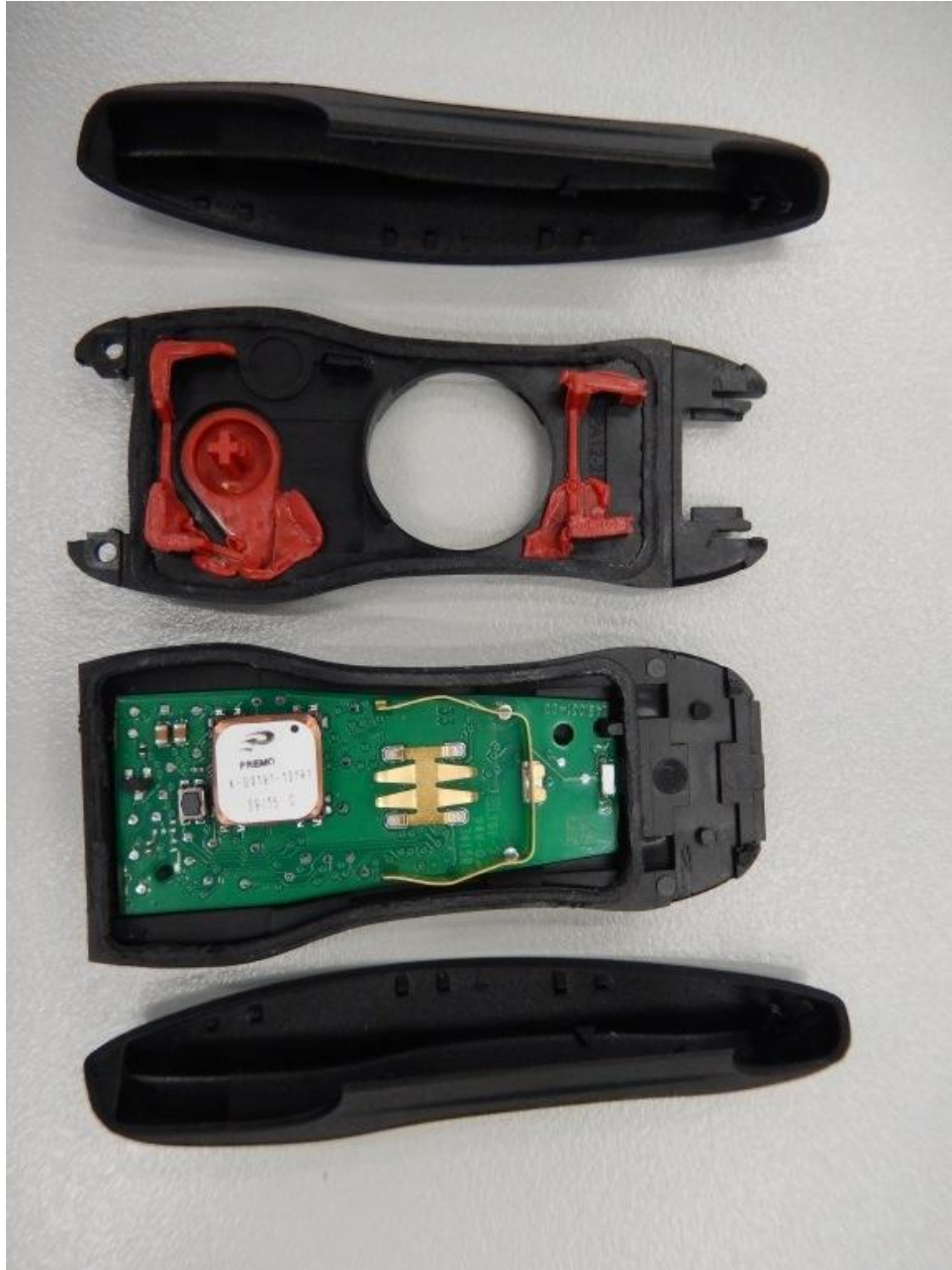
153783_12.JPG: PK1, bottom view (side covers and rear cover removed)
