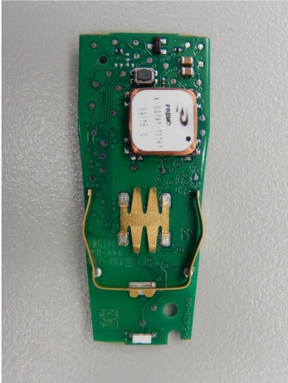
153783_13.JPG: PK1, PCB, bottom view
