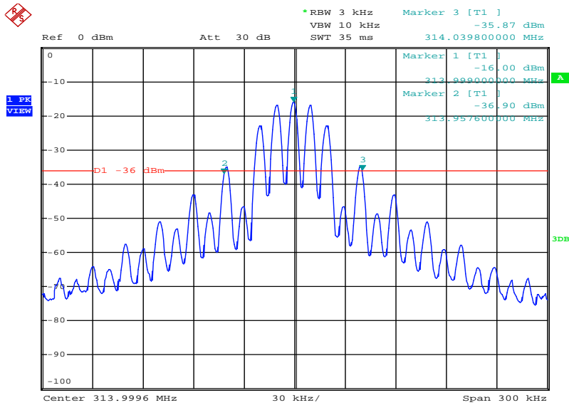
Plot 2: 20 dB Emissions bandwidth ch 1
