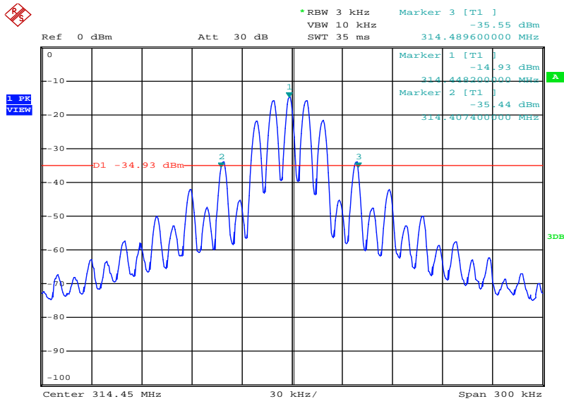
Plot 6: 20 dB Emissions bandwidth ch 3
