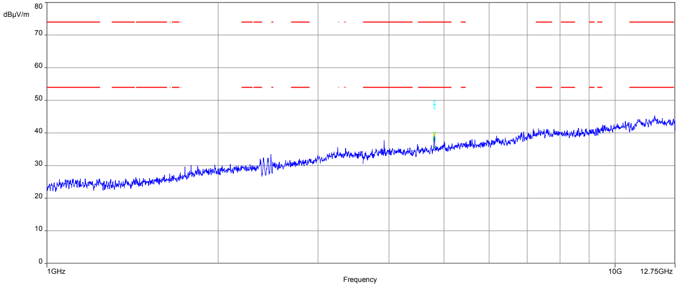
Plot 1: 1 GHz to 12.75 GHz, TX mode, 2402 MHz, vertical & horizontal polarization
