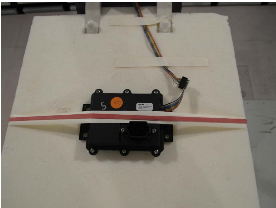
Photo 8: EUT at the anechoic chamber
