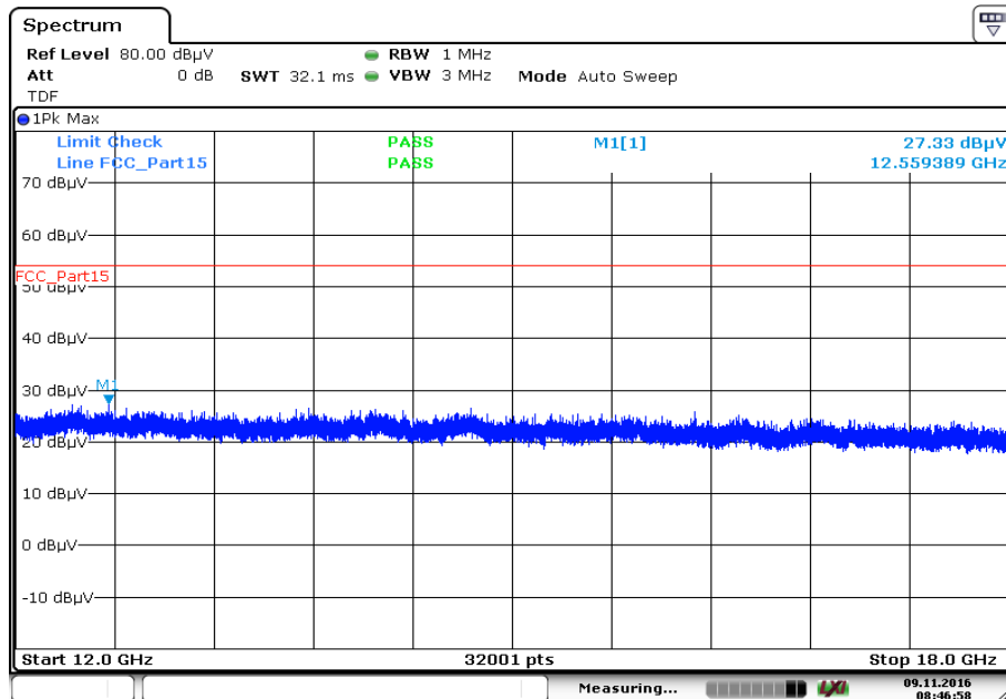
Plot 5: 12 GHz to 18 GHz, TX mode, 2440 MHz, vertical & horizontal polarization
