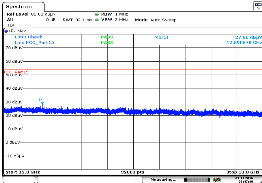
Plot 8: 12 GHz to 18 GHz, TX mode, 2480 MHz, vertical & horizontal polarization
