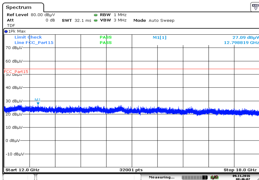
Plot 2: 12 GHz to 18 GHz, TX mode, 2402 MHz, vertical & horizontal polarization
