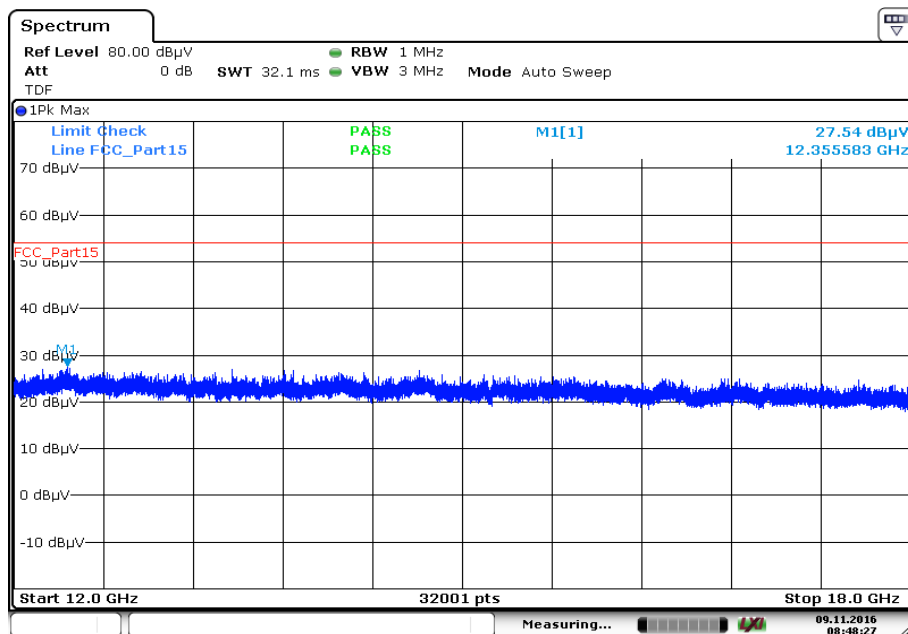
Plot 2: 12 GHz to 18 GHz, RX / idle – mode, vertical & horizontal polarization
