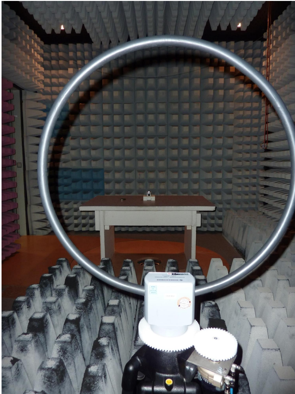
161842_1.JPG: Test setup fully anechoic chamber
