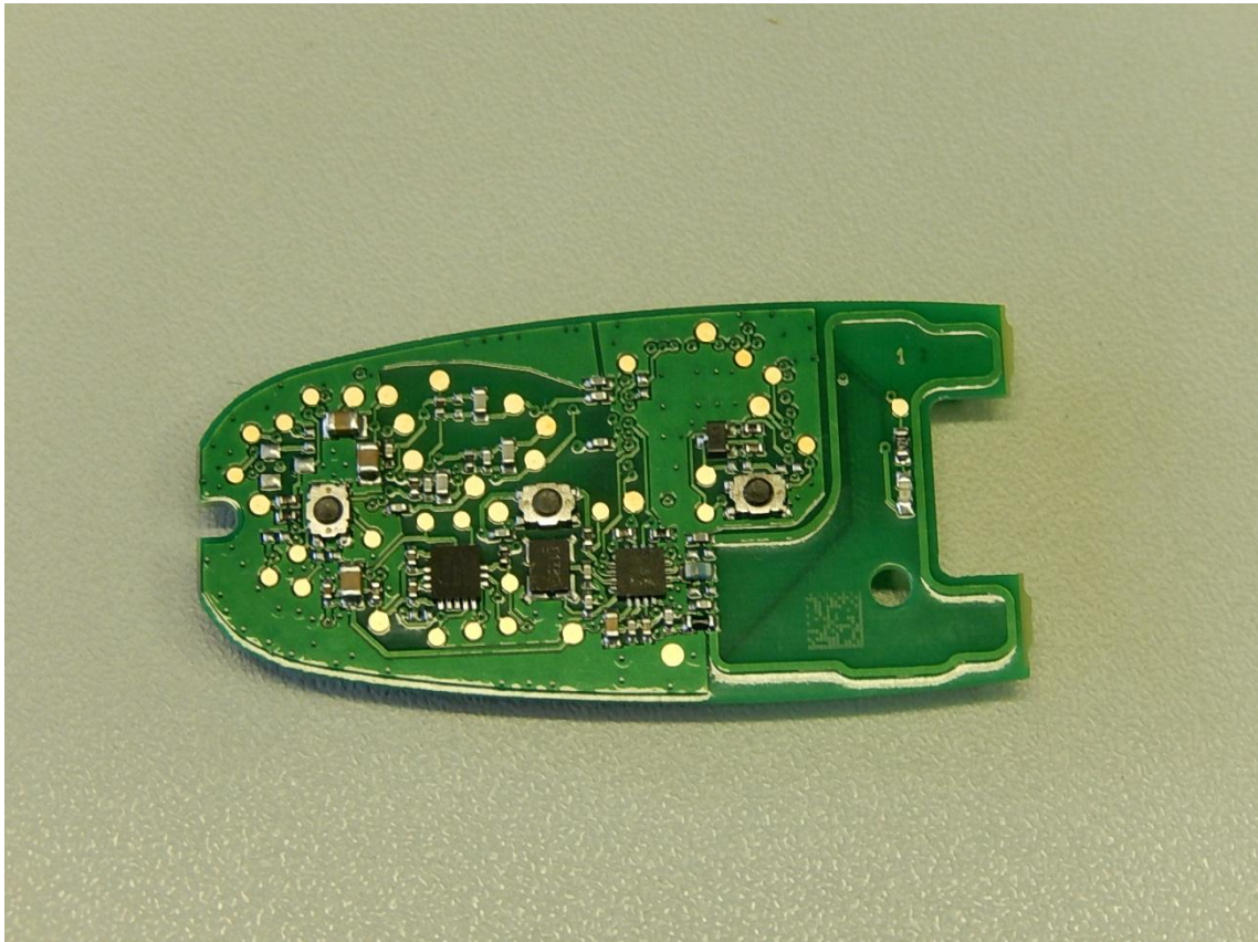
161842_12.JPG: PCB, top view
