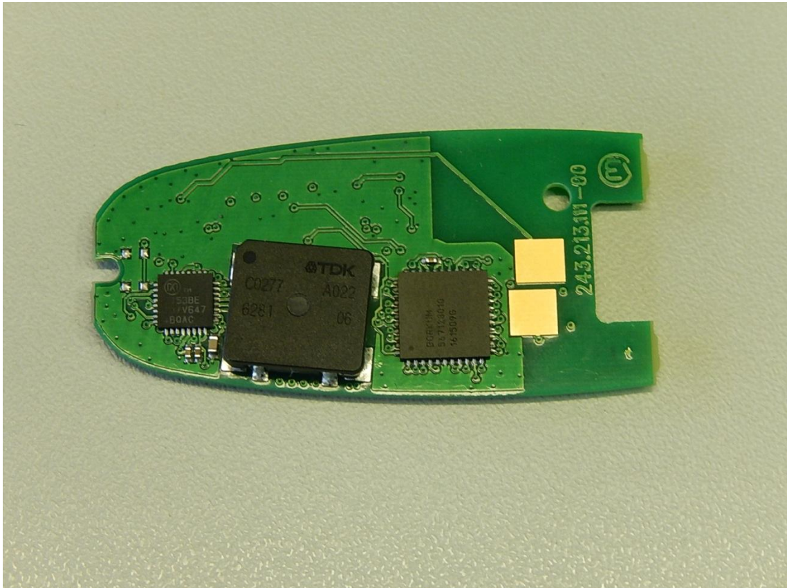
161842_11.JPG: PCB, bottom view
