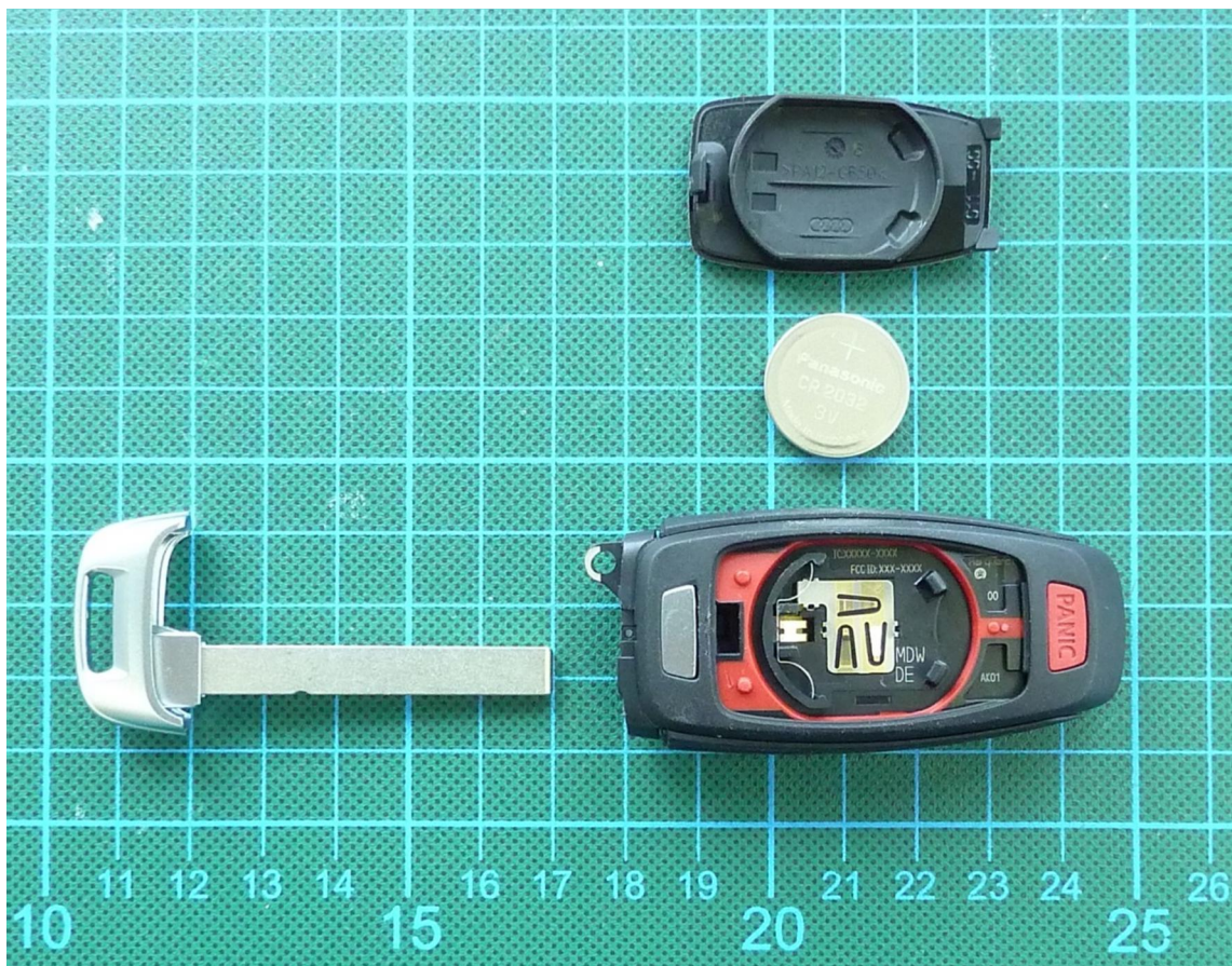
161842_9.JPG: AK2 Basis, bottom view (battery cover removed)
