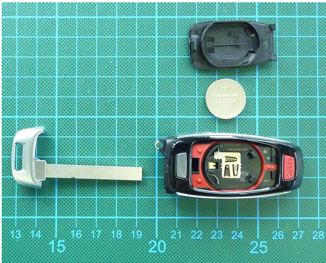
161842_10.JPG: AK2 Comfort, bottom view (battery cover removed)
