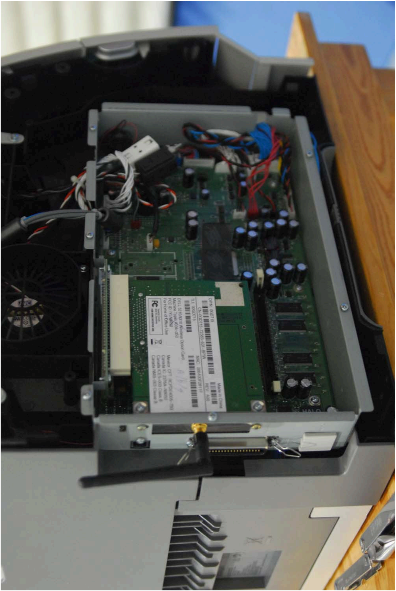
Figure 7: Installation of FCCID: IYLN8052 in a Host Printer (cover removed for clarity)
