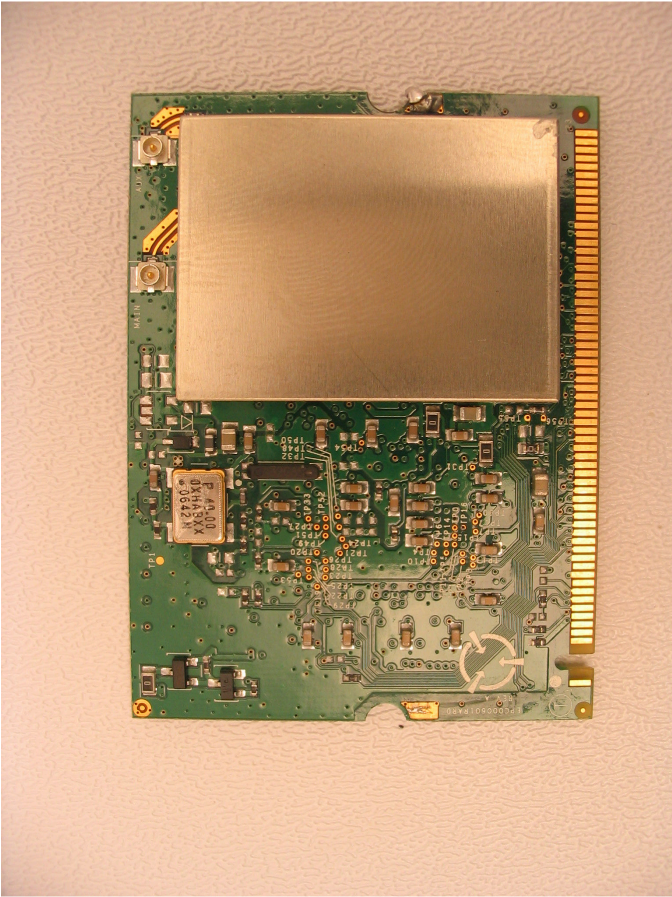
Figure 4: Top Side of the 802.11 Module
