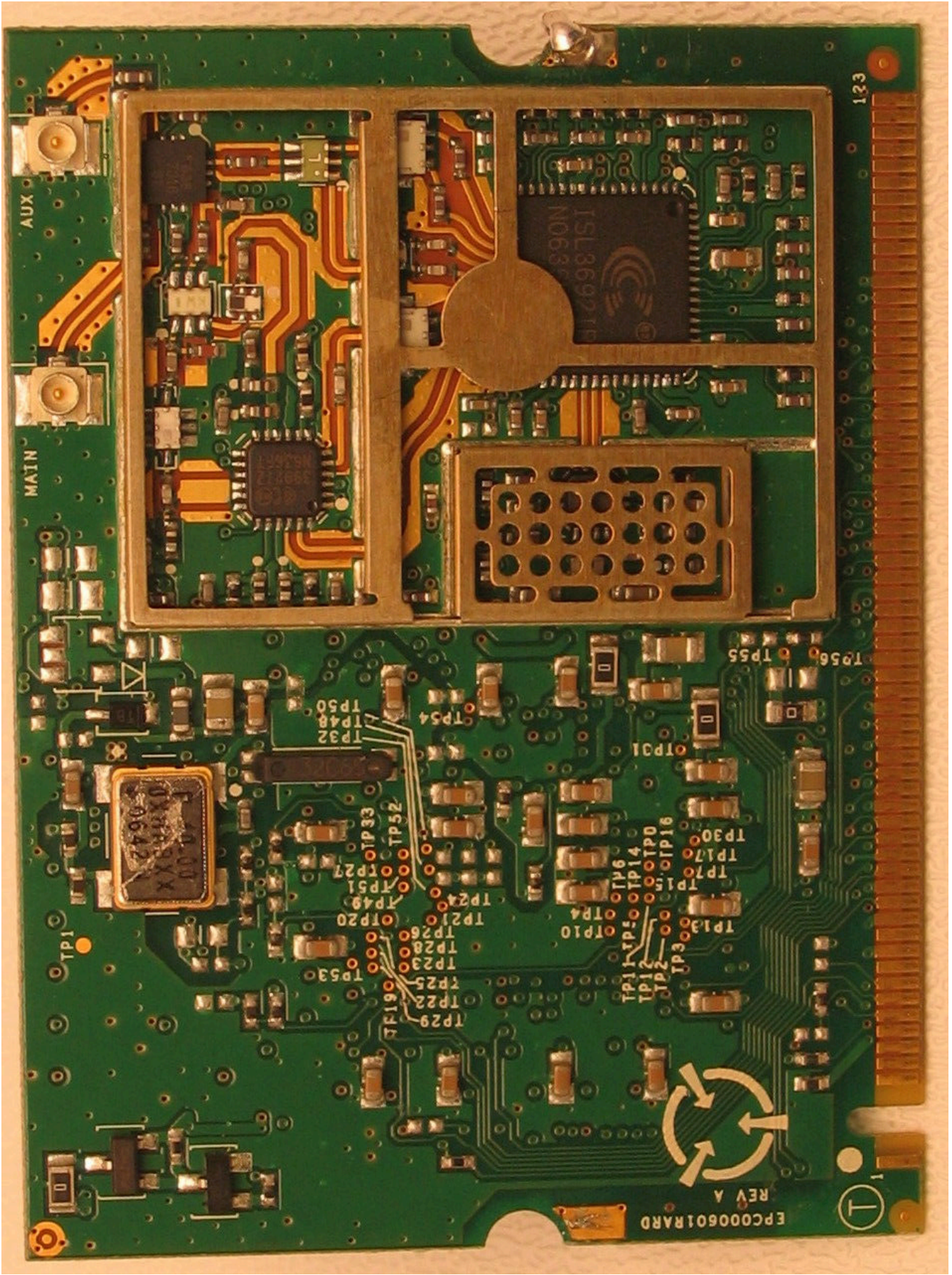
Figure 5: Top Side of the 802.11 Module with the Shield Removed
