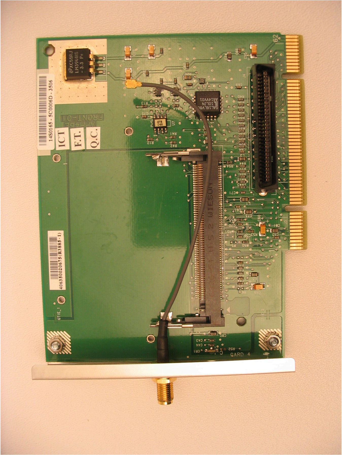
Figure 3: Top Side of Board with the 802.11 Module Removed
