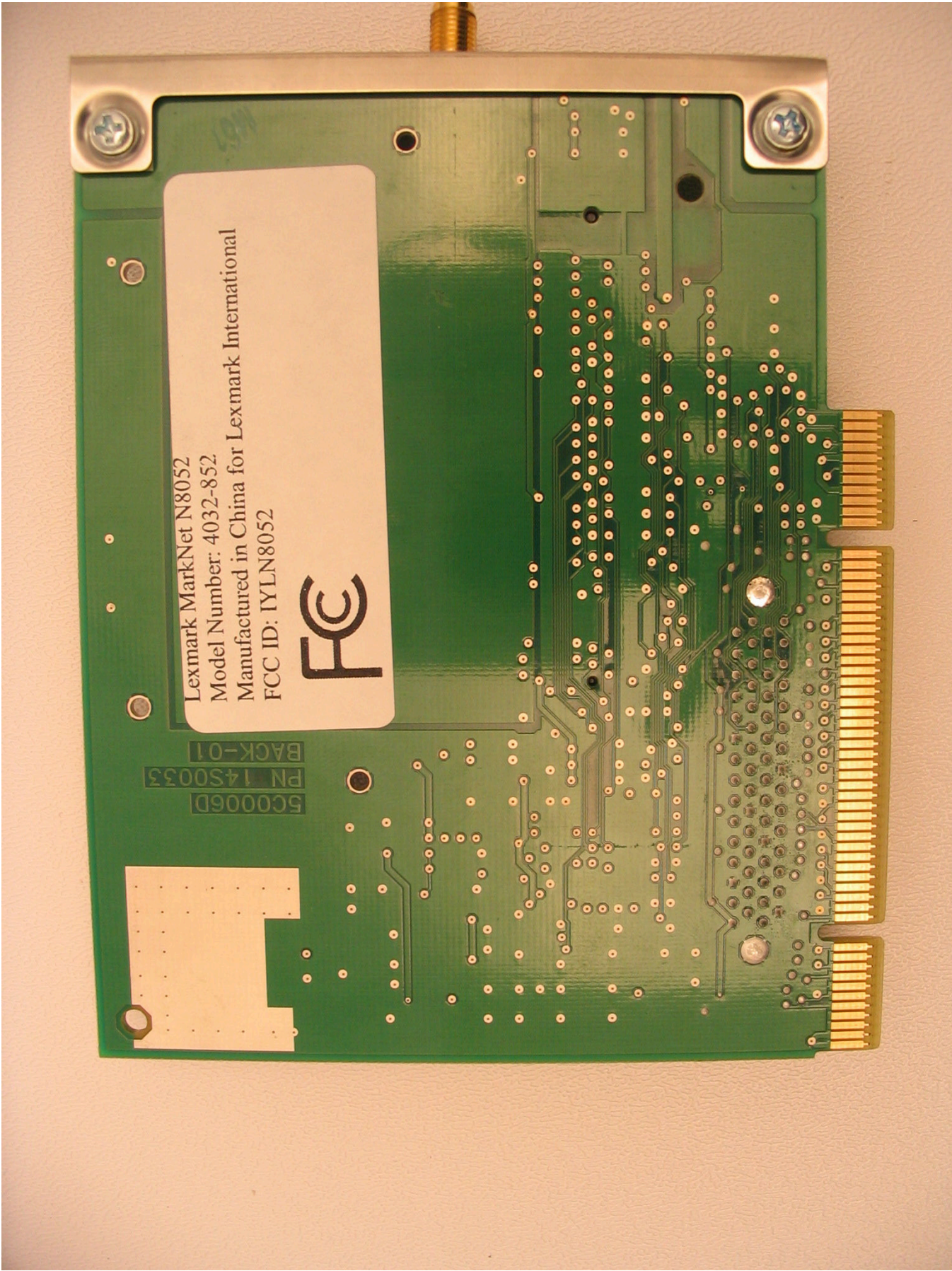
Figure 2: Bottom Side of Board
