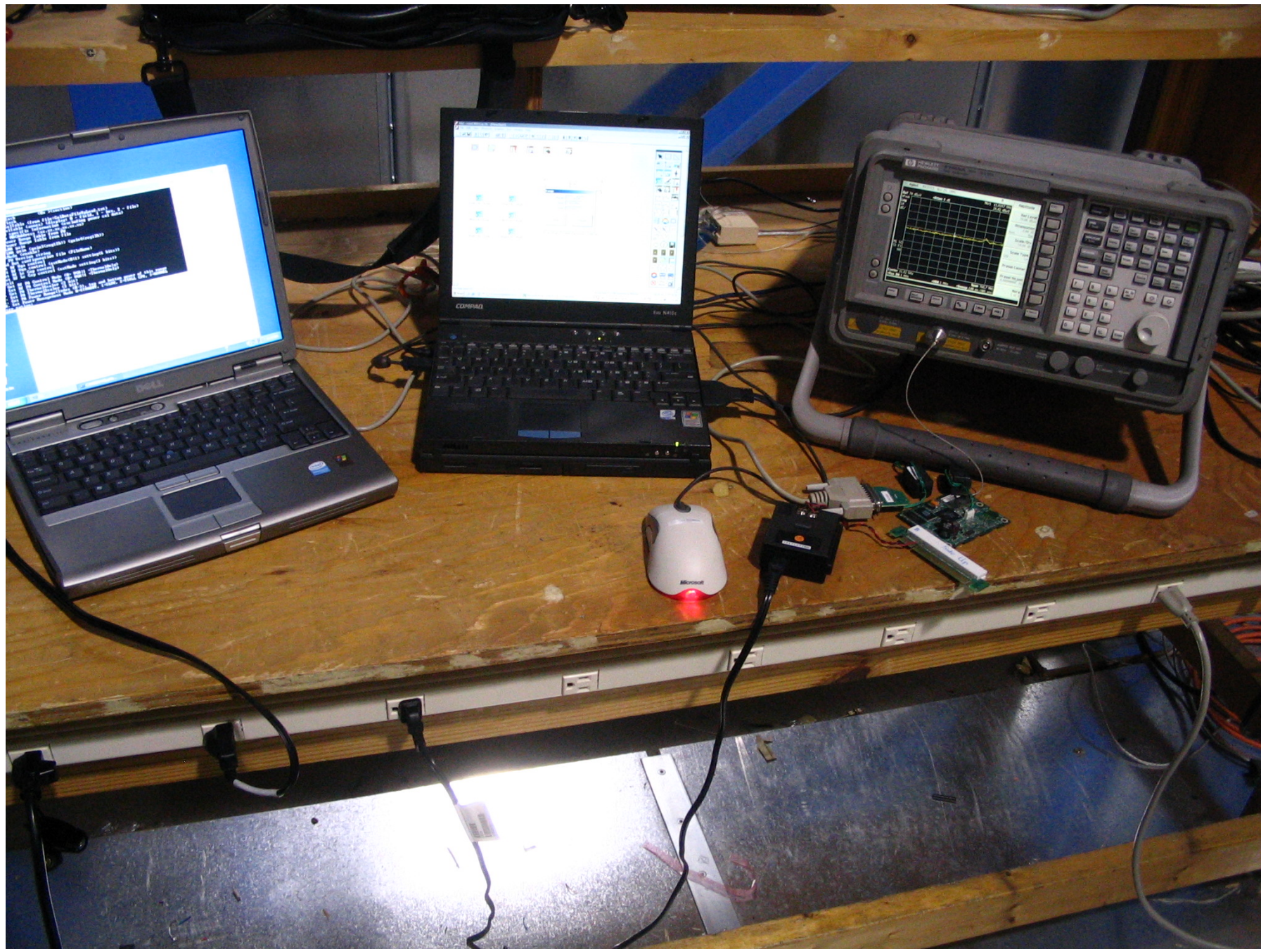
Figure 4: Conducted Emissions and Power Measurements
