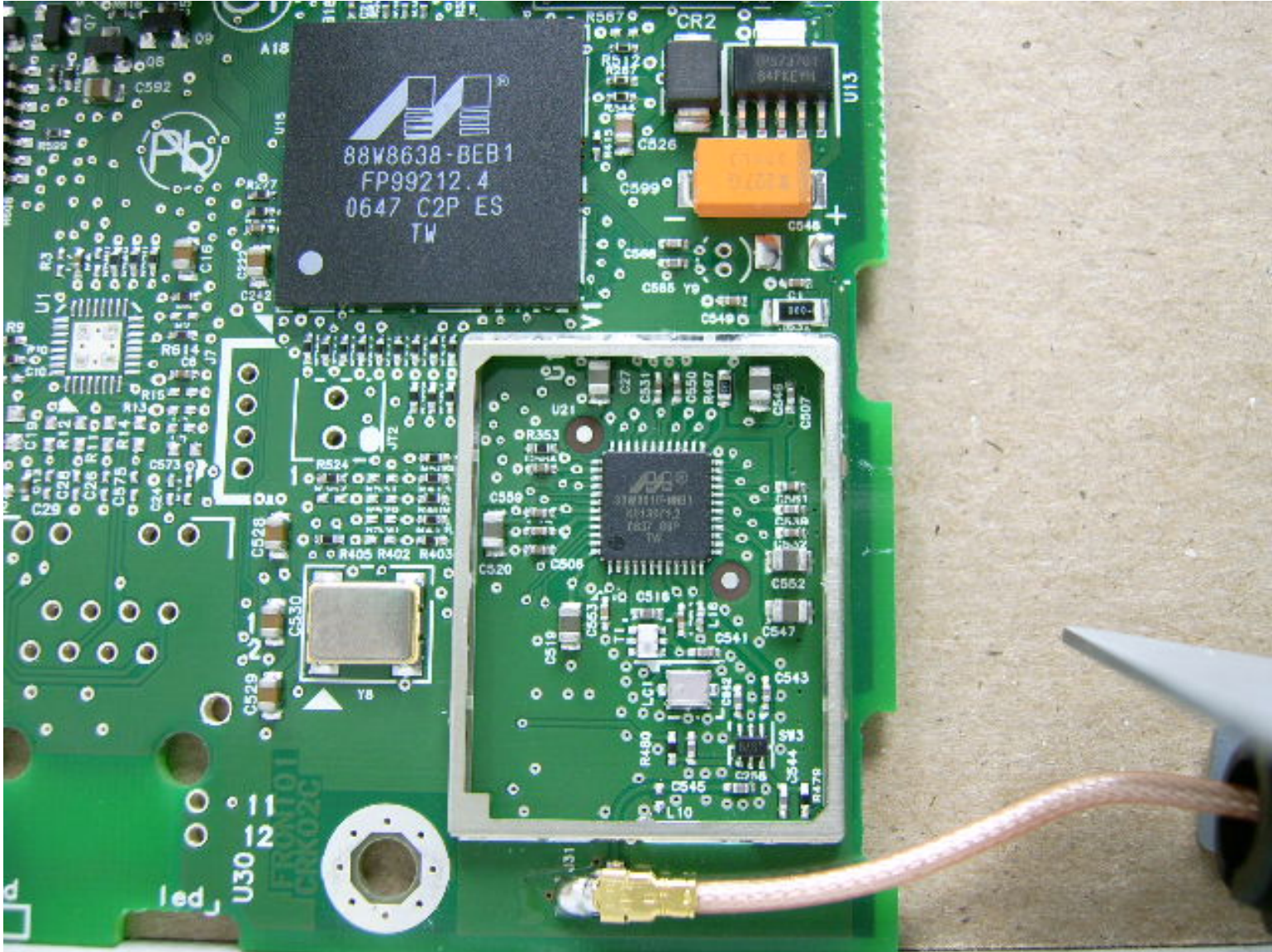
Figure 6: Behind Shielded off Area #2
