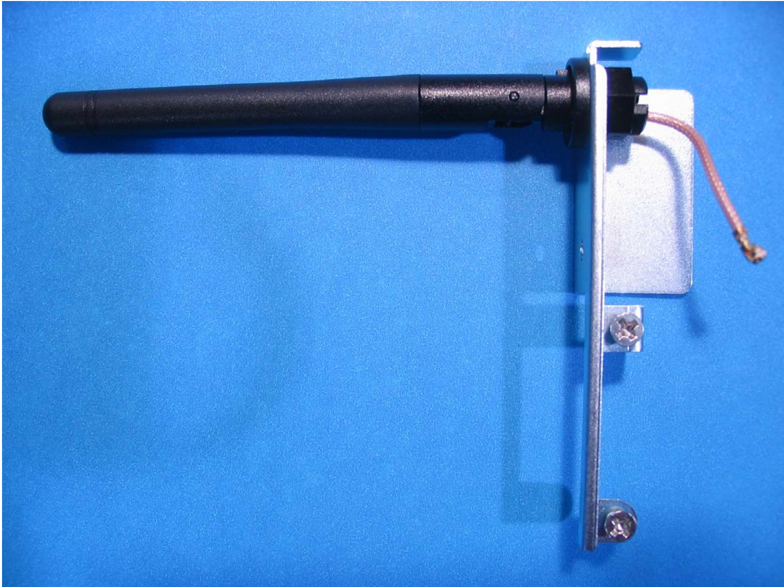
Figure 4: Antenna Assembly
