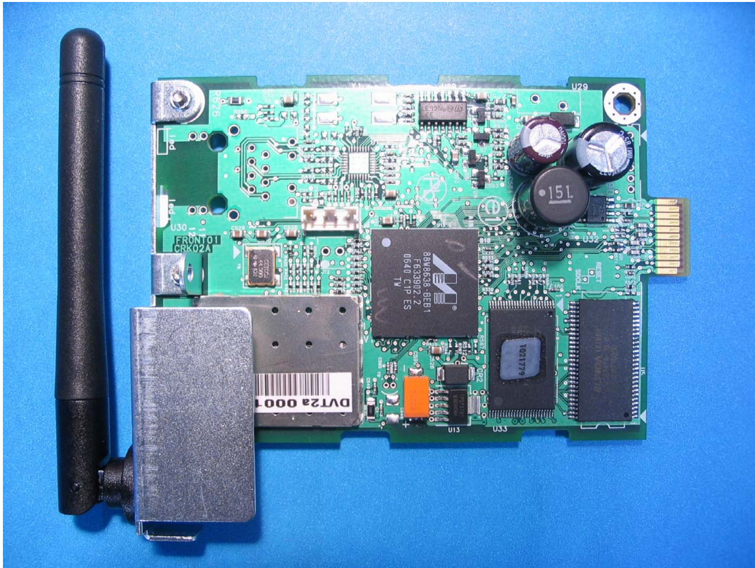
Figure 1: N2050 Card and Antenna Top View
