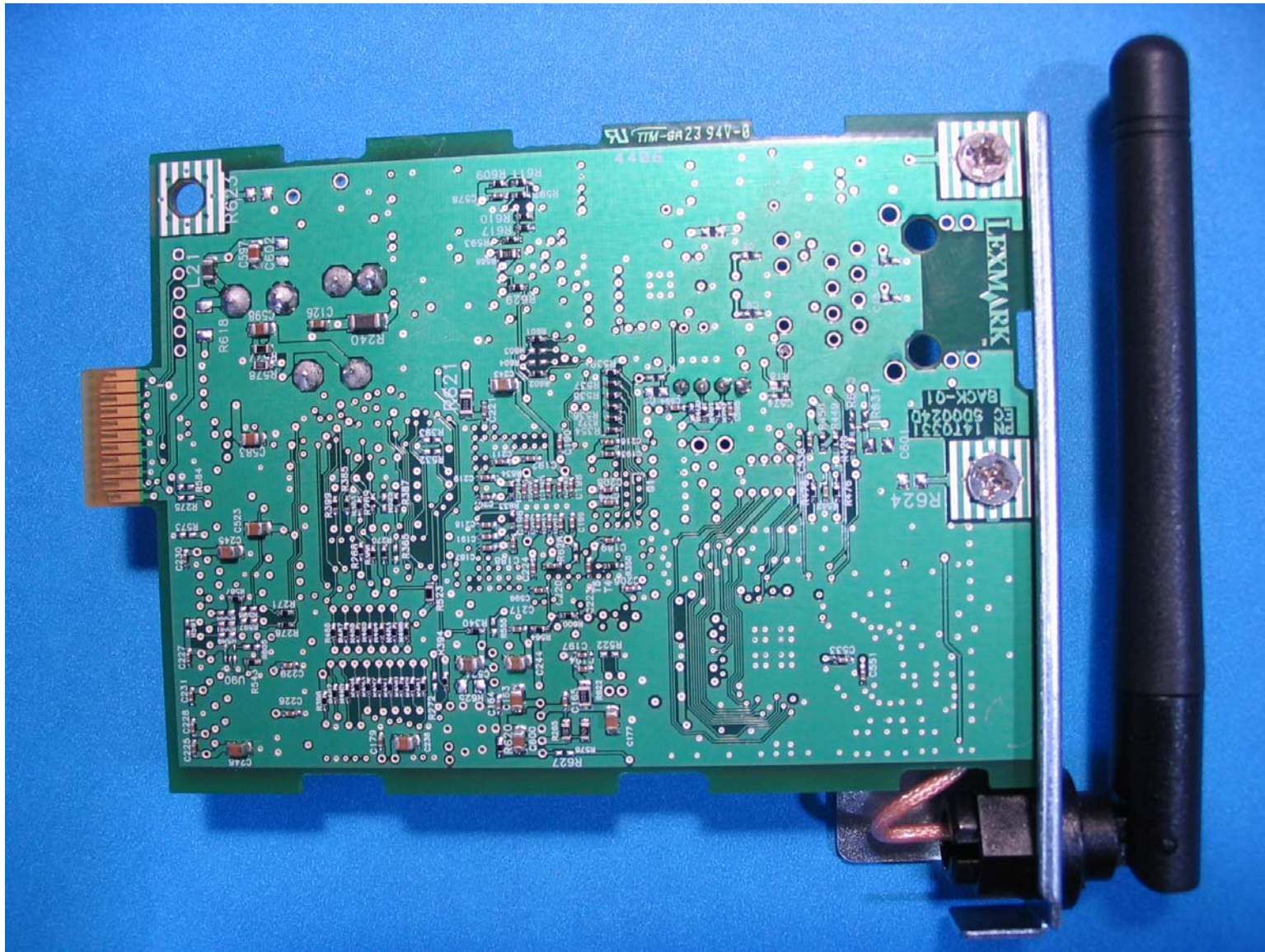
Figure 2: N2050 Card and Antenna Bottom View
