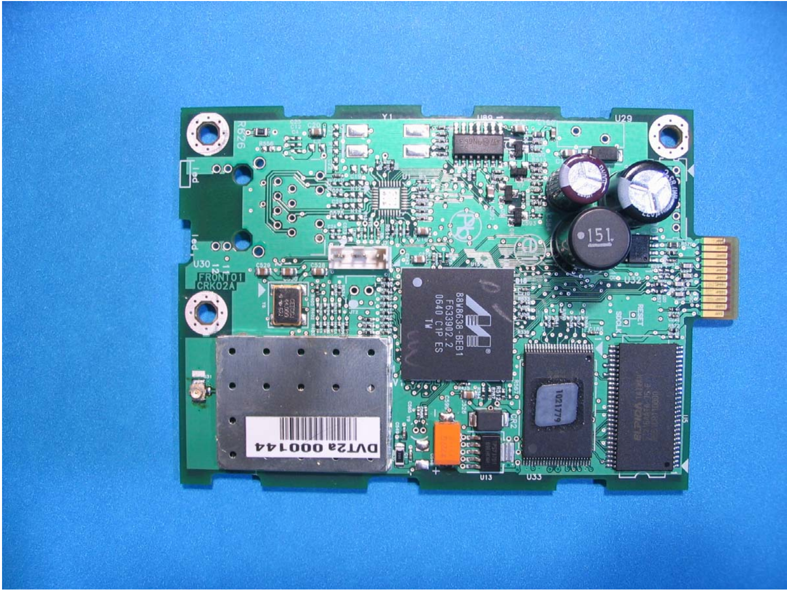
Figure 3: N2050 Card and Antenna Top View Antenna Removed
