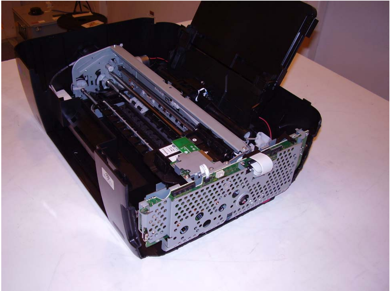
Side view of EUT mounted in printer engine frame with black plastic covers (plastic sidewall cut away for access).
