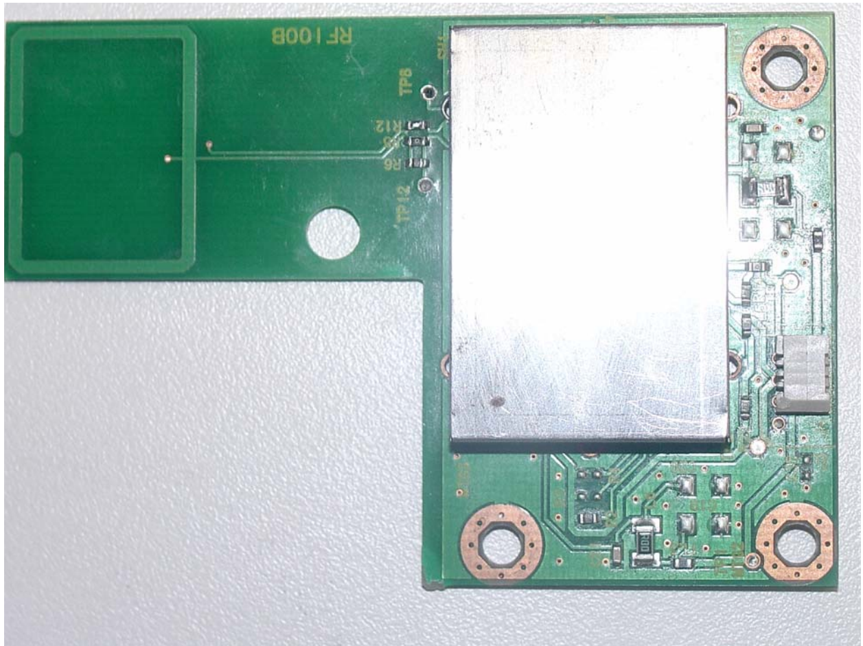
Top side of EUT.
