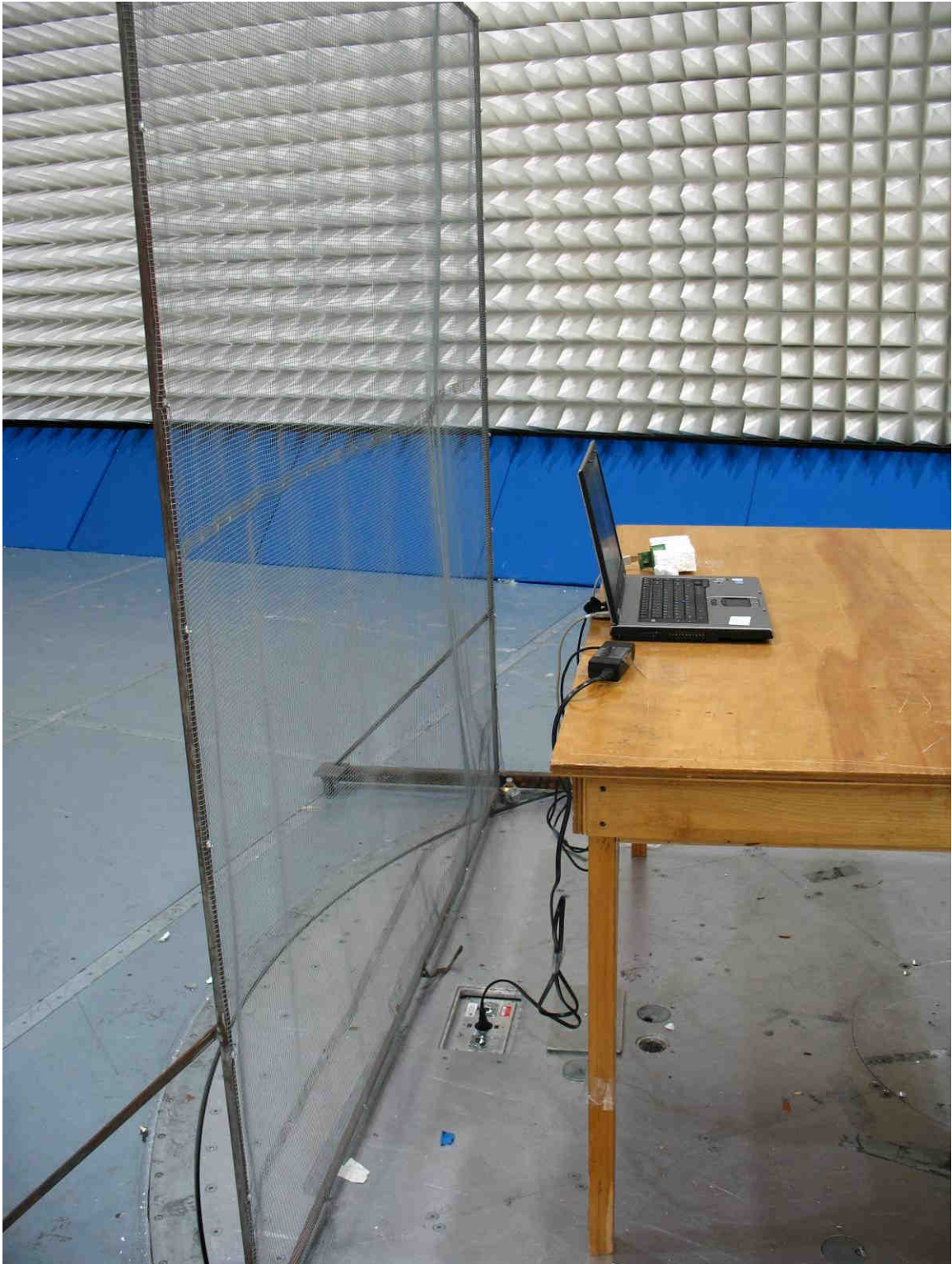
Conducted Emissions (Side)
