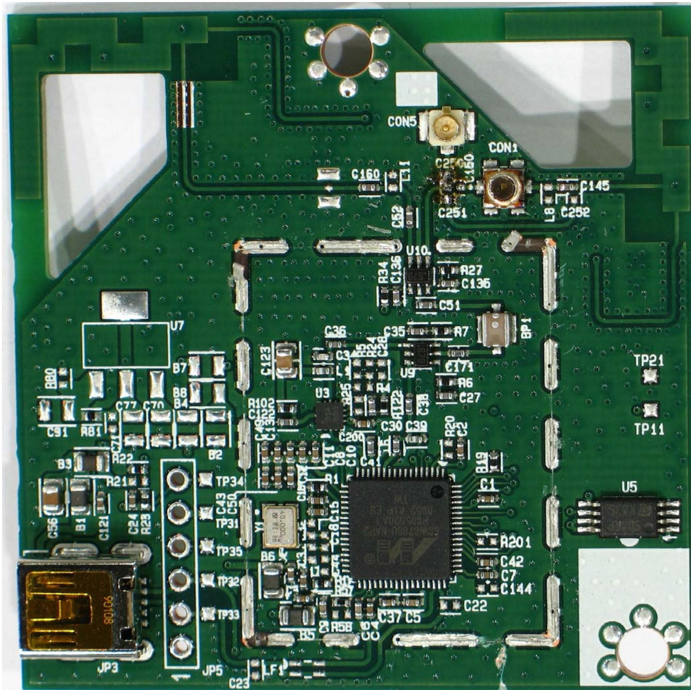
Front Side of PCB (Shield Removed)
