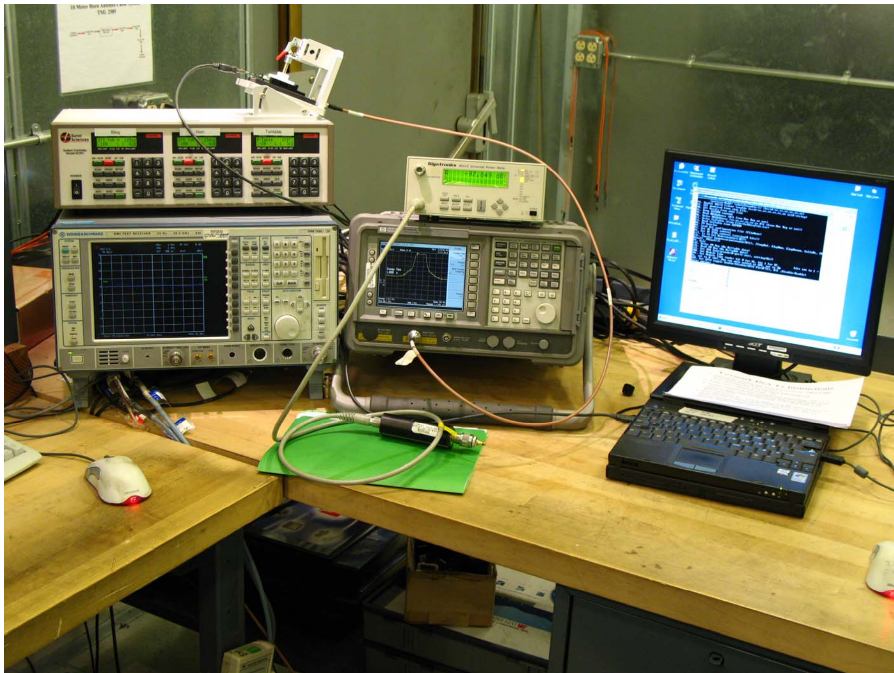
Conducted Measurements at Antenna Terminals
