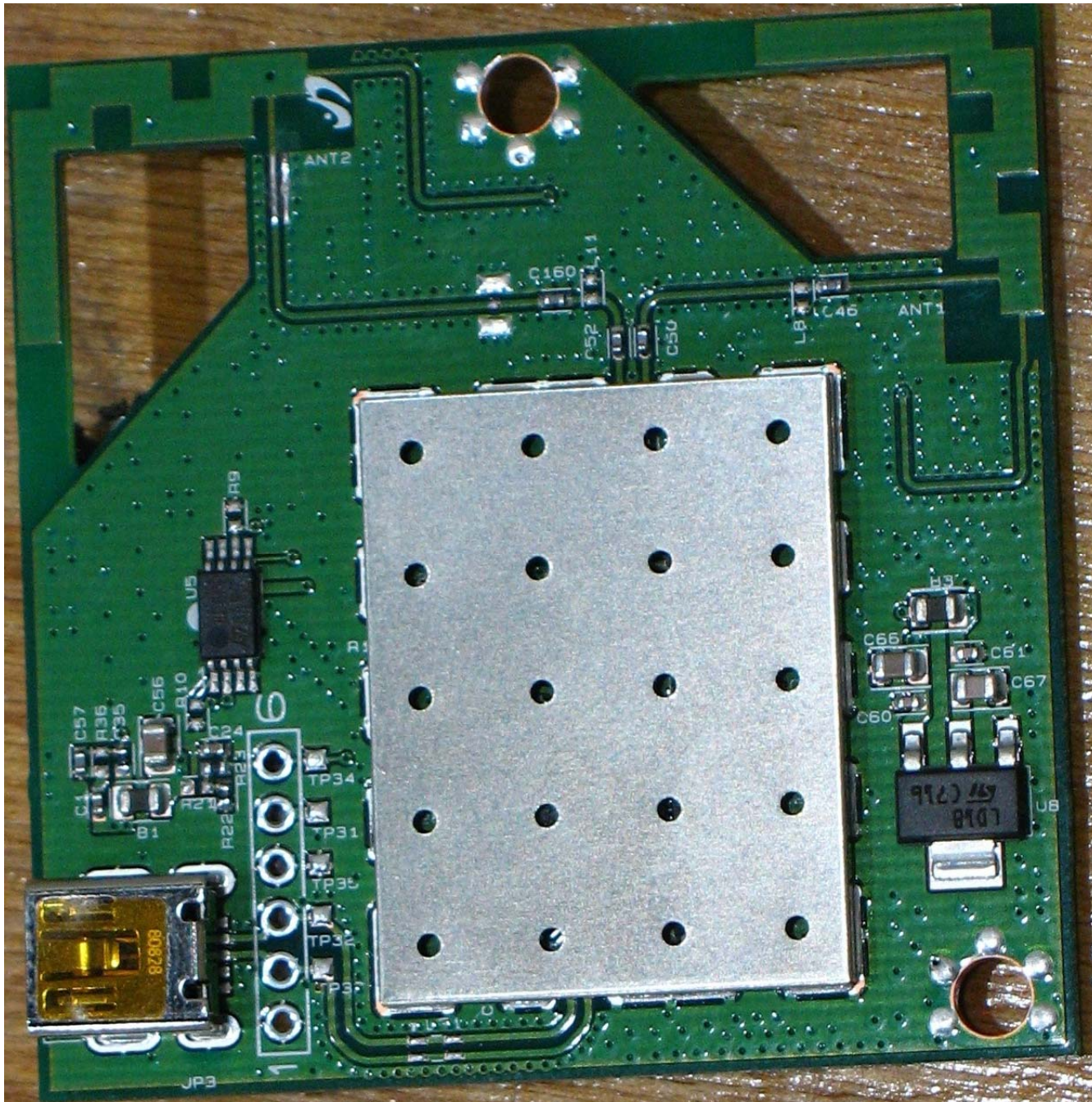
Front Side of PCB (Shield In Place)
