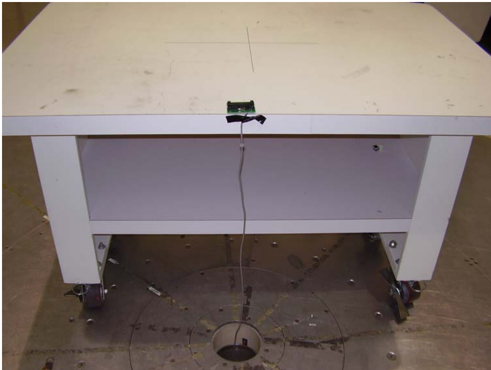
Test configuration for transmitter radiated emissions (back view).
