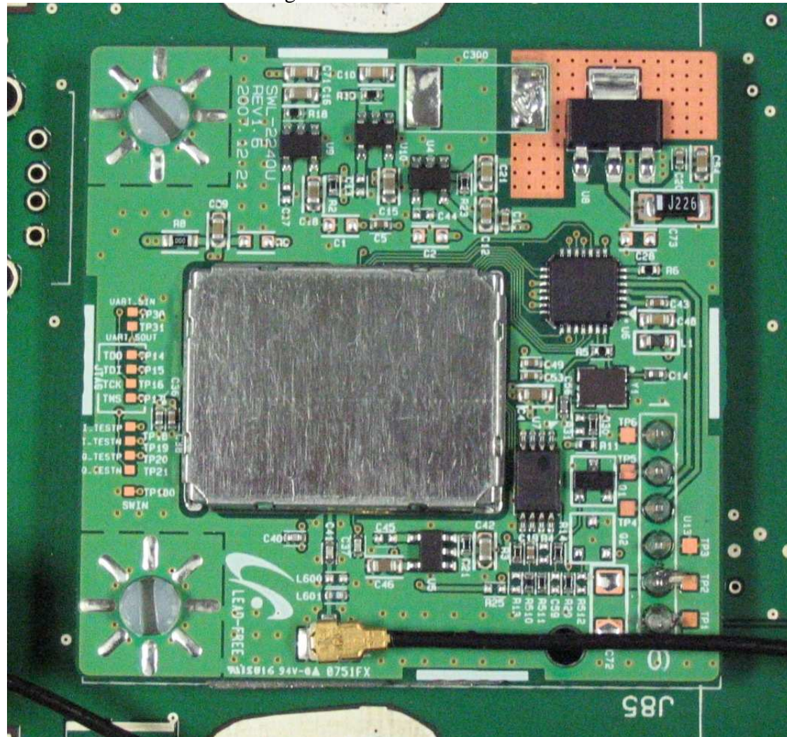
Alternate Configuration – Module Soldered to Host PCB
