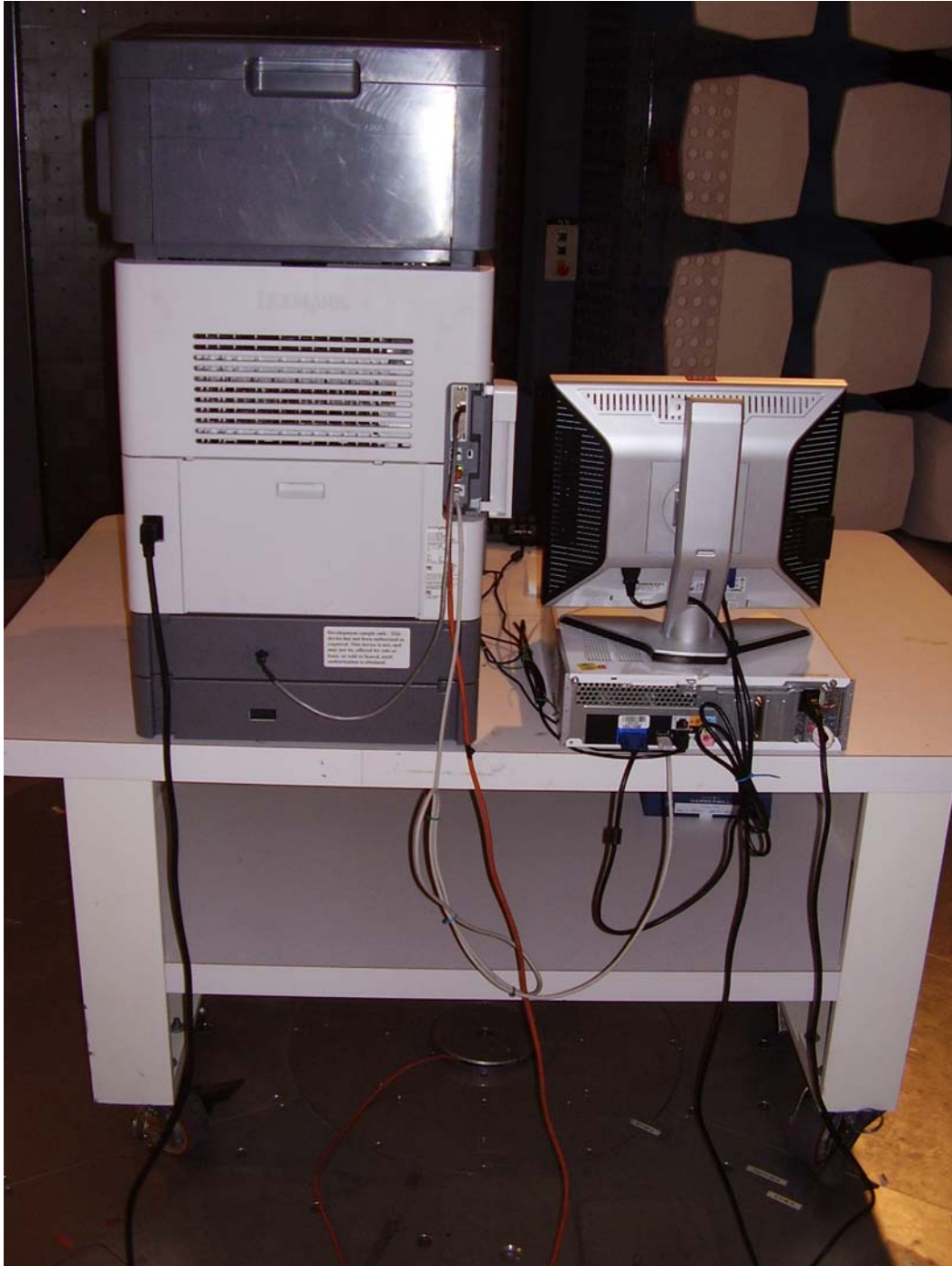
Test configuration for transmitter radiated spurious emissions (back view).
