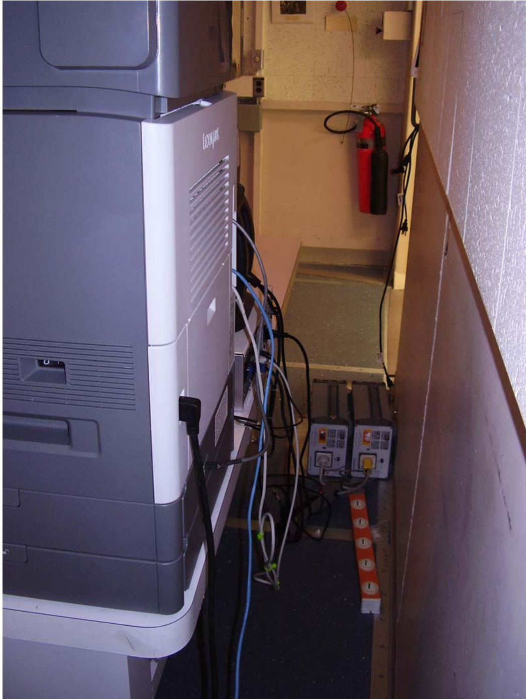
Test configuration for transmitter AC conducted emissions (side view).
