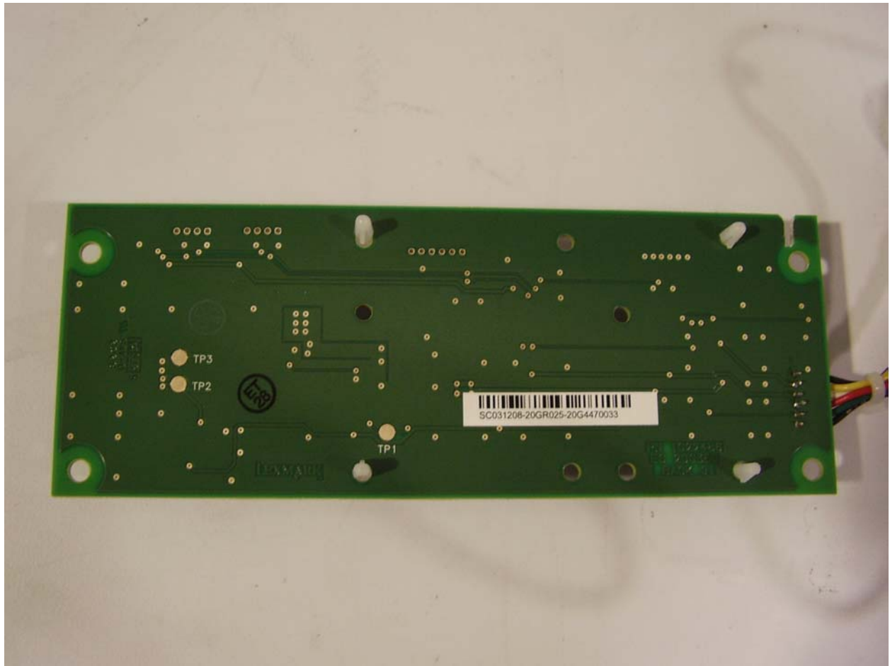
Back view of radio interface card.
