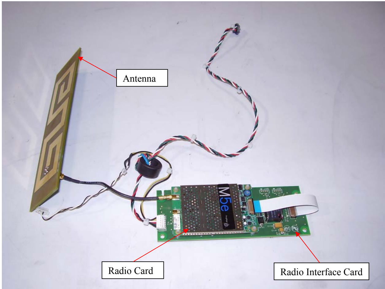
Top view of antenna and radio assembly without mounting bracket.
