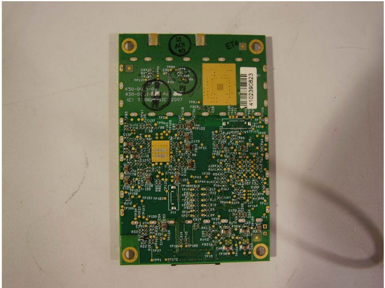
Back view of radio card.
