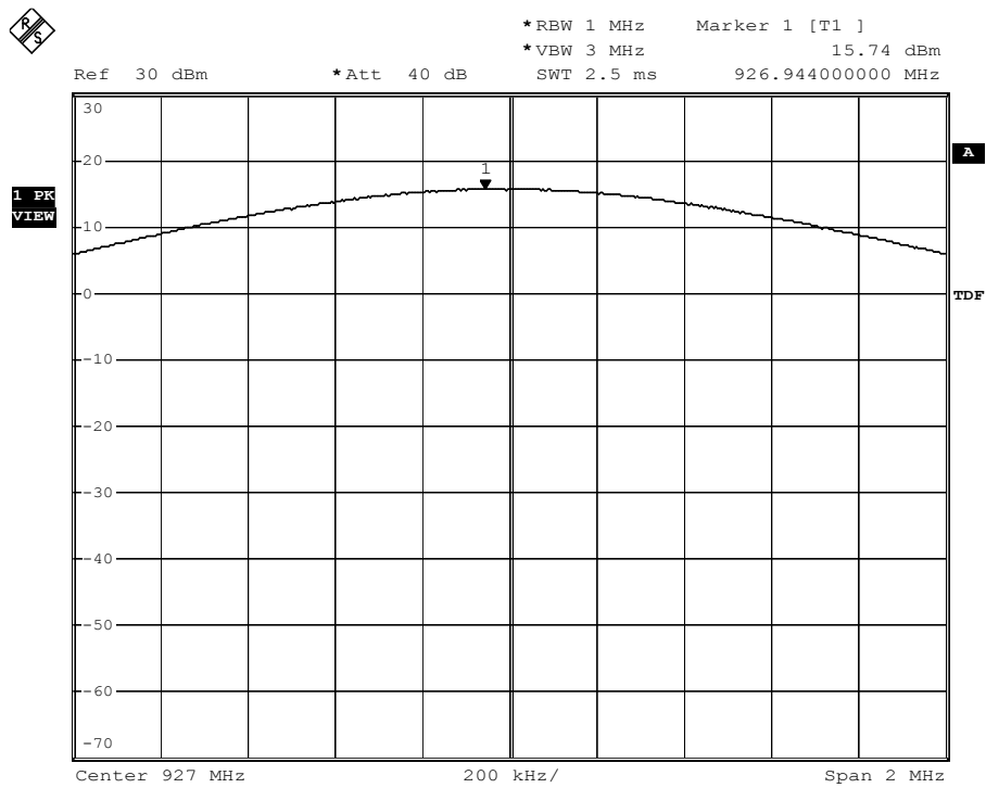
Figure 35. Conducted output power (low power setting); Channel 50, 115% nominal voltage.
