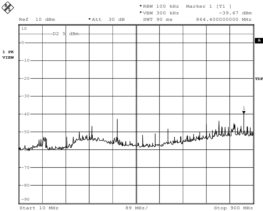
Figure 37. Out of band emissions at antenna port; 10 MHz - 900 MHz.
