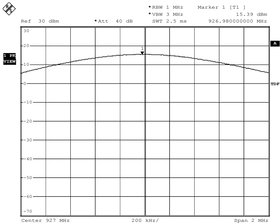
Figure 29. Conducted output power (low power setting); Channel 50, nominal voltage.
