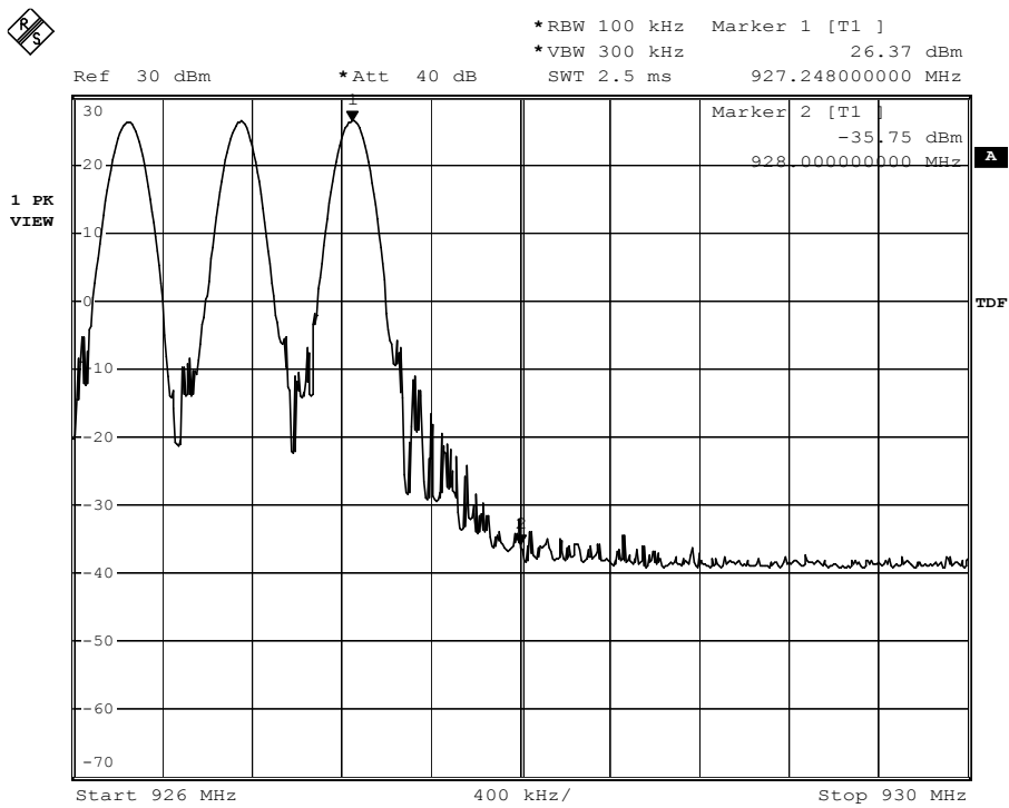
Figure 43. Band edge compliance; EPC Gen2 mode; Channel 50, hopping enabled.
