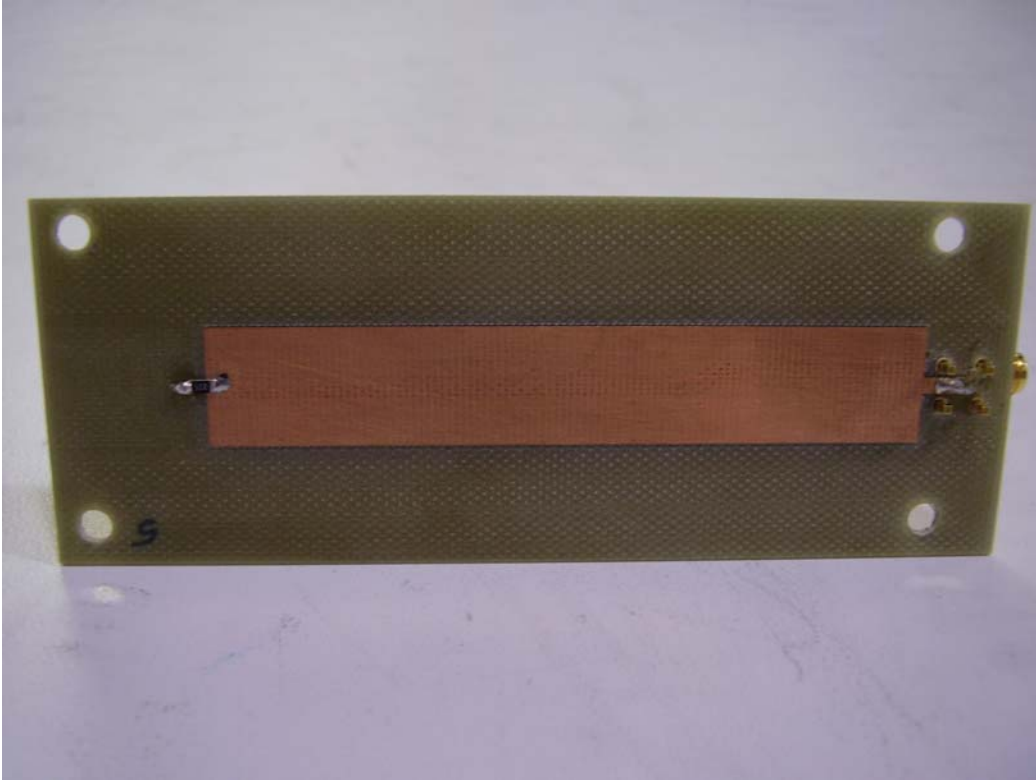
Figure 5. Front view of antenna removed from EUT.
