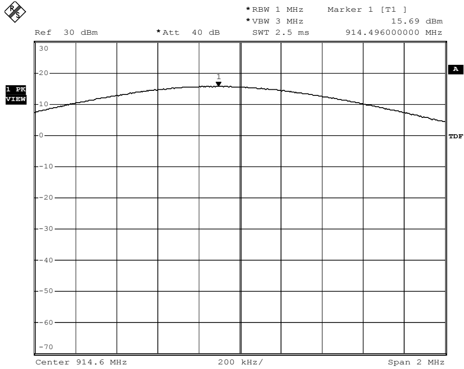
Figure 34. Conducted output power (low power setting); Channel 25, 115% nominal voltage.
