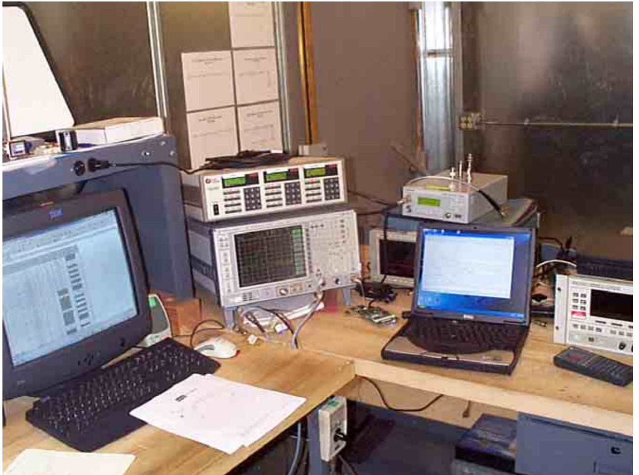
Figure 1: Conducted Testing
