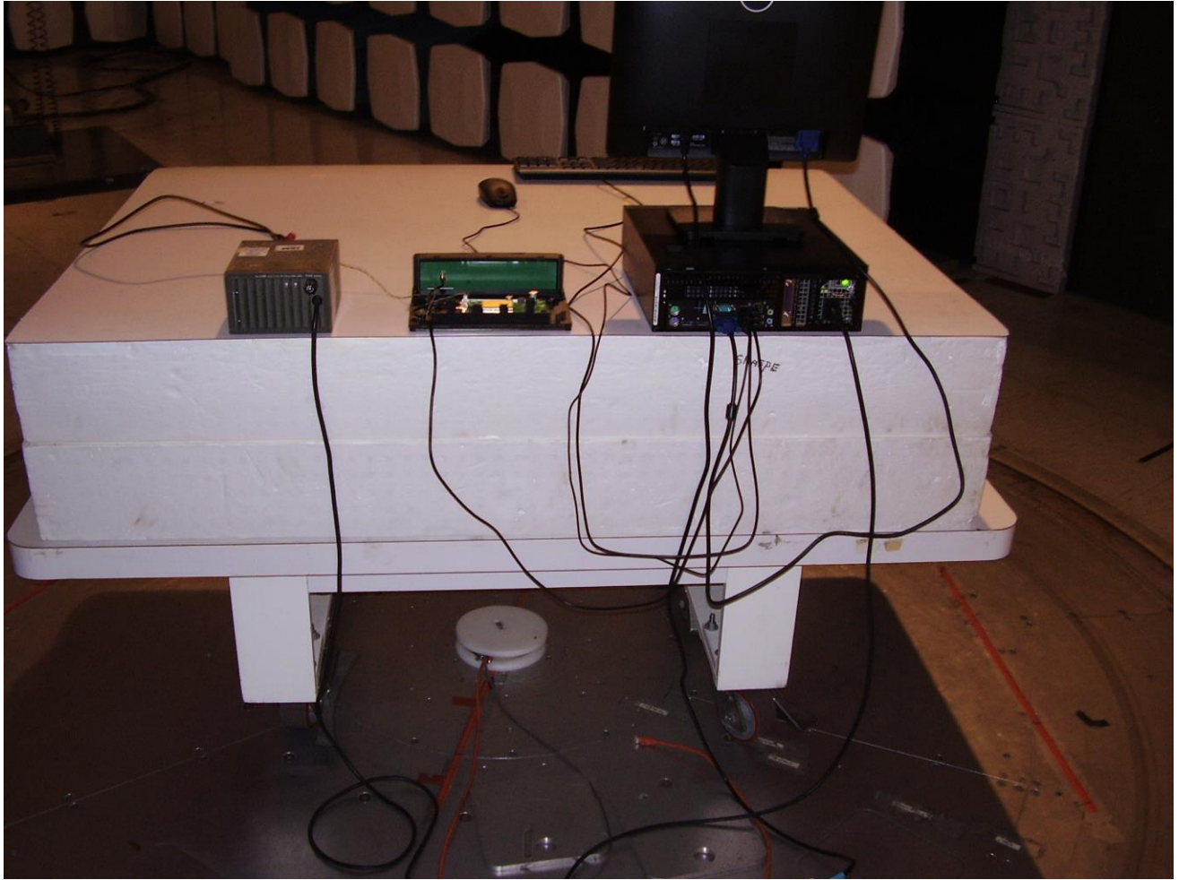
Test configuration for transmitter radiated spurious emissions 30 – 1000 MHz (back view).
