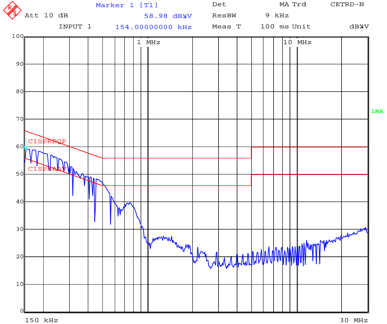
Plot 1, AC Wireline Conducted Emissions Line N (Neutral)
