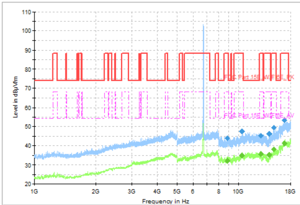
Fig. 39 Transmitter Spurious Emission (802.11ax-HE40, CH155, 1GHz-18GHz)
