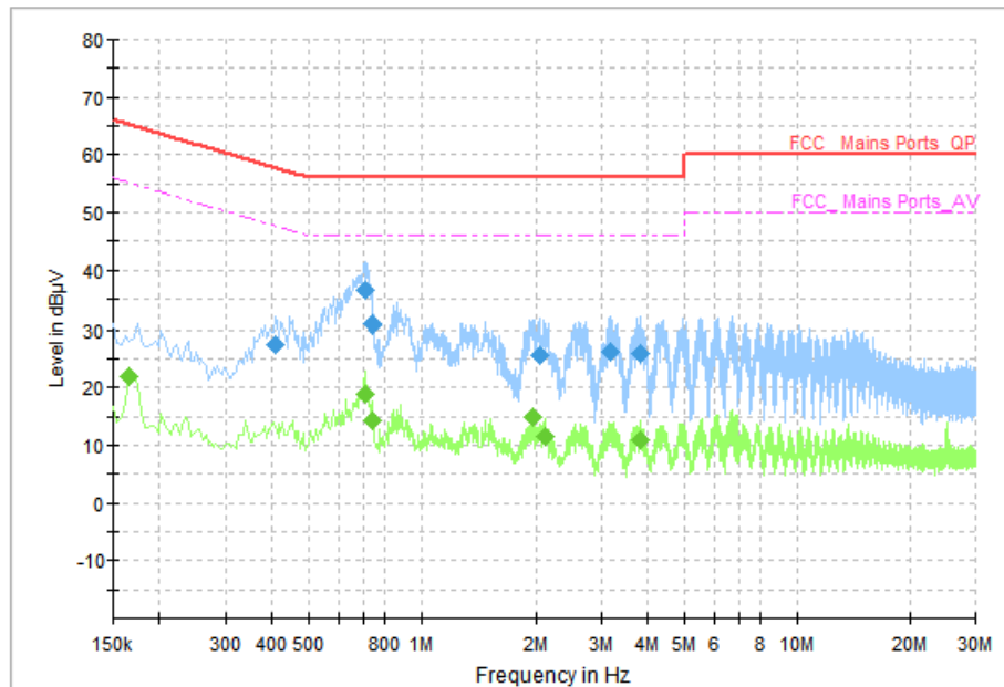
Fig. 62 AC Power line Conducted Emission (Idle)
