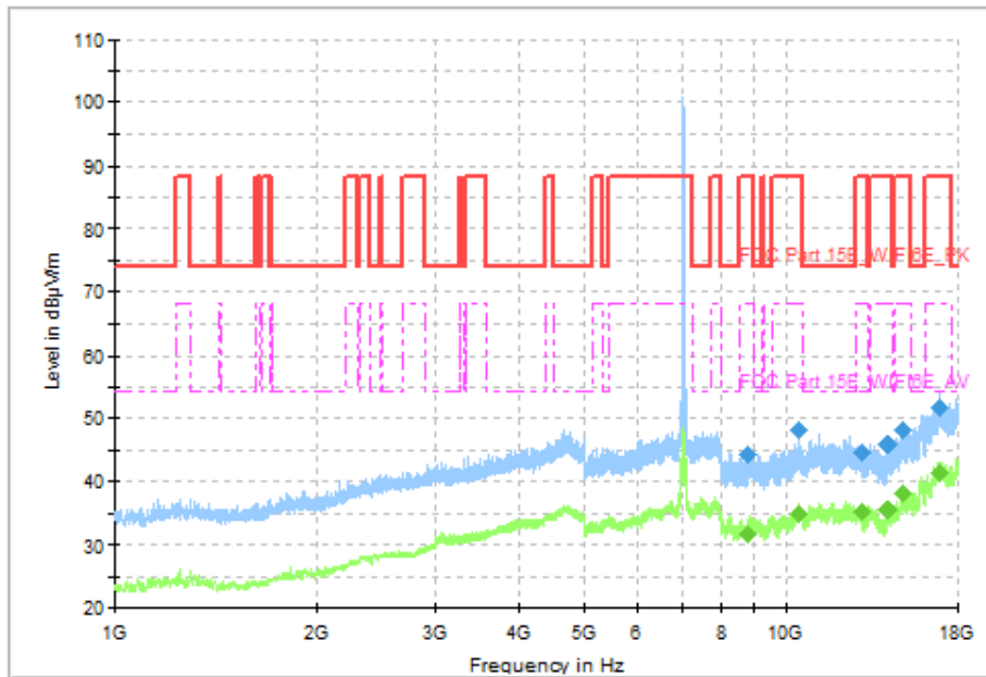
Fig. 49 Transmitter Spurious Emission (802.11ax-HE80, CH211, 1GHz-18GHz)
