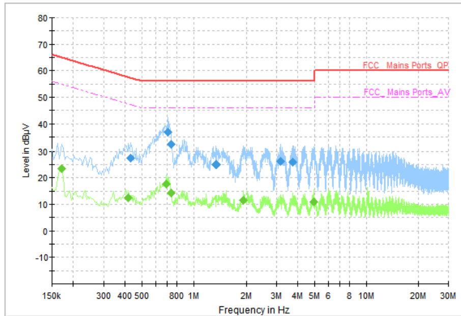
Fig. 61 AC Power line Conducted Emission (Traffic)
