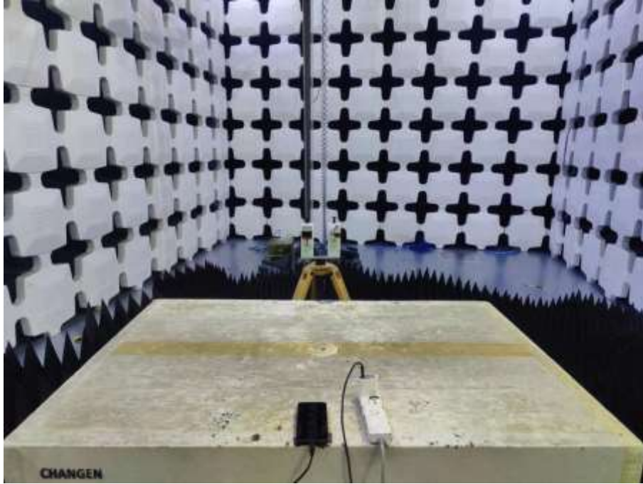
7. Radiated Emissions (Part 15B, Camera/Video Player/Scan QR code, 18GHz-26.5GHz)
