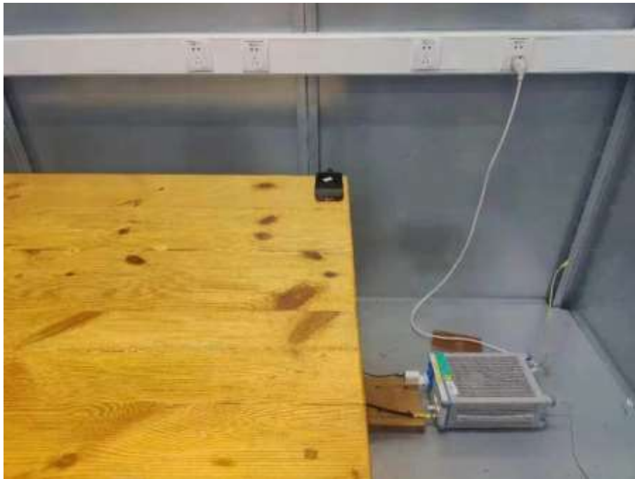
14. Conducted Emission (Part 15B& Part 15C&E, Camera/Video Player/Scan QR code/ Wi-Fi/Bluetooth)
