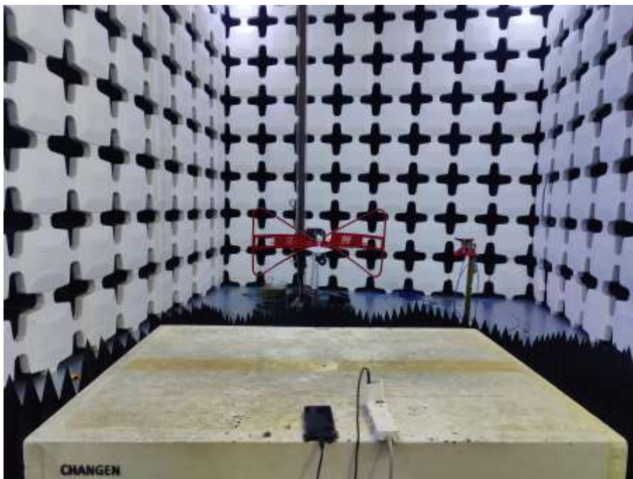
6. Radiated Emissions (Part 15B, Camera/Video Player/Scan QR code,1GHz-18GHz)
