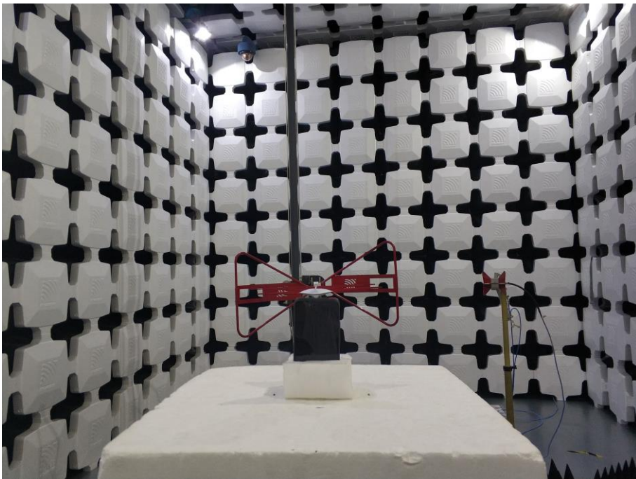
2. Radiated Emissions (Part 15C&15E 30M-18GHz)
