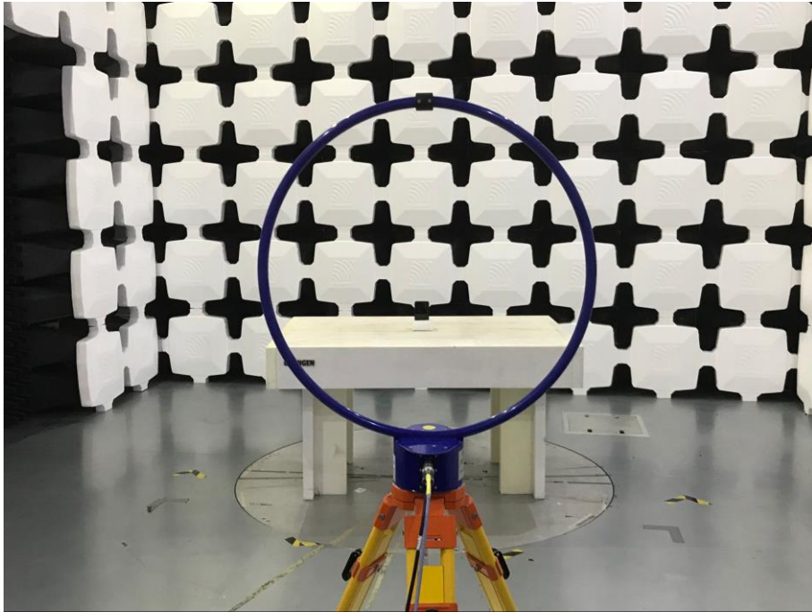
1. Radiated Emissions (Part 15C&15E 9kHz-30MHz)
