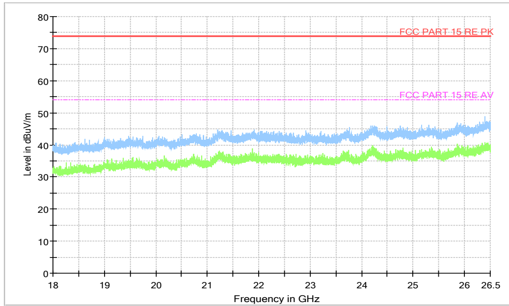
Fig. 27 Radiated Spurious Emission (All Channels, 18 GHz ~26.5 GHz)
