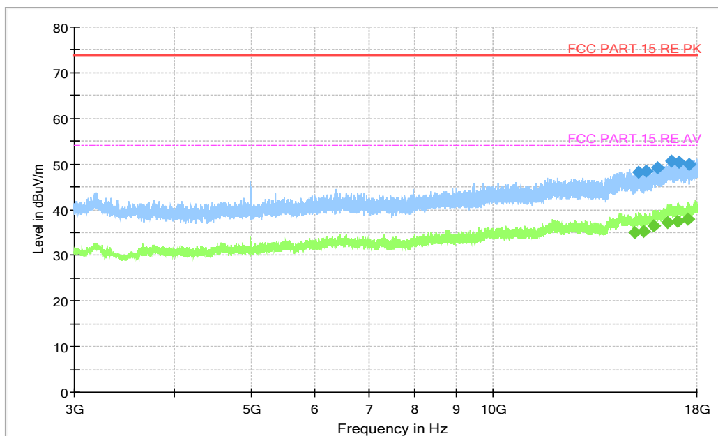
Fig. 6 Radiated Spurious Emission (GFSK, Ch78, 3 GHz ~18 GHz)
