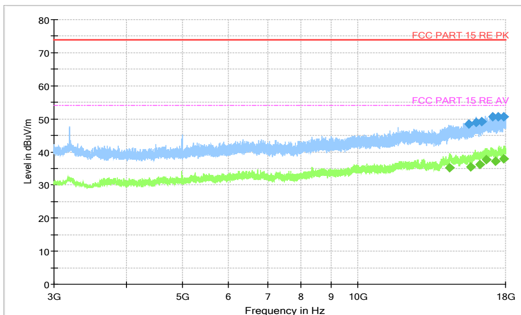
Fig. 4 Radiated Spurious Emission (GFSK, Ch39, 3 GHz ~18 GHz)
