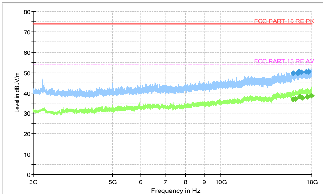
Fig. 10 Radiated Spurious Emission ( \pi/4 DQPSK, Ch0, 3 GHz ~18 GHz)
