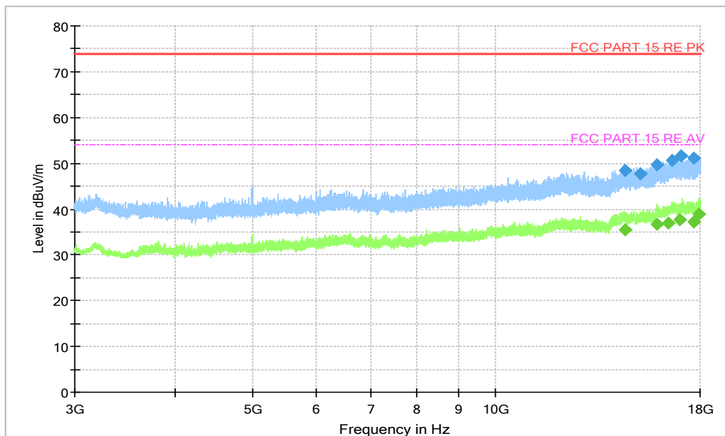
Fig. 18 Radiated Spurious Emission (8DPSK, Ch0, 3 GHz ~18 GHz)
