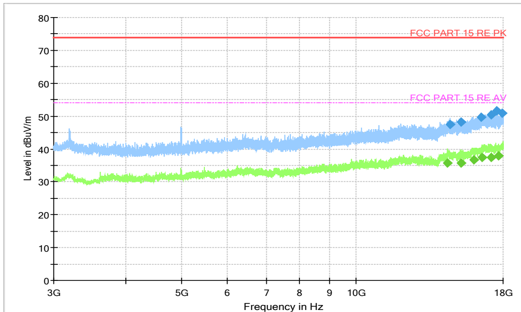
Fig. 14 Radiated Spurious Emission ( \pi/4 DQPSK, Ch78, 3 GHz ~18 GHz)
