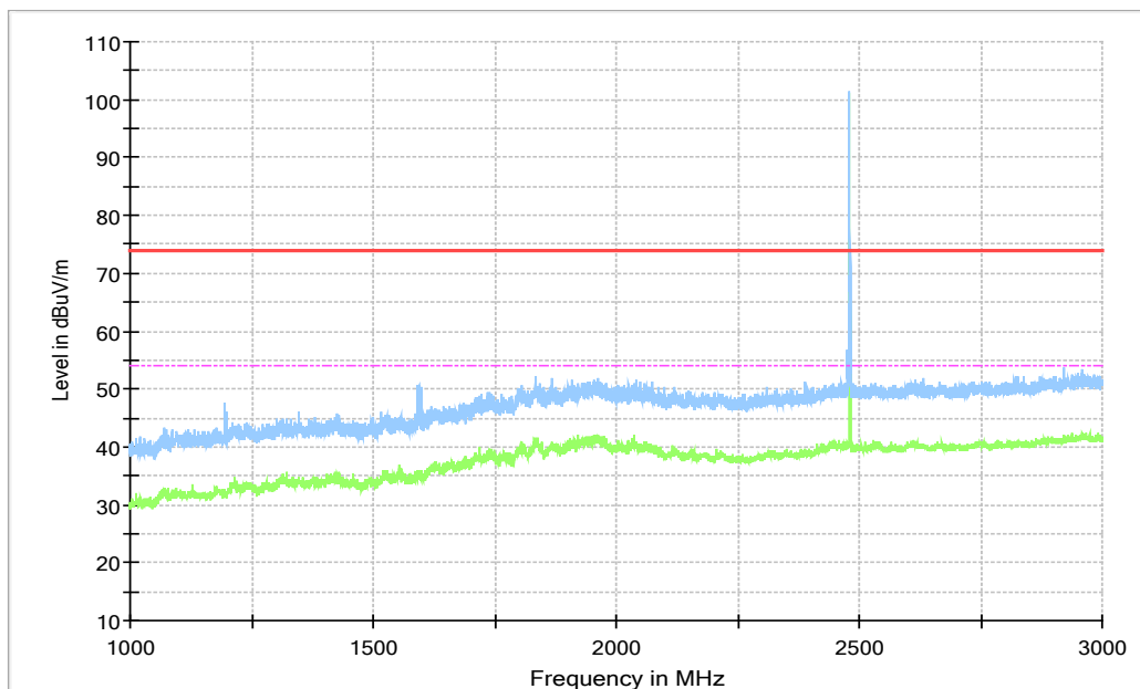
Fig. 5 Radiated Spurious Emission (GFSK, Ch78, 1 GHz ~3 GHz)
