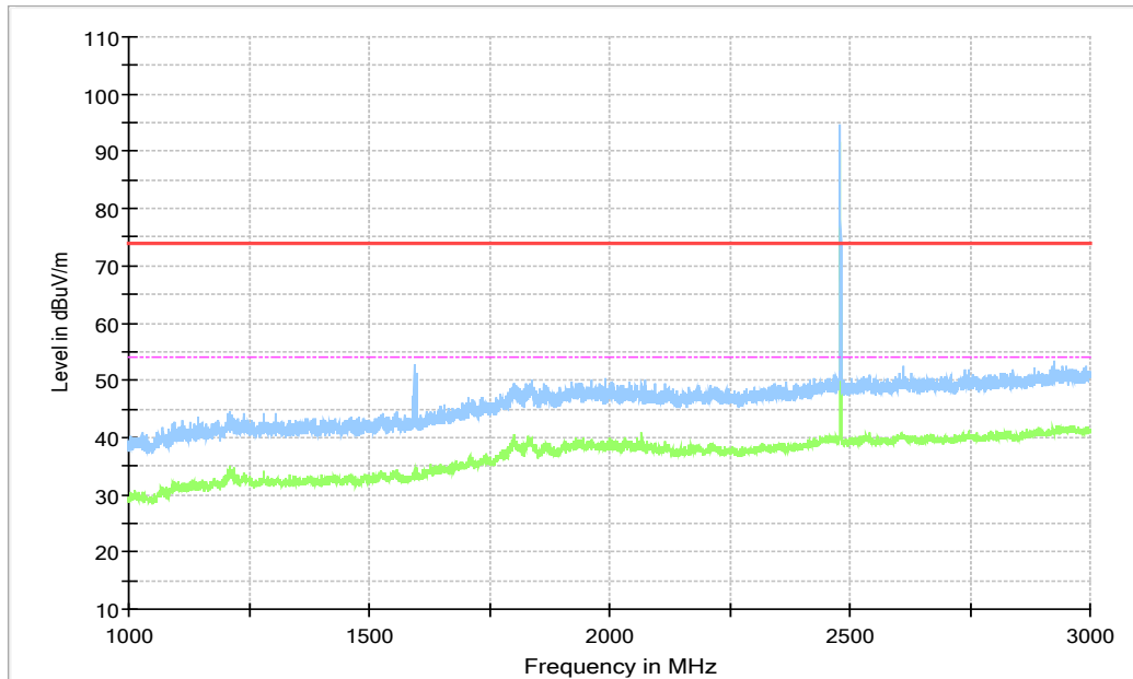
Fig. 13 Radiated Spurious Emission ( \pi/4 DQPSK, Ch78, 1 GHz ~3 GHz)
