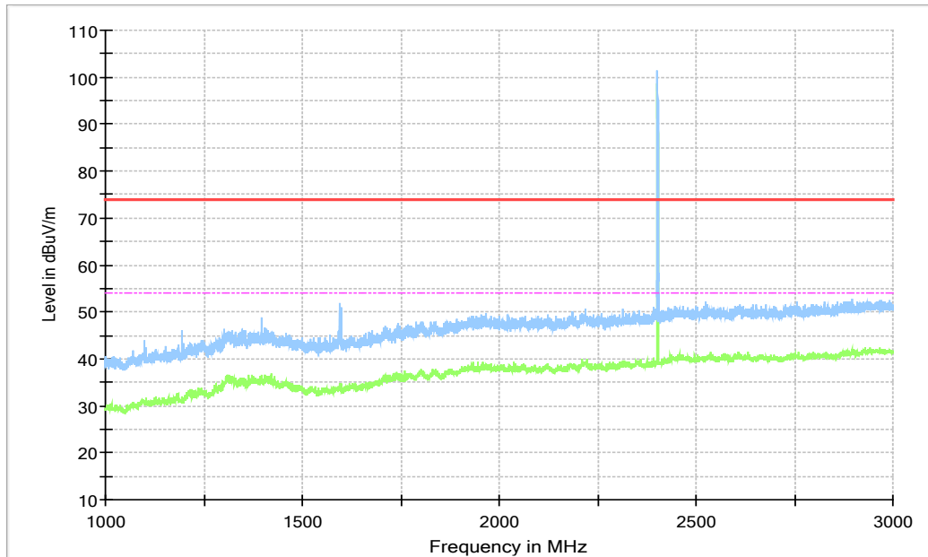
Fig. 9 Radiated Spurious Emission ( \pi/4 DQPSK, Ch0, 1 GHz ~3 GHz)
