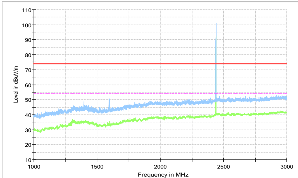
Fig. 11 Radiated Spurious Emission ( \pi/4 DQPSK, Ch39, 1 GHz ~3 GHz)
