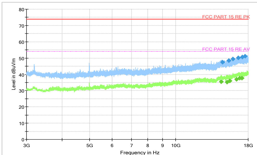
Fig. 22 Radiated Spurious Emission (8DPSK, Ch78, 3 GHz ~18 GHz)
