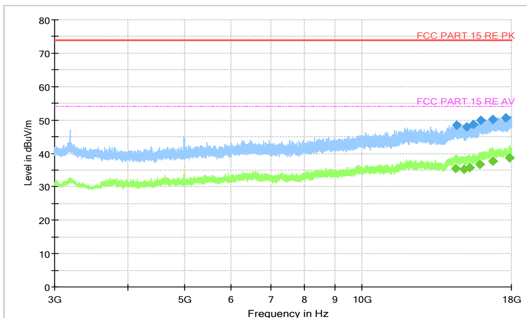
Fig. 20 Radiated Spurious Emission (8DPSK, Ch39, 3 GHz ~18 GHz)
