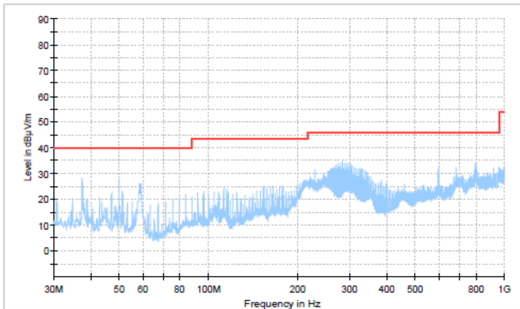
Fig. 26 Radiated Spurious Emission (All Channels, 30 MHz ~1 GHz)
