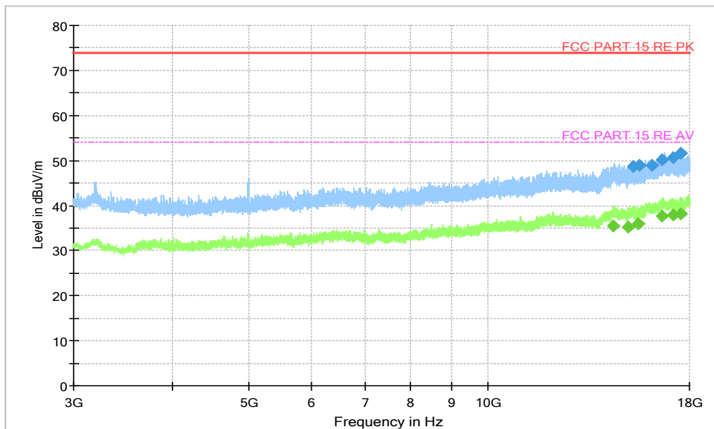
Fig. 12 Radiated Spurious Emission ( \pi/4 DQPSK, Ch39, 3 GHz ~18 GHz)
