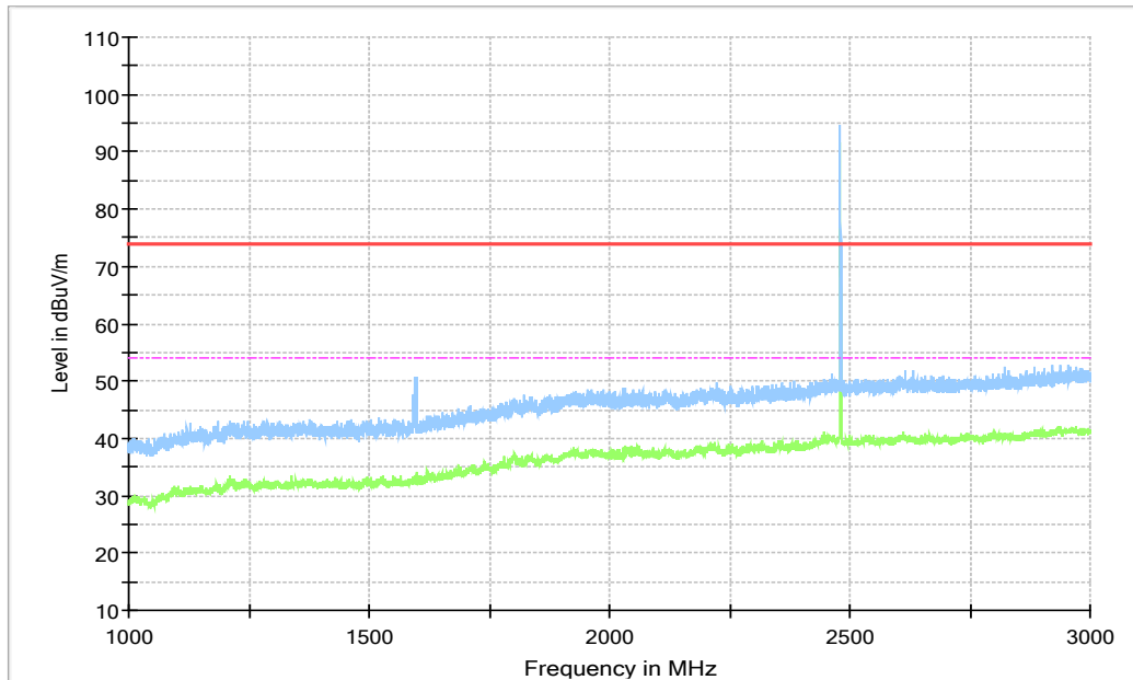
Fig. 21 Radiated Spurious Emission (8DPSK, Ch78, 1 GHz ~3 GHz)
