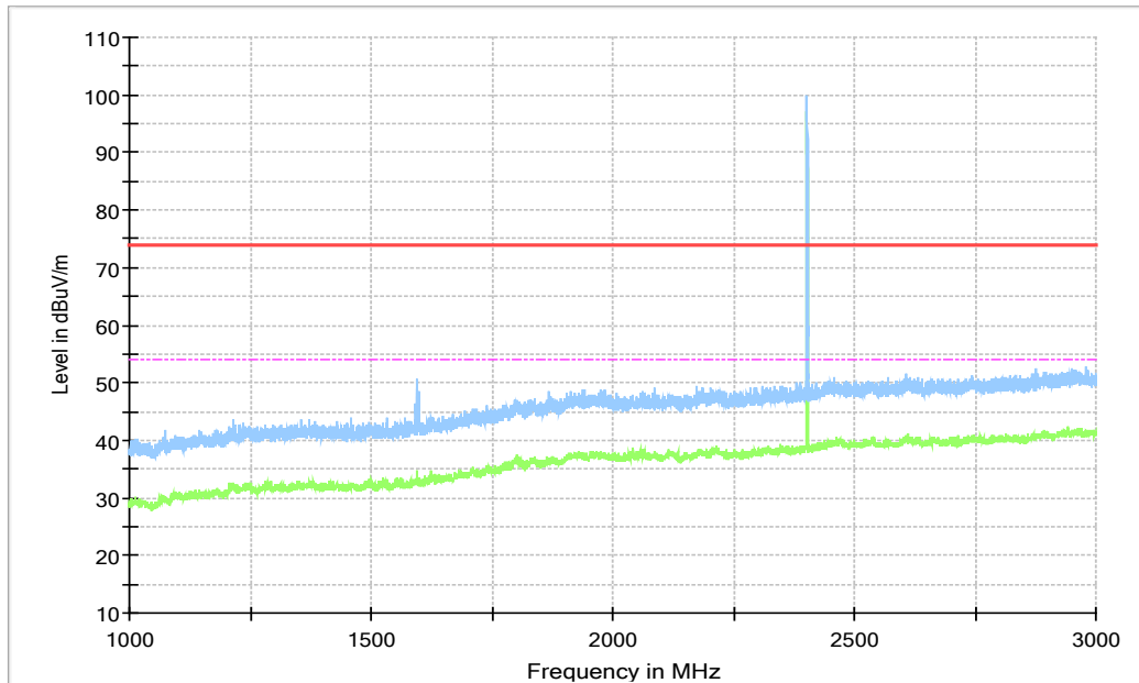
Fig. 17 Radiated Spurious Emission (8DPSK, Ch0, 1 GHz ~3 GHz)
