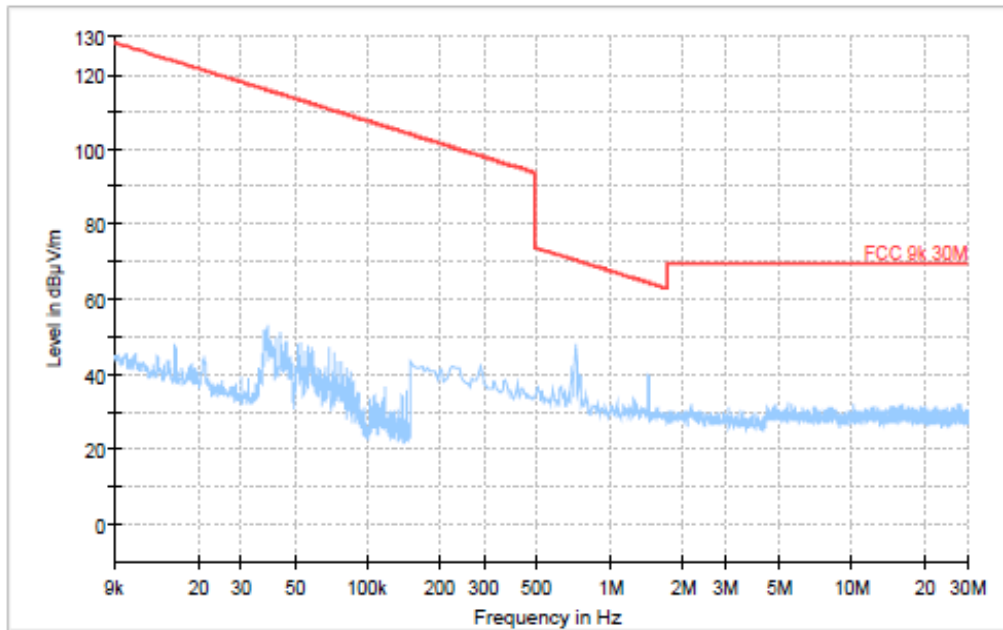
Fig. 25 Radiated Spurious Emission (All Channels, 9 kHz ~30 MHz)
