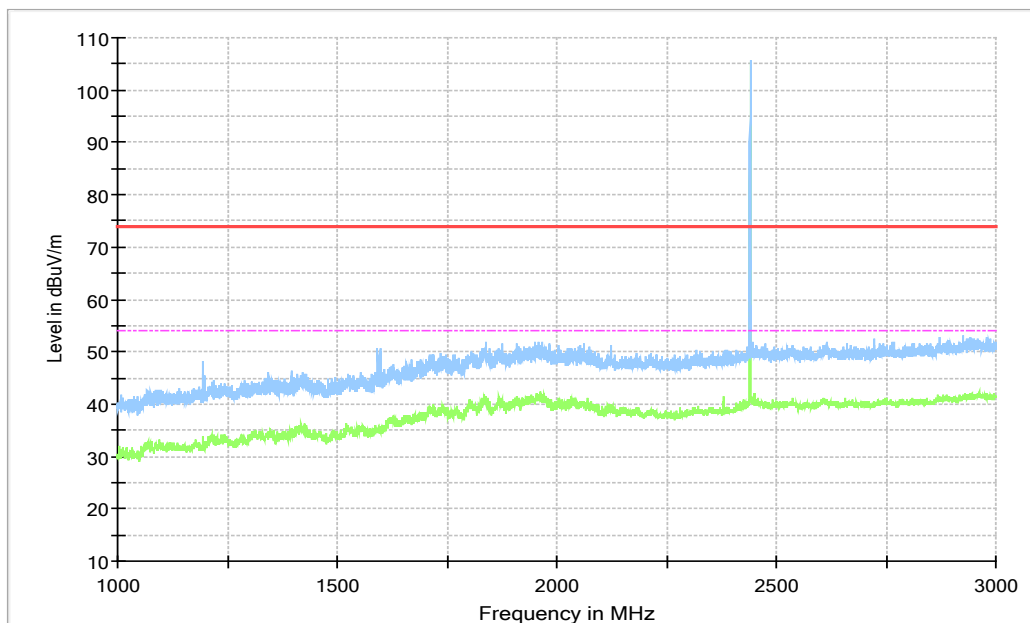
Fig. 3 Radiated Spurious Emission (GFSK, Ch39, 1 GHz ~3 GHz)
