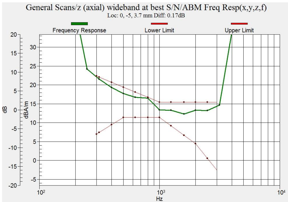
Figure B.14 Frequency Response of LTE-Band 38
