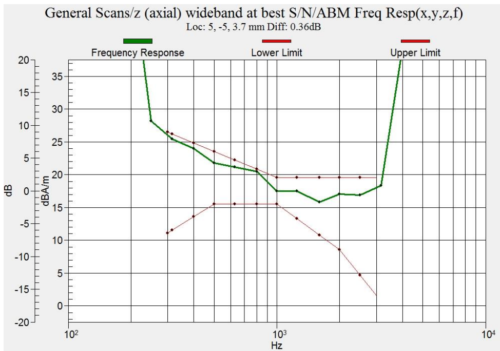
Figure B.29 Frequency Response of WIFI 5.5G (MIMO)
