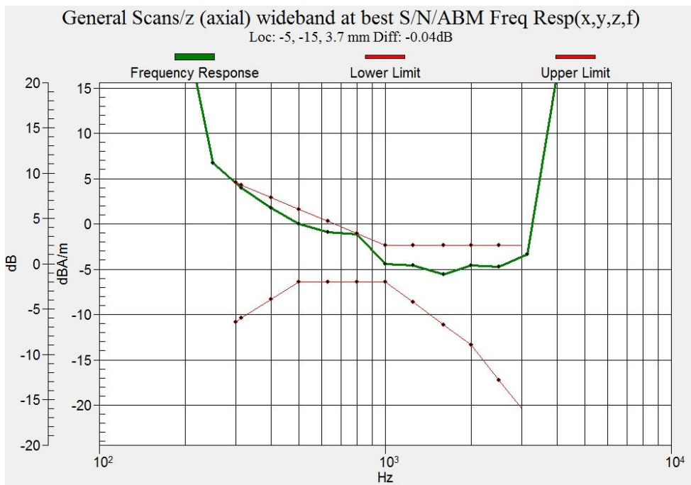
Figure B.24 Frequency Response of WIFI 5.5G (Second antenna)
