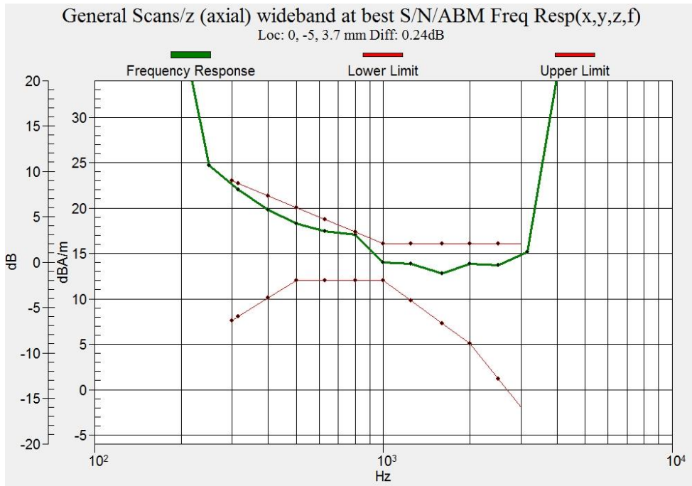
Figure B.13 Frequency Response of LTE-Band 26
