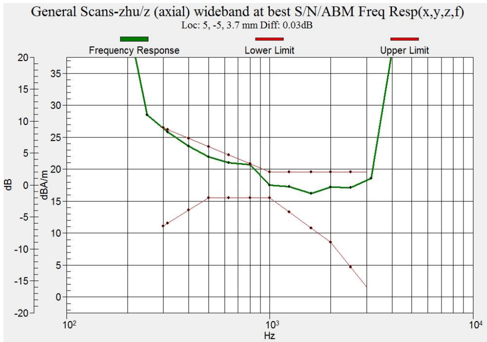
Figure B.16 Frequency Response of WIFI 2.4G (Main antenna)
