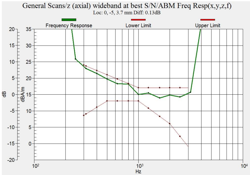
Figure B.27 Frequency Response of WIFI 5.2G (MIMO)
