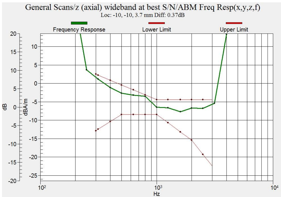
Figure B.23 Frequency Response of WIFI 5.3G (Second antenna)
