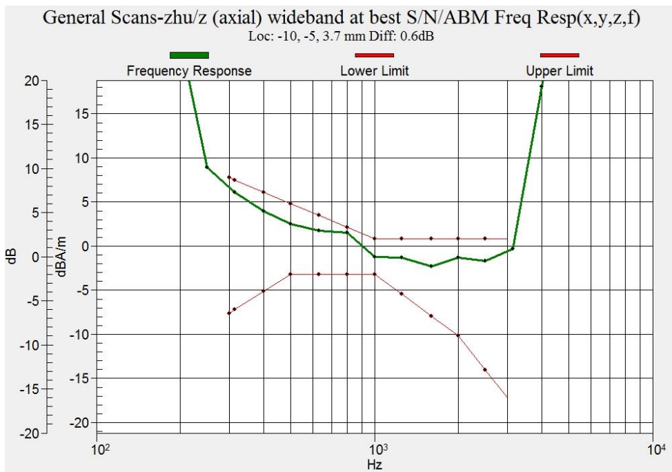
Figure B.30 Frequency Response of WIFI 5.8G (MIMO)
