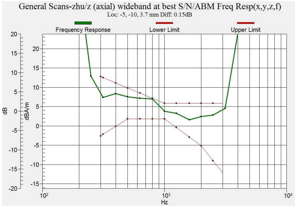
Figure B.18 Frequency Response of WIFI 5.3G (Main antenna)
