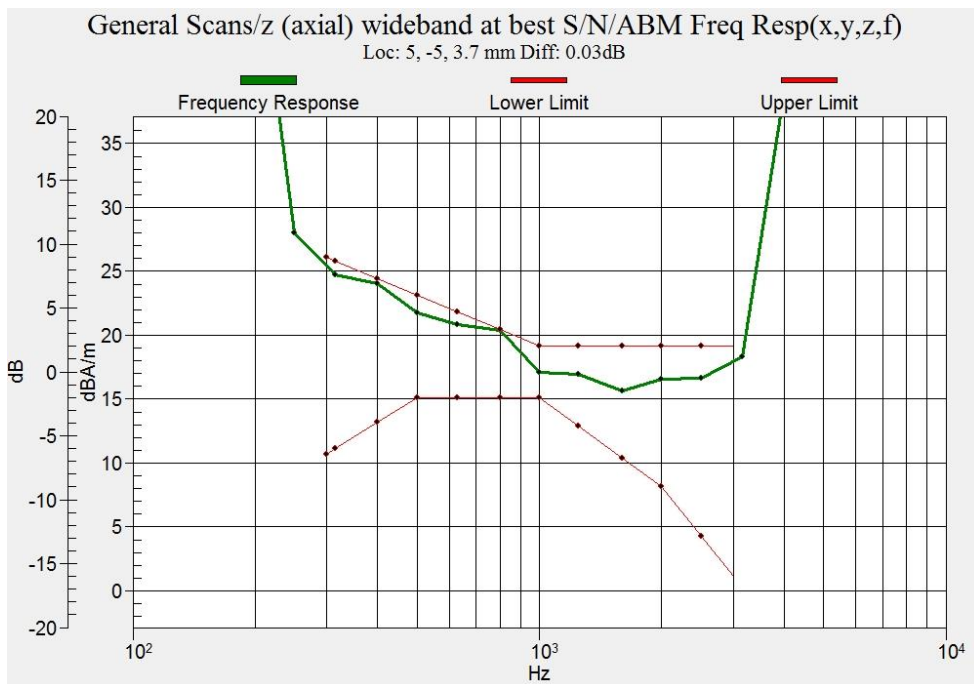
Figure B.28 Frequency Response of WIFI 5.3G (MIMO)
