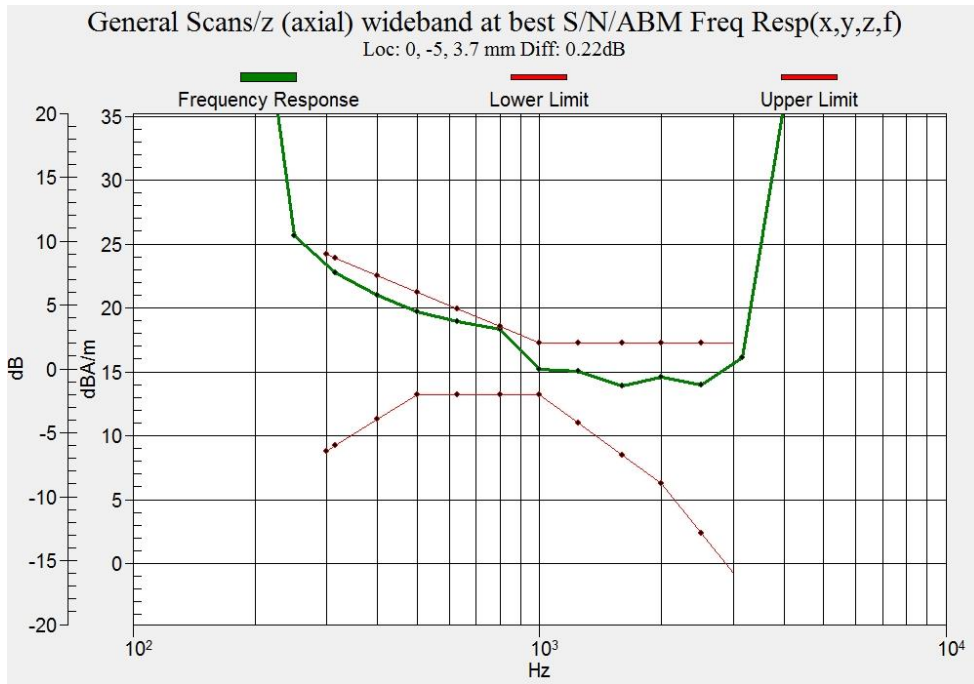
Figure B.21 Frequency Response of WIFI 2.4G (Second antenna)
